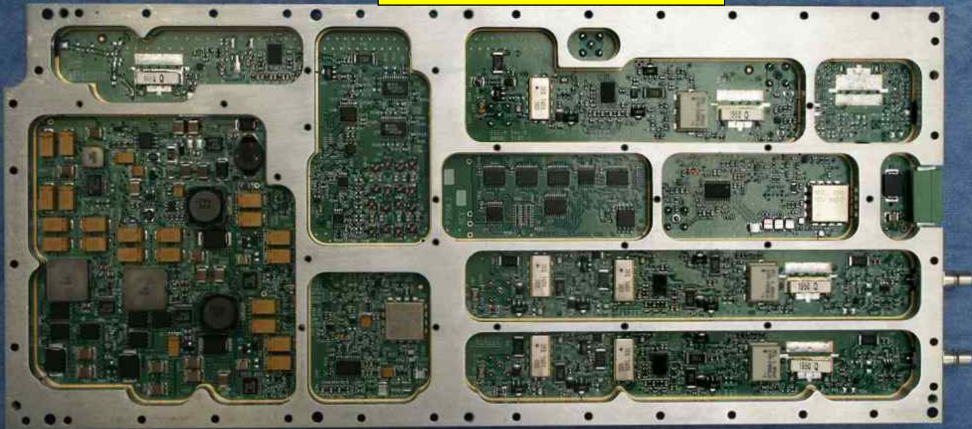
DIGITAL CONTROL MODULE RF BOARD UPLINK (TOP)
