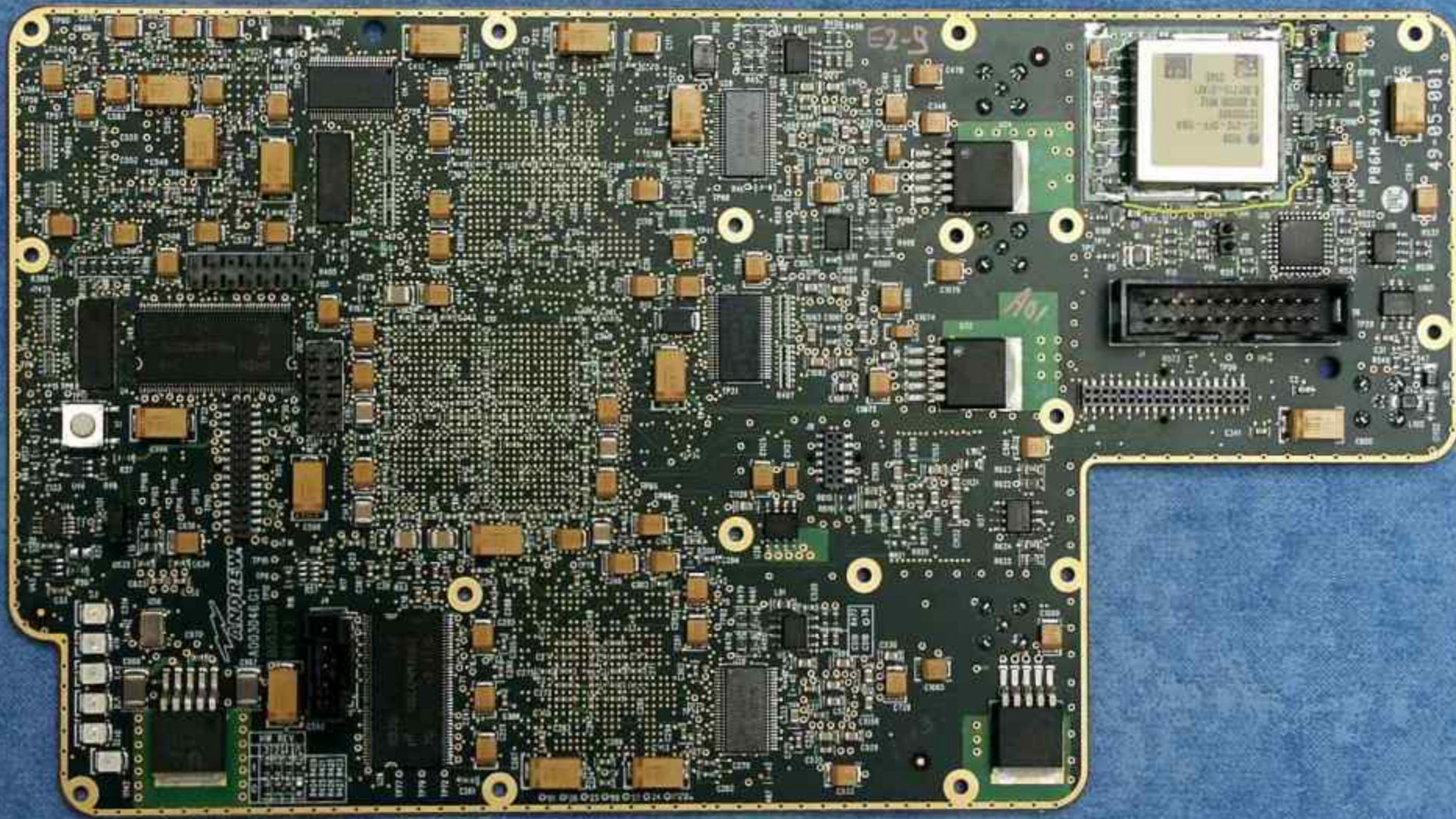
DIGITAL CONTROL MODULE LOGIC BOARD UPLINK (TOP)
