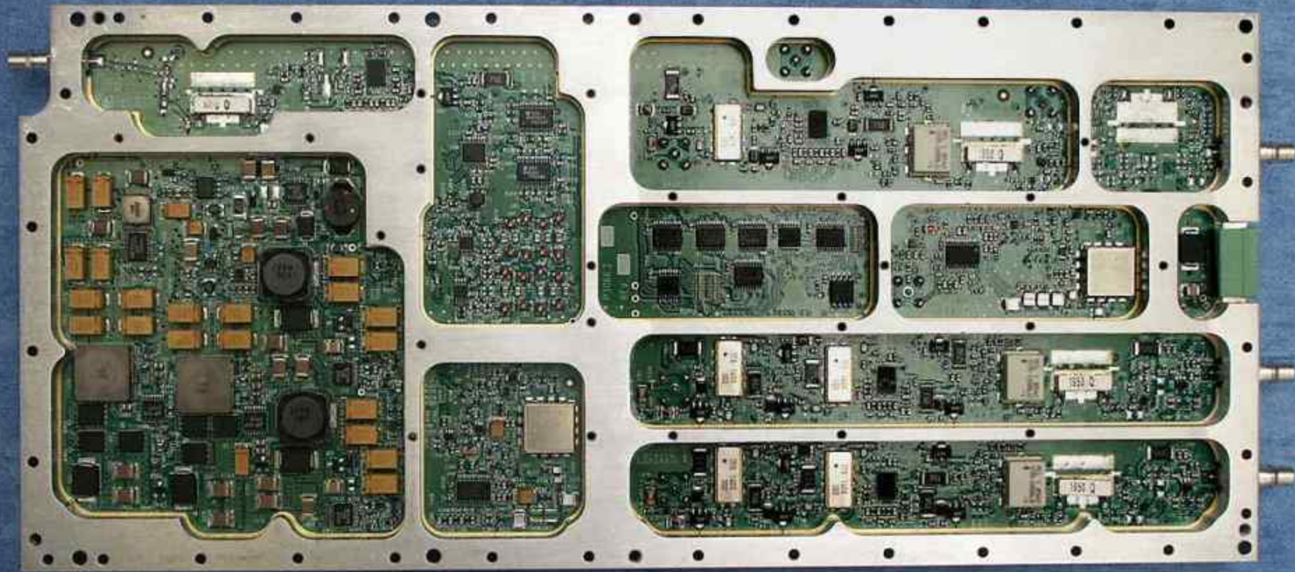
DIGITAL CONTROL MODULE DOWNLINK RF TOP
