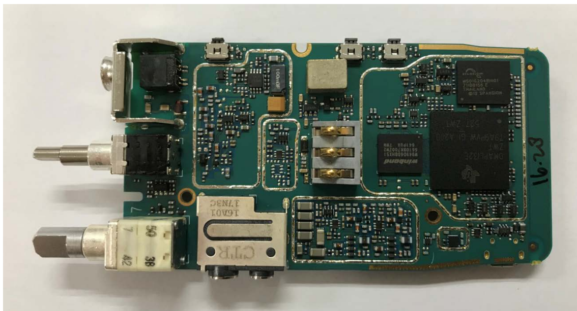
RF board without Shields (Bottom)
