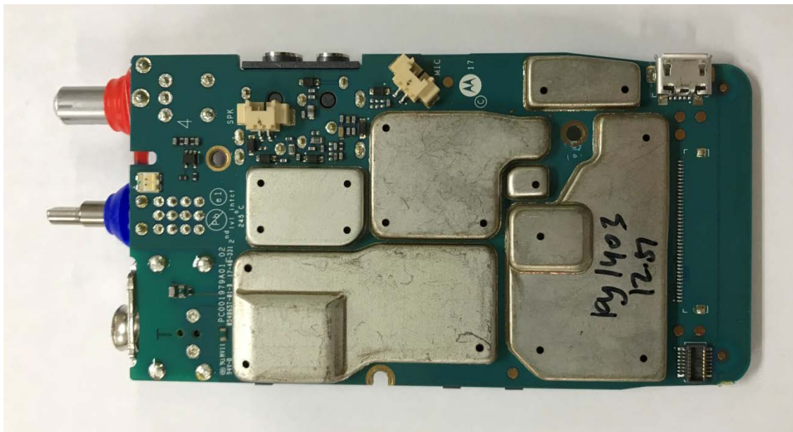
RF board with Shields (Top)
