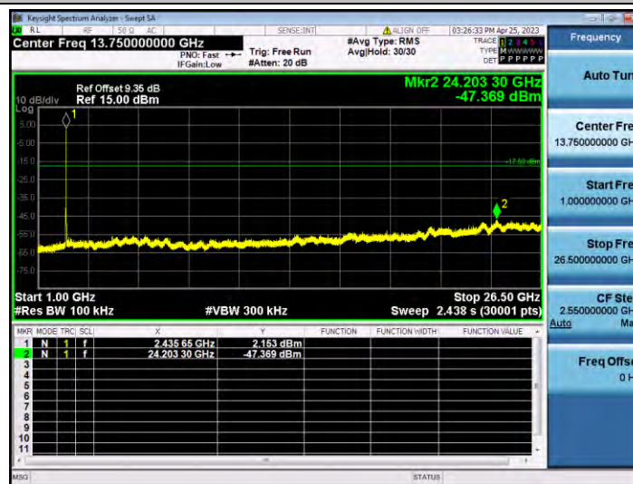
11G_Ant2_2437_1000~26500
