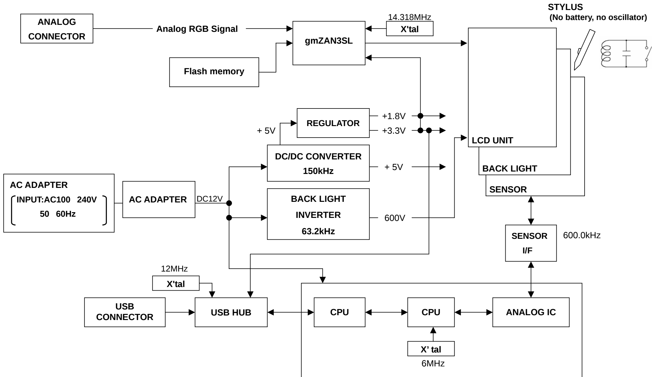
< DTF-720 Block Diagram >
