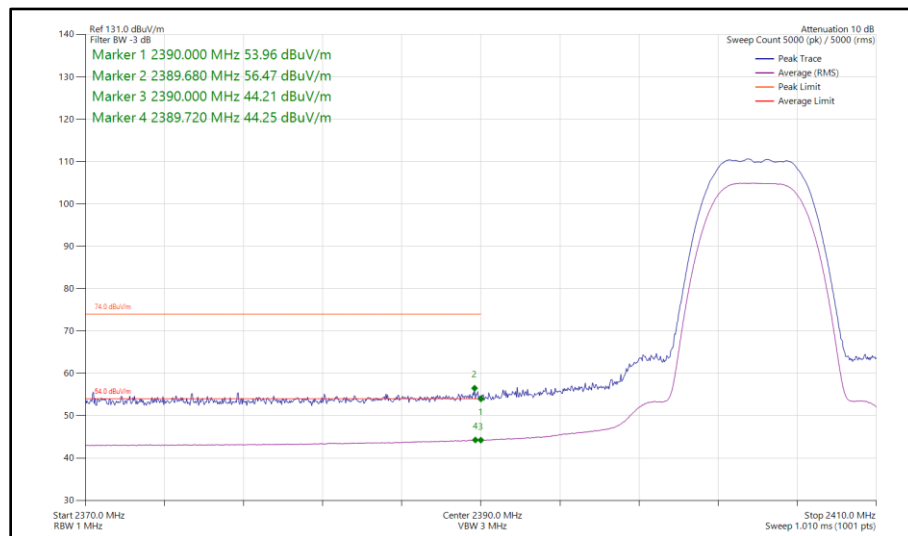
Figure 62 - Bluetooth HDR8, MIMO, Core 0-1 - 2404 MHz Band Edge Frequency 2390 MHz
