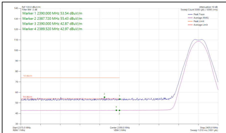
Figure 34 - Bluetooth LE2M, MIMO, Core 0-1 - 2402 MHz Band Edge Frequency 2390 MHz
