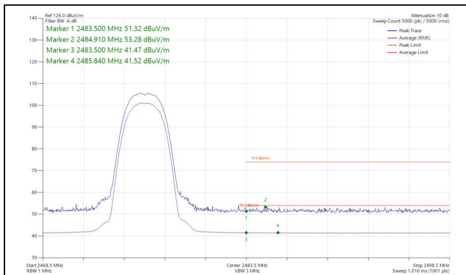
Figure 35 - Bluetooth HDR4, MIMO, Core 0-1 - 2476 MHz Band Edge Frequency 2483.5 MHz
