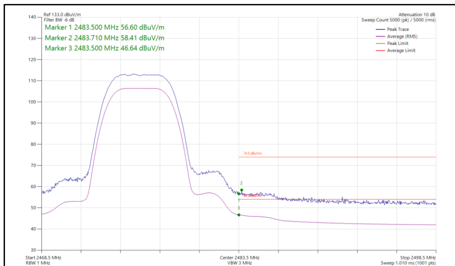
Figure 64 - Bluetooth HDR8, MIMO, Core 0-1 - 2476 MHz Band Edge Frequency 2483.5 MHz
