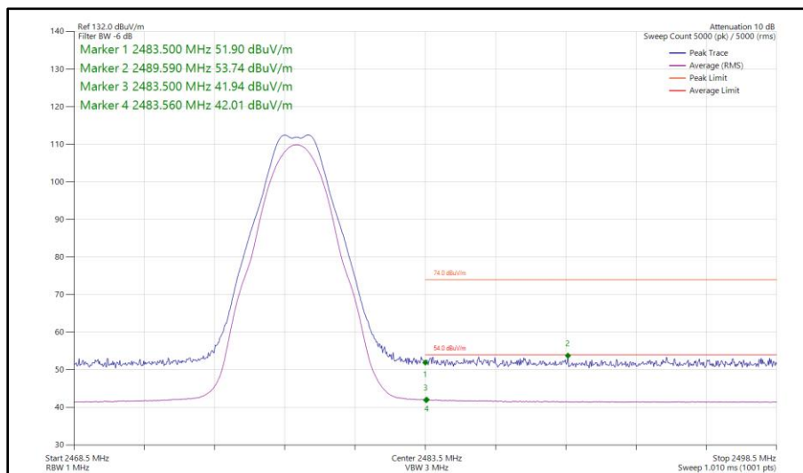
Figure 39 - Bluetooth LE2M, MIMO, Core 0-1 - 2478 MHz Band Edge Frequency 2483.5 MHz
