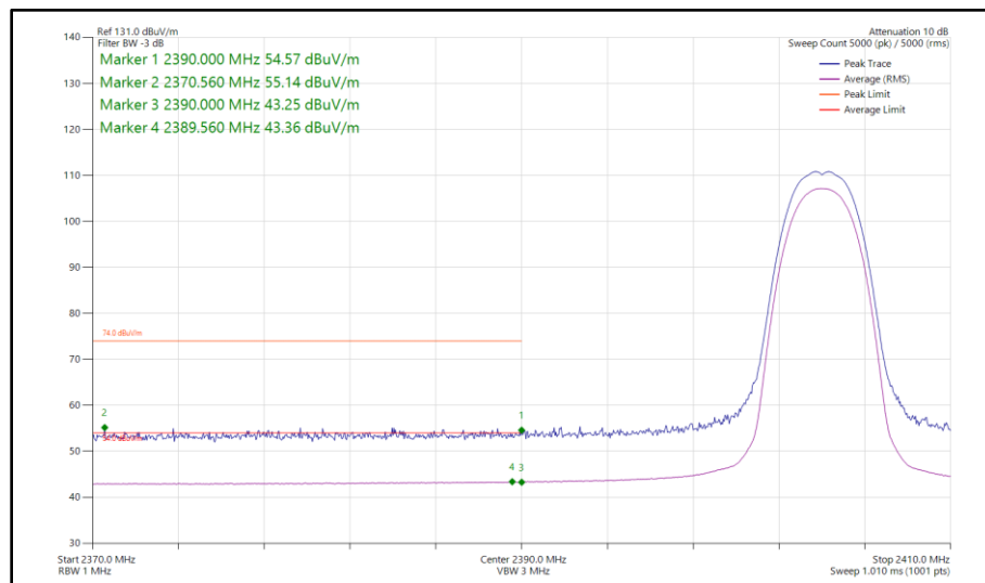
Figure 61 - Bluetooth HDR4, MIMO, Core 0-1 - 2404 MHz Band Edge Frequency 2390 MHz
