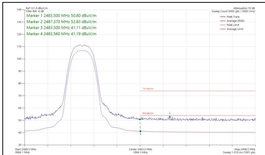
Figure 63 - Bluetooth HDR4, MIMO, Core 0-1 - 2476 MHz Band Edge Frequency 2483.5 MHz
