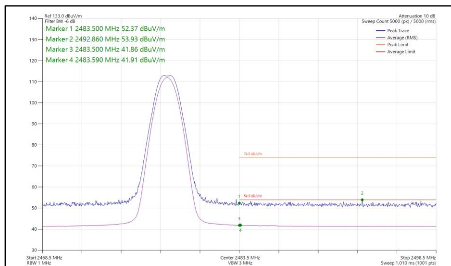
Figure 37 - Bluetooth LE1M, MIMO, Core 0-1 - 2478 MHz Band Edge Frequency 2483.5 MHz
