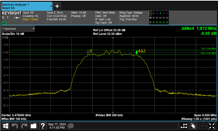
Figure 70 - Core 0 (A) 2476 MHz (CH74) 6 dB Bandwidth
