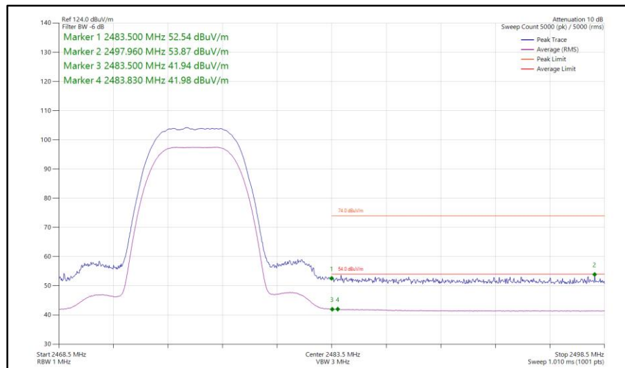
Figure 36 - Bluetooth HDR8, MIMO, Core 0-1 - 2476 MHz Band Edge Frequency 2483.5 MHz
