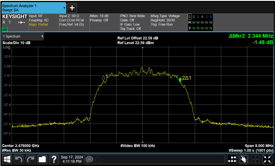
Figure 69 - Core 0 (A) 2476 MHz (CH74) 99% Bandwidth
