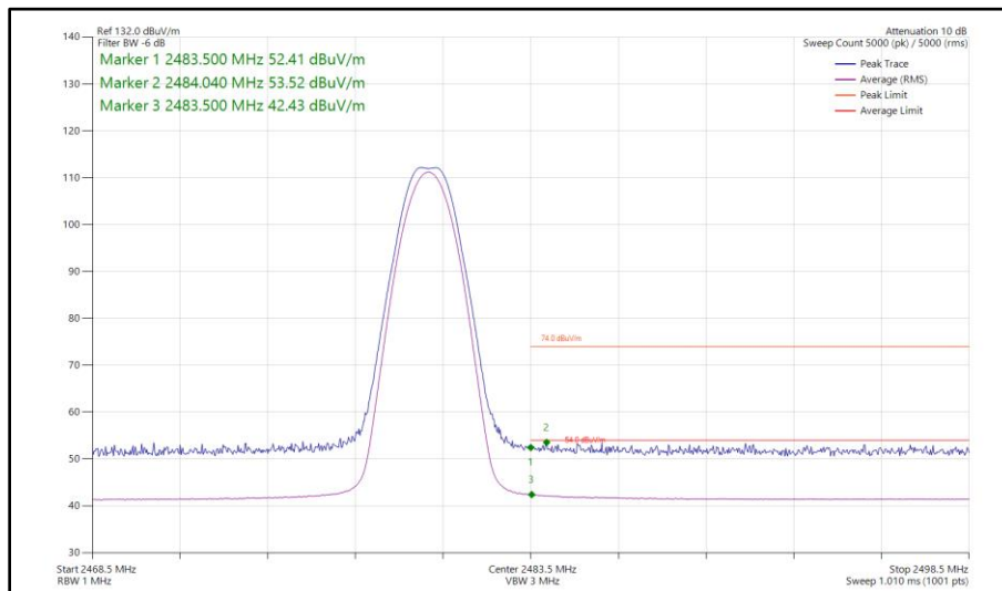
Figure 38 - Bluetooth LE1M, MIMO, Core 0-1 - 2480 MHz Band Edge Frequency 2483.5 MHz
