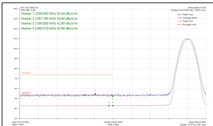
Figure 33 - Bluetooth LE1M, MIMO, Core 0-1 - 2402 MHz Band Edge Frequency 2390 MHz
