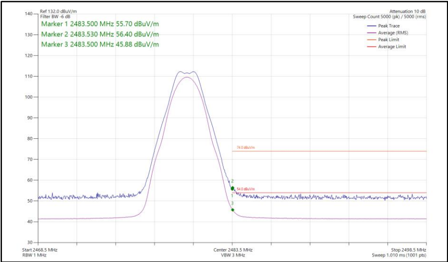
Figure 40 - Bluetooth LE2M, MIMO, Core 0-1 - 2480 MHz Band Edge Frequency 2483.5 MHz
