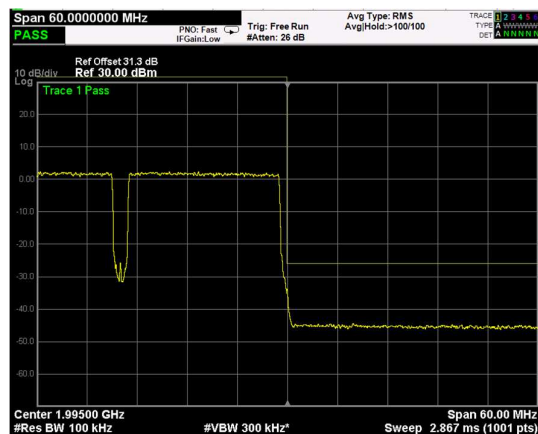
High Band Edge, 2 Carrier, Modulation: QPSK, BW=20MHz
