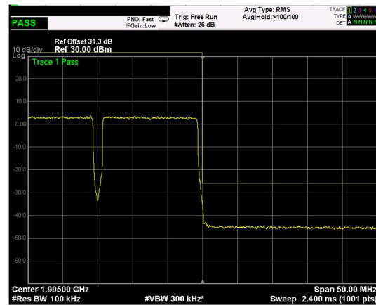
High Band Edge, 2 Carrier, Modulation: 16QAM, BW=15MHz
