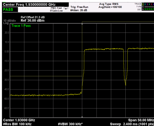
Low Band Edge, 2 Carrier, Modulation: QPSK, BW=15MHz
