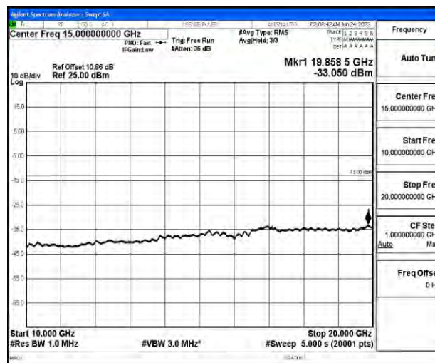
Band4-20MHz-16QAM-20300-1RB#0-Range5:10000~20000MHz
