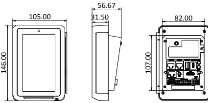
Figure 6: device dimensions (mm)
