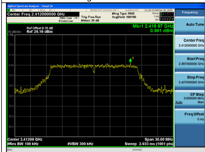
802.11g on Channel 01
