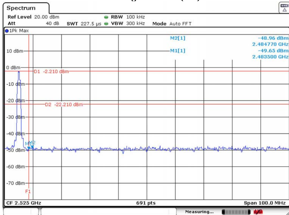
GFSK High Channel (1M)
