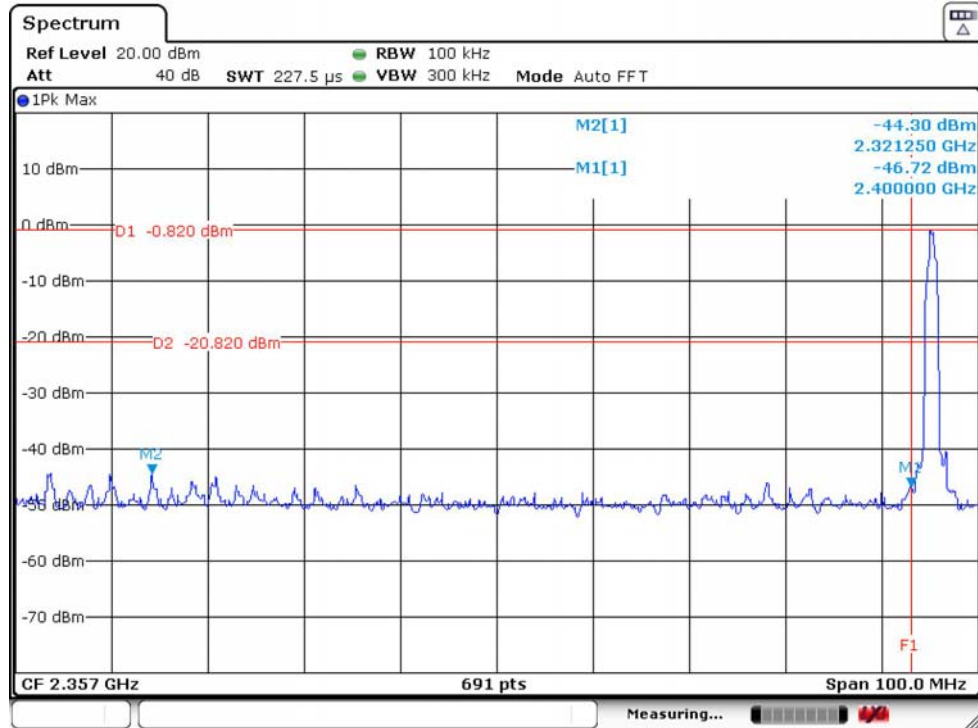
GFSK Low Channel (1M)
