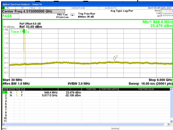
GPRS_850_Higher_Conducted Spurios
