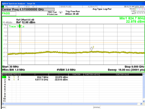
GPRS 850 Lower Conducted Spurios
