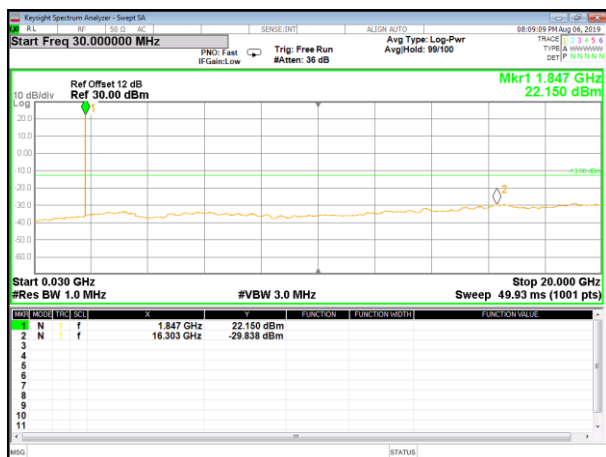
BC1 CDMA Lower Conducted Spurious
