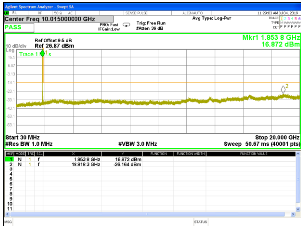
B2_HSDPA_Lower_Conducted_Spurious
