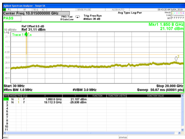
GPRS_1900_Lower_Conducted_Spurious
