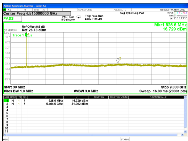
B5_HSUPA Lower Conducted Spurious
