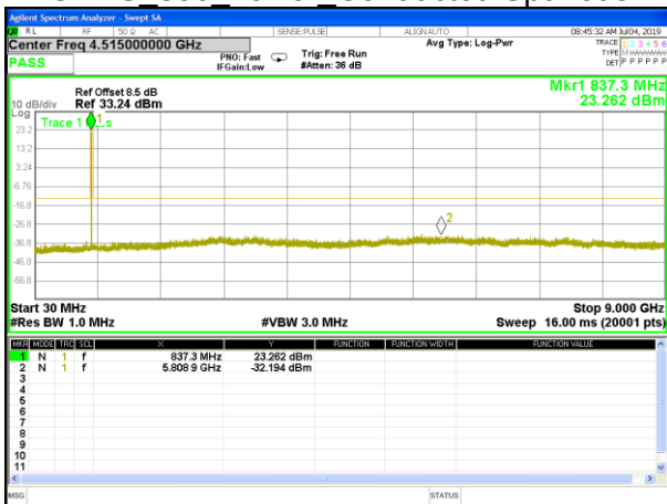
GPRS 850 Middle Conducted Spurios
