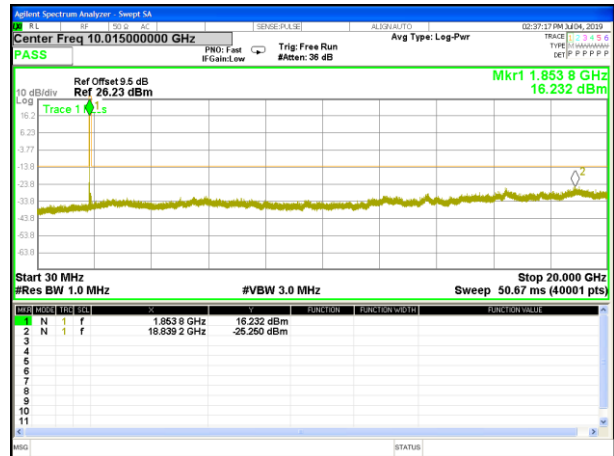
B2_HSUPA_Lower_Conducted_Spurious
