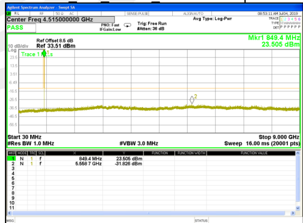
EGPRS_850_Higher_Conducted Spurios
