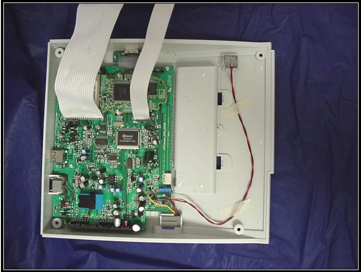
PHOTOGRAPH 27: INSIDE BOTTOM CASE WITH PCB'S ATTACHED
