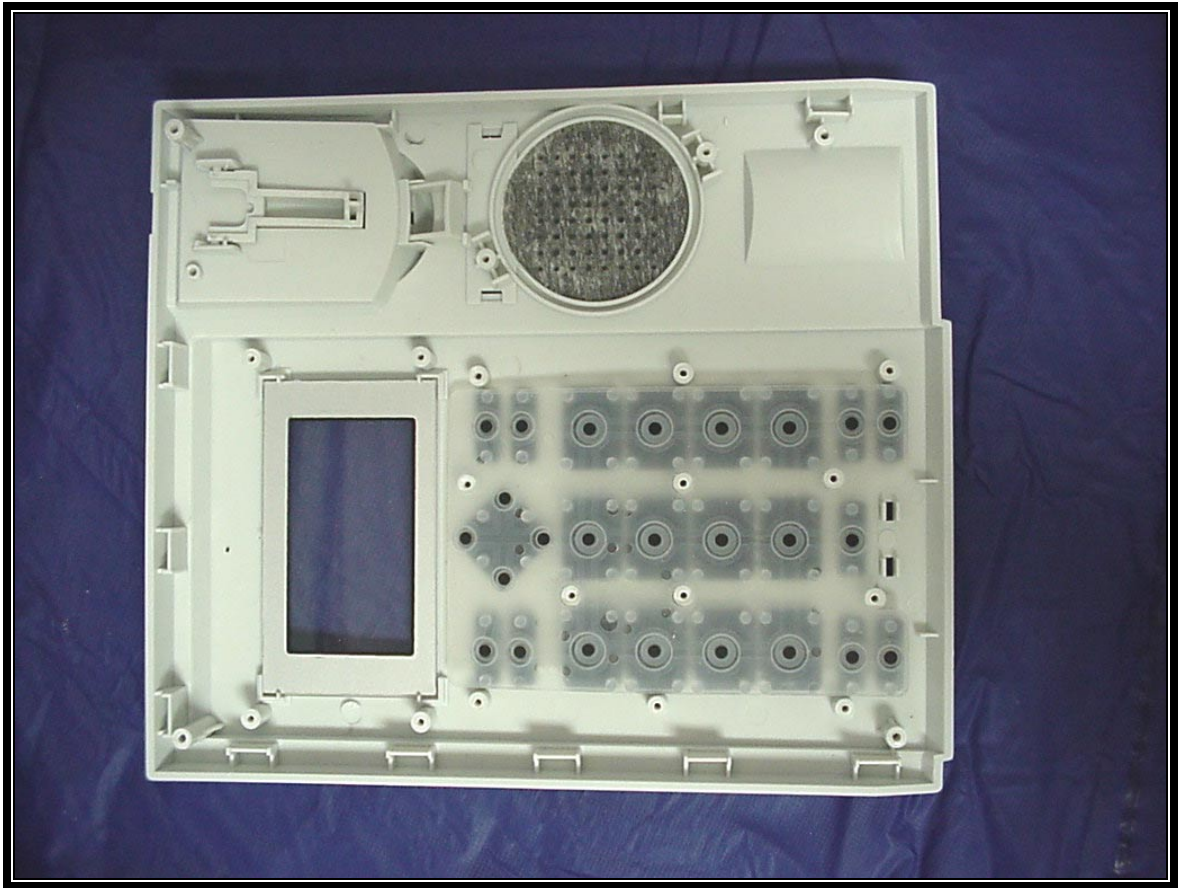
PHOTOGRAPH 25: INSIDE TOP COVER
