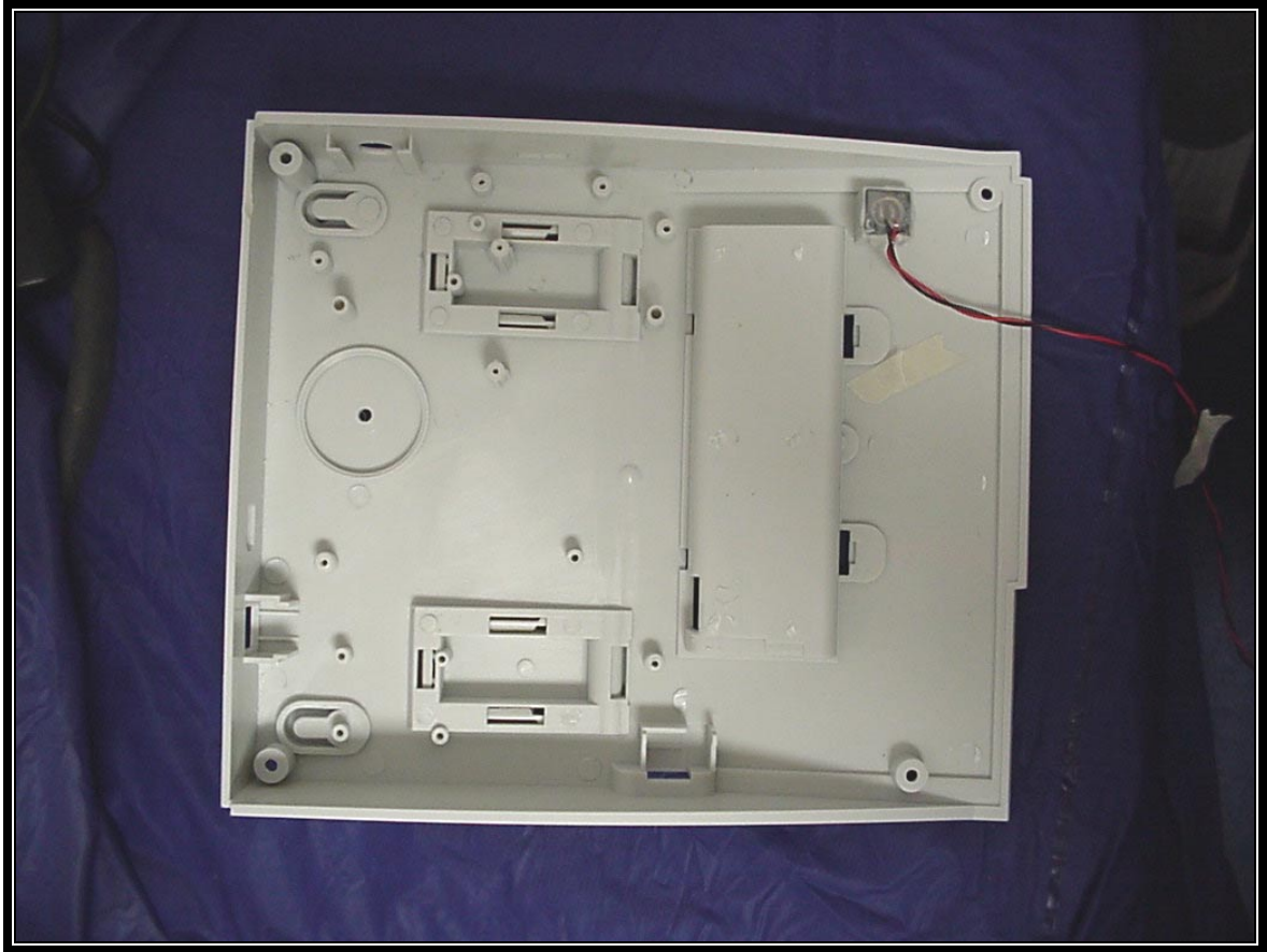
PHOTOGRAPH 26: INSIDE BOTTOM CASE
