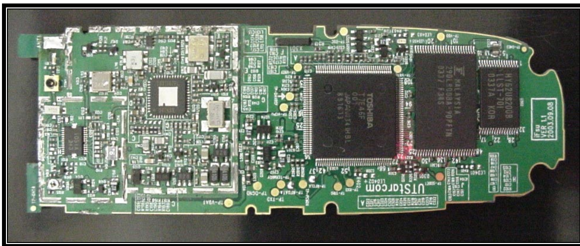
PHOTOGRAPH 30: TOP OF RF PCB WITHOUT SHIELDS
