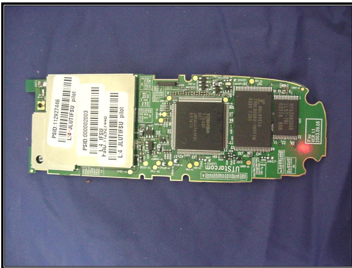
PHOTOGRAPH 29: TOP OF RF PCB WITH SHIELDS
