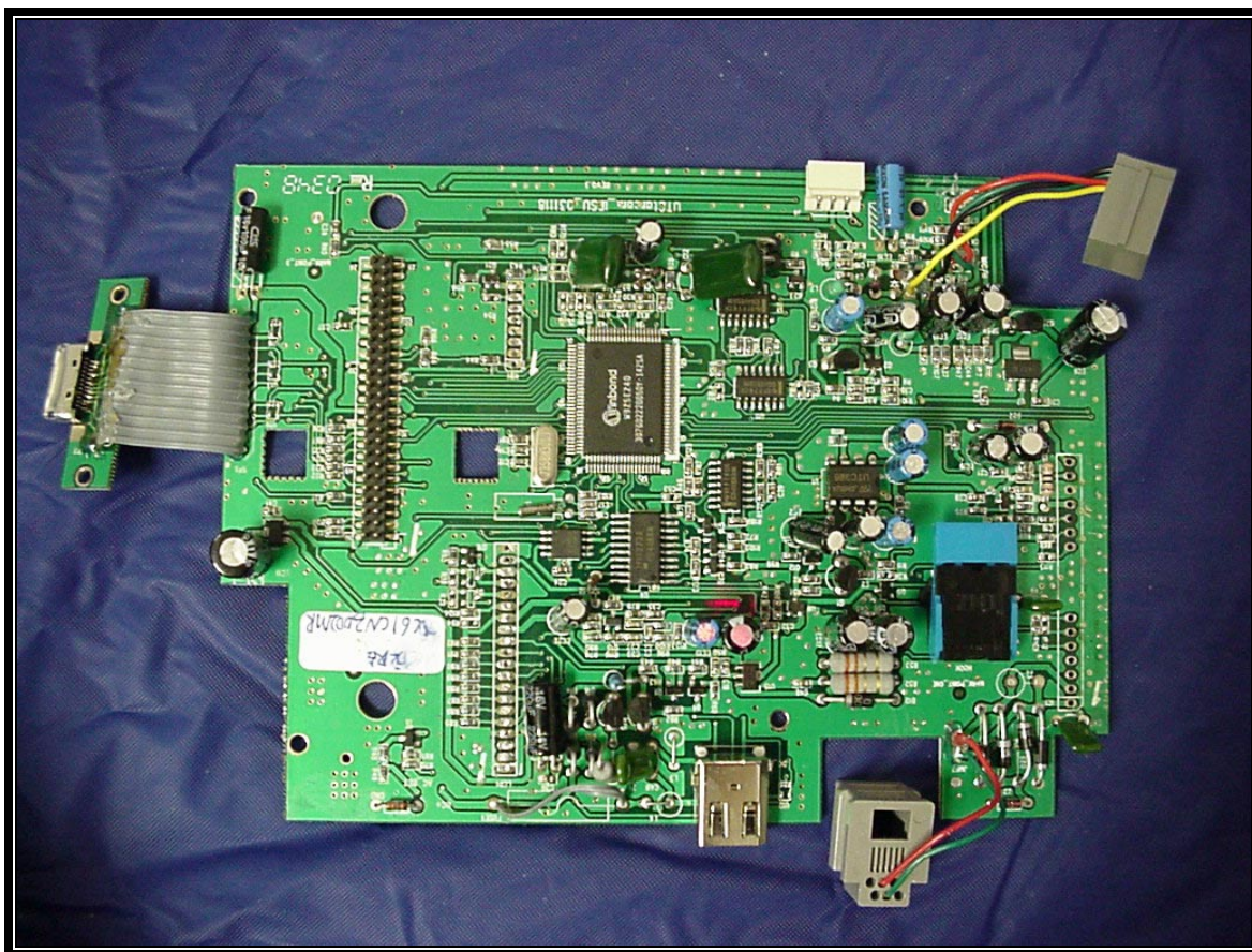
PHOTOGRAPH 34: TOP OF MAIN PCB
