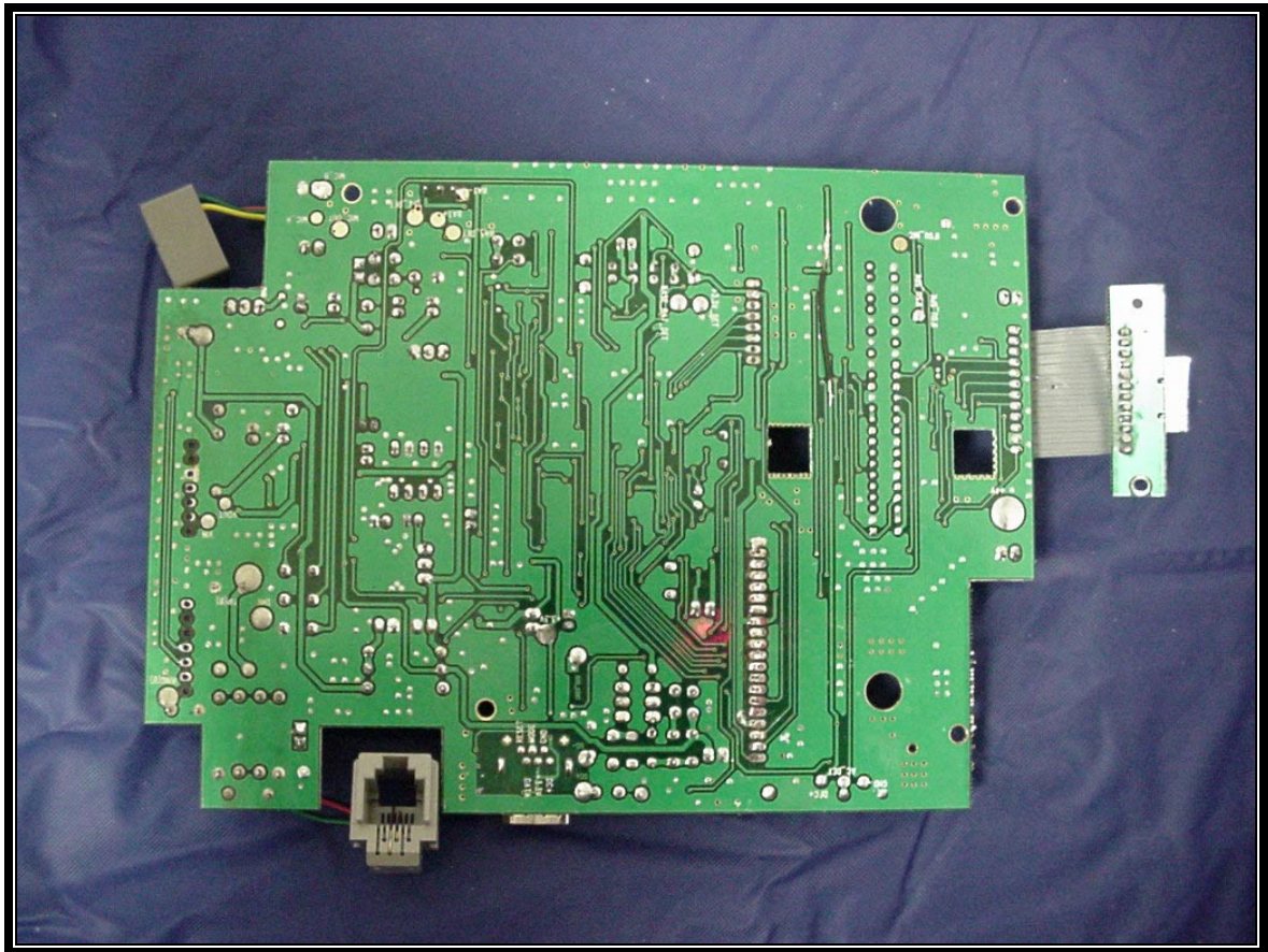
PHOTOGRAPH 35: BOTTOM OF MAIN PCB
