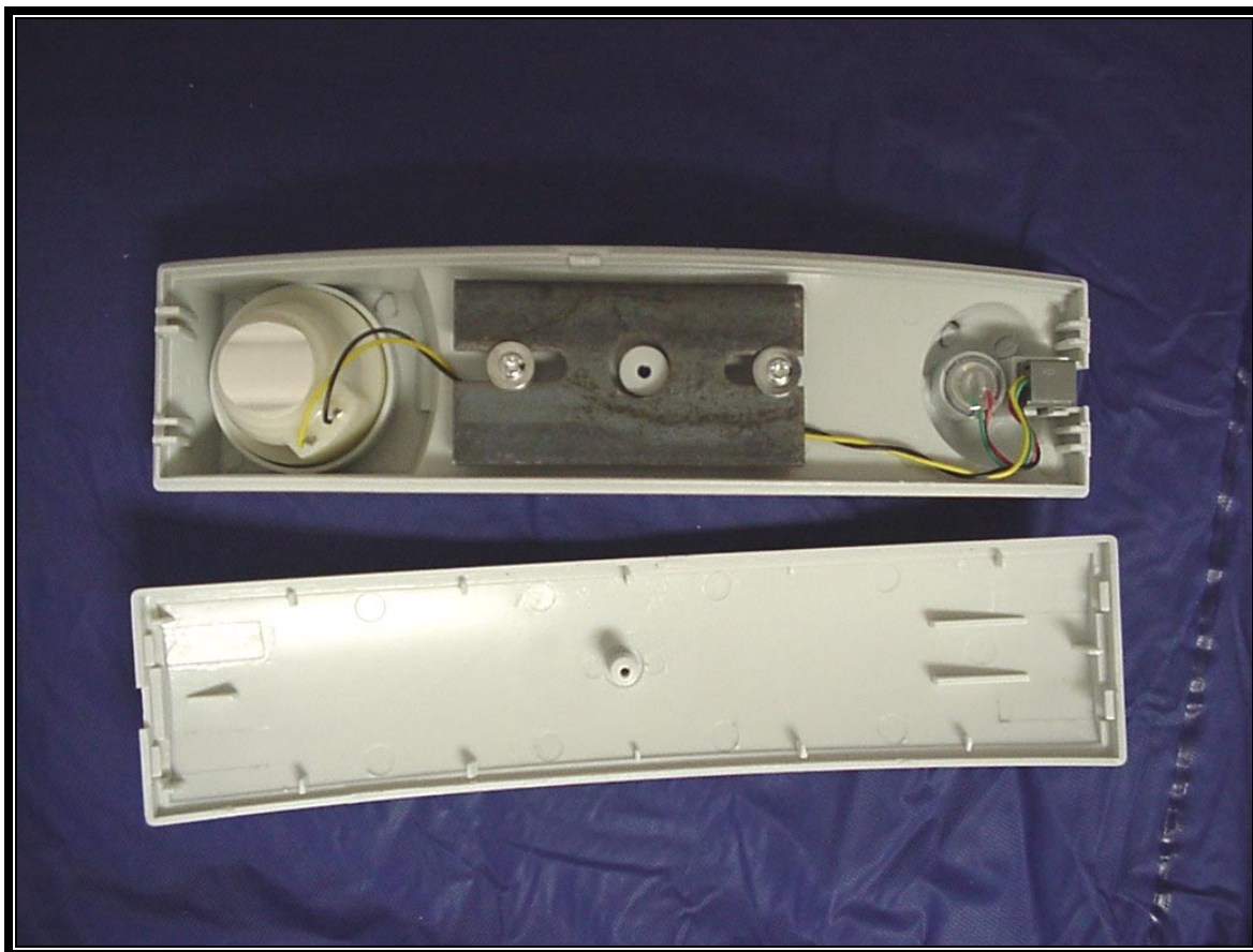
PHOTOGRAPH 24: INSIDE HANDSET
