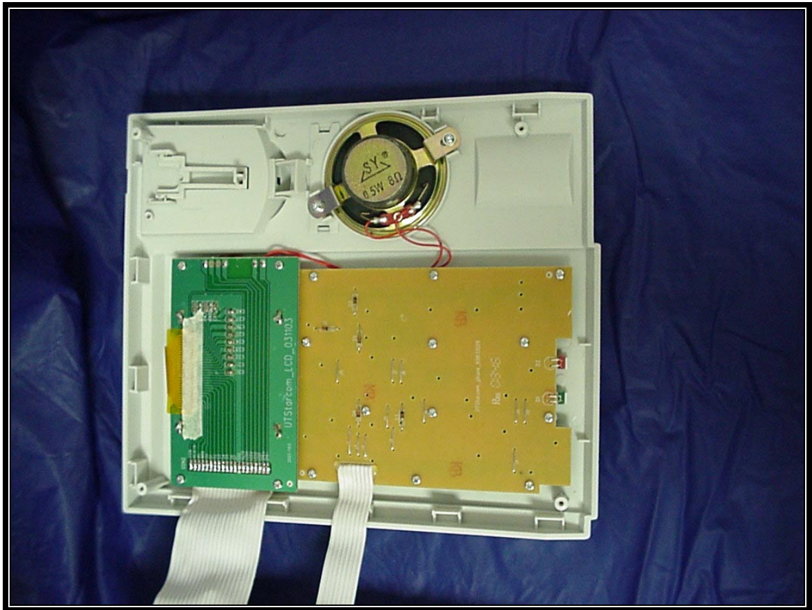
PHOTOGRAPH 28: INSIDE TOP CASE WITH PCB'S ATTACHED
