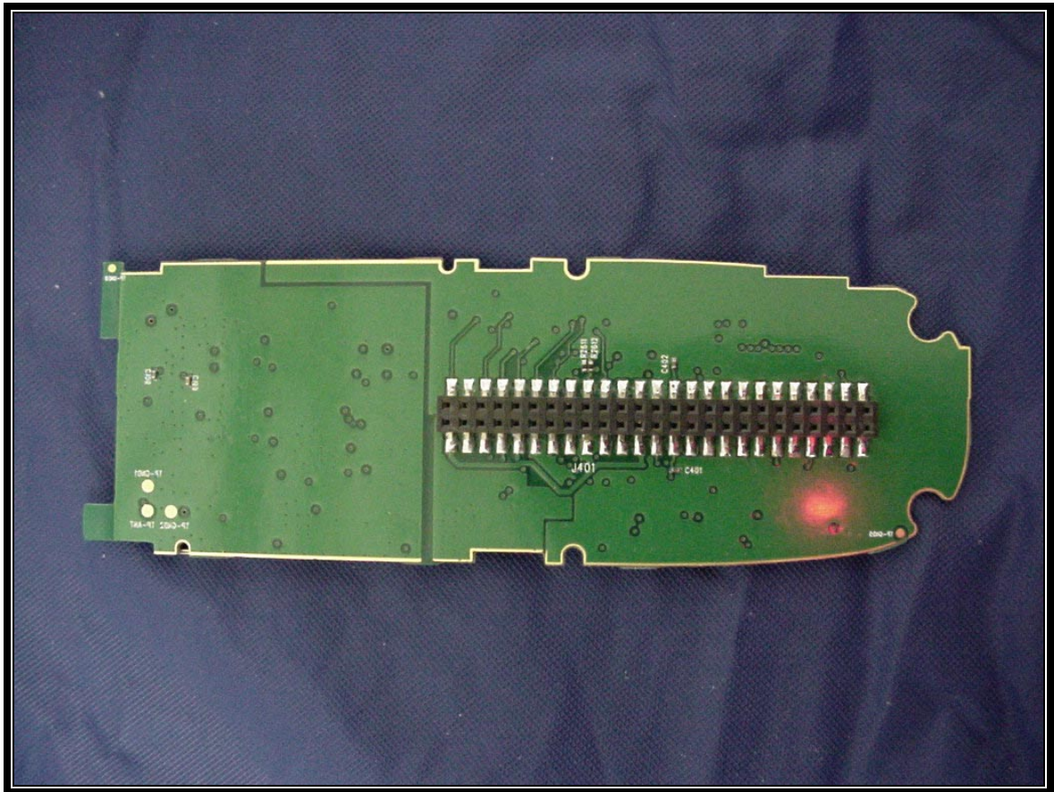
PHOTOGRAPH 31: BOTTOM OF RF PCB
