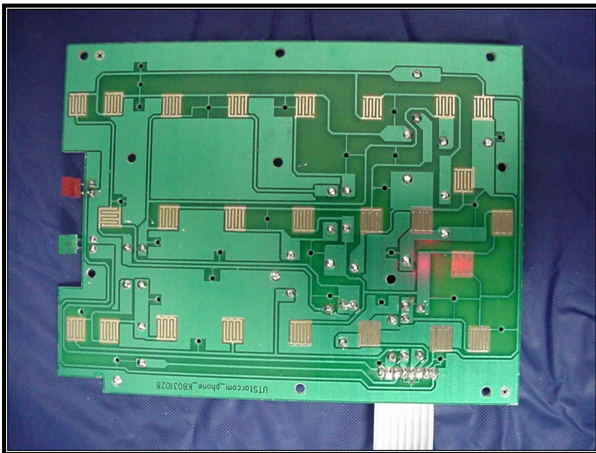
PHOTOGRAPH 38: TOP OF KEYPAD PCB
