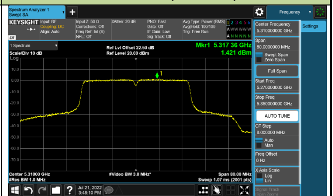
Channel 62 (5310MHz)
