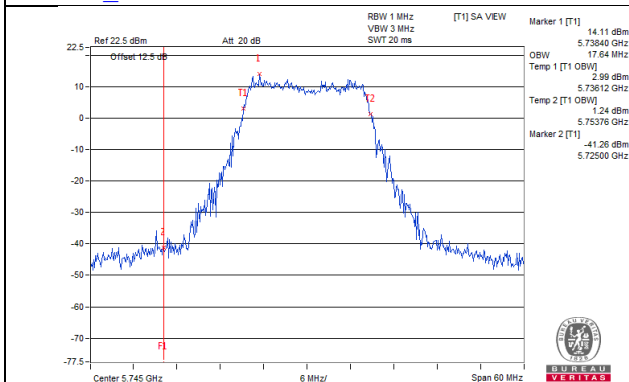
802.11a_Chain 6 / CH149
