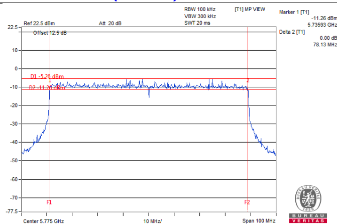
802.11ax (HE80+80) / Chain 0: CH155
