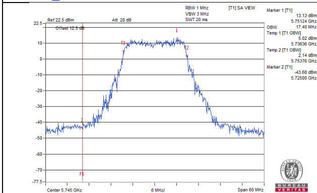
802.11a_Chain 4 / CH149
