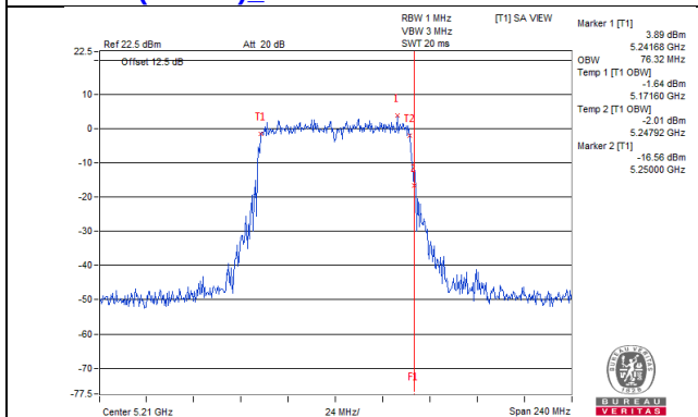
802.11ac (VHT80) Chain 6 / CH42
