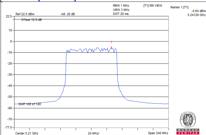
802.11ax (HE80+80) / Chain 7: CH42
