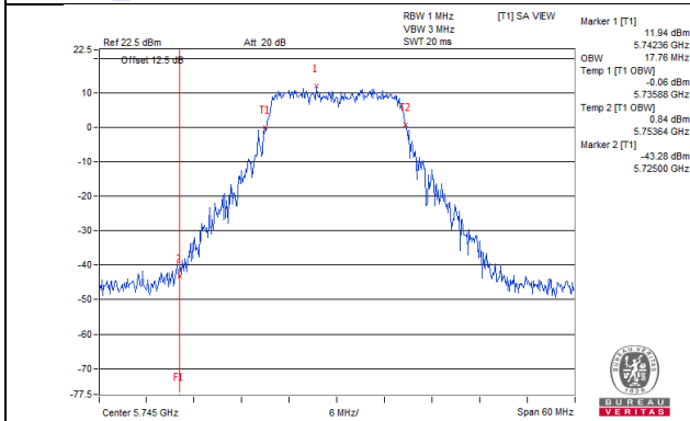
802.11a_Chain 2 / CH149
