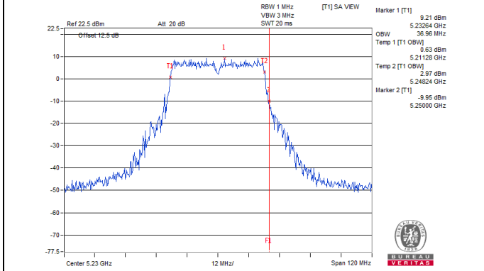
802.11ac (VHT40) Chain 2 / CH46
