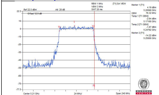
802.11ac (VHT80) Chain 4 / CH42
