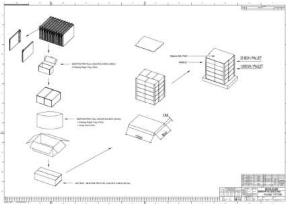
Figure 13. 8.2" Packing-Diagram (1,200 X 800)
