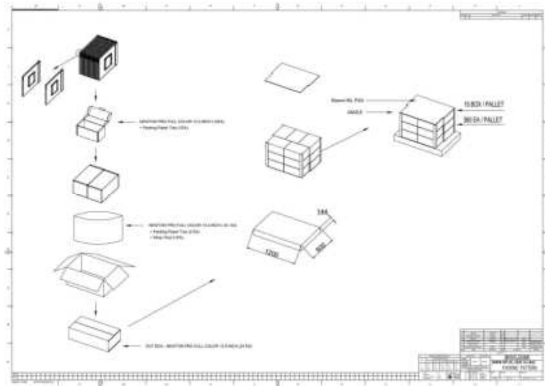
Figure 15. 13.3" Packing-Diagram (1,200 X 800)
