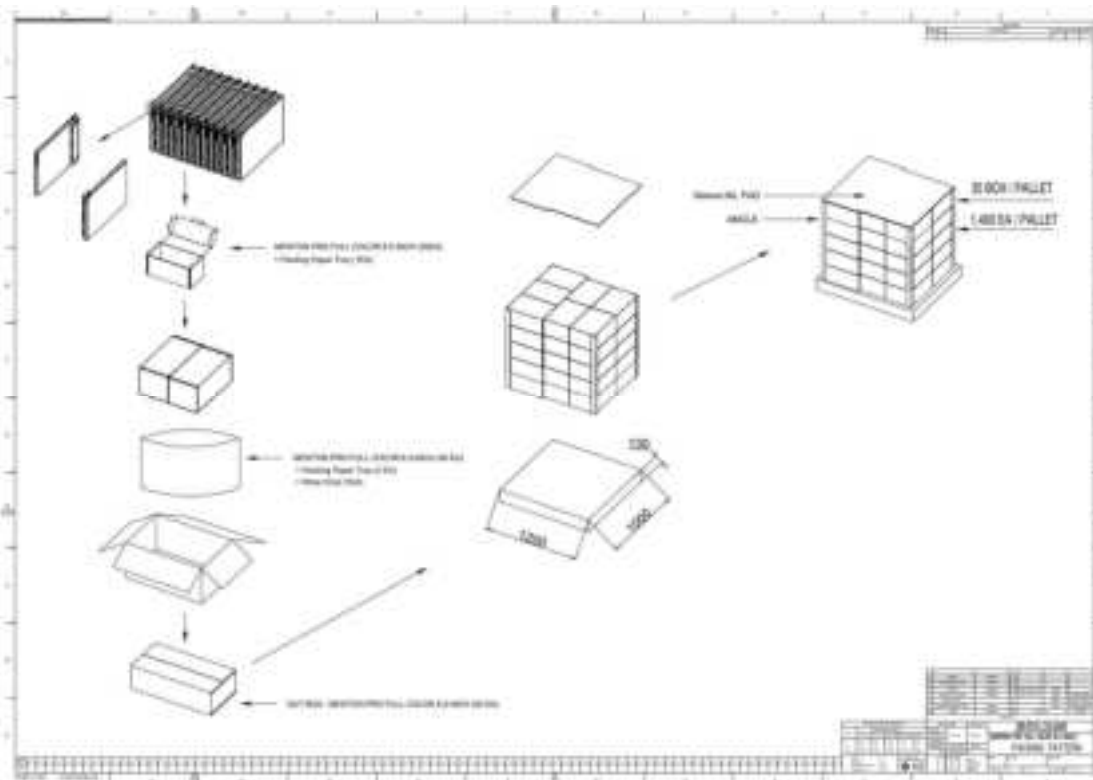
Figure 14. 8.2" Packing-Diagram (1,200 X 1,000)
