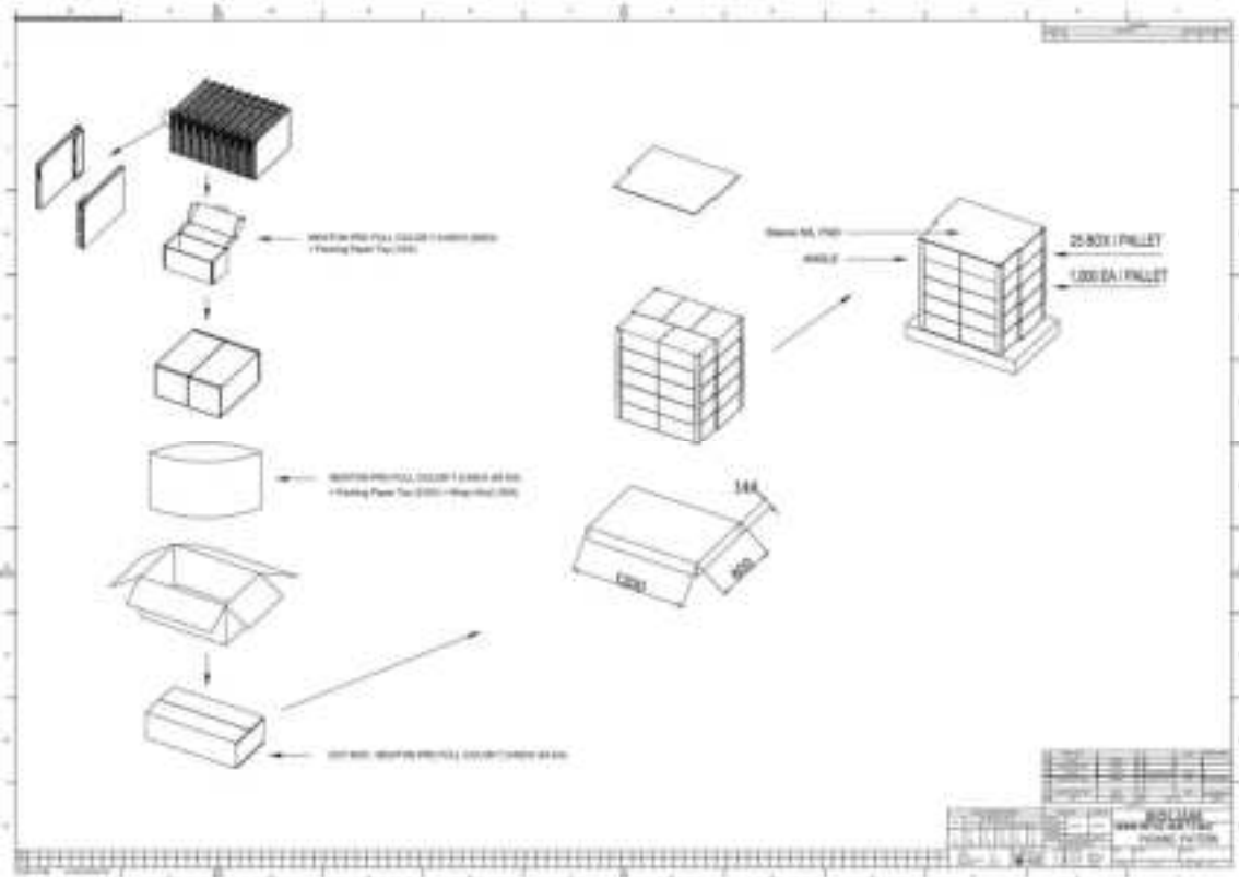
Figure 11. 7.3" Packing-Diagram (1,200 X 800)
