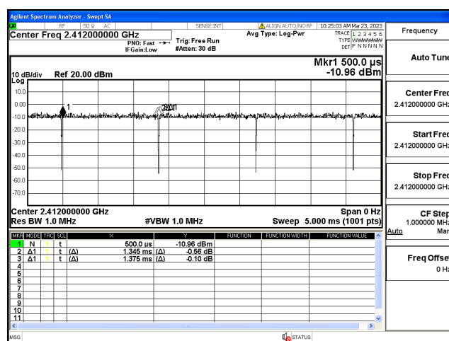
802.11g
