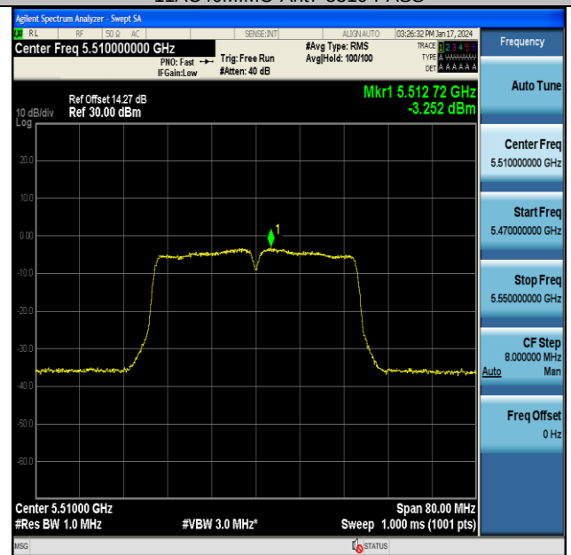
11AC40MIMO-Ant7-5510-PASS
