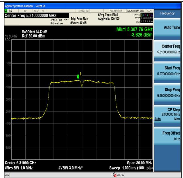
11AC40MIMO-Ant7-5310-PASS
