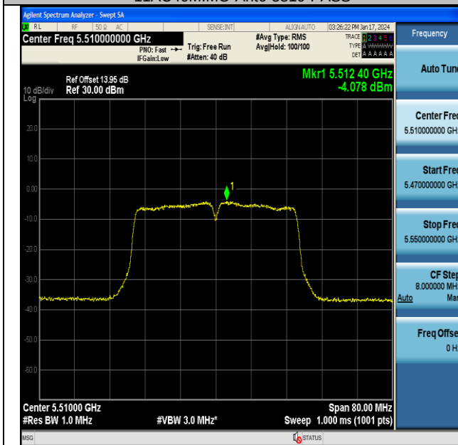
11AC40MIMO-Ant6-5510-PASS
