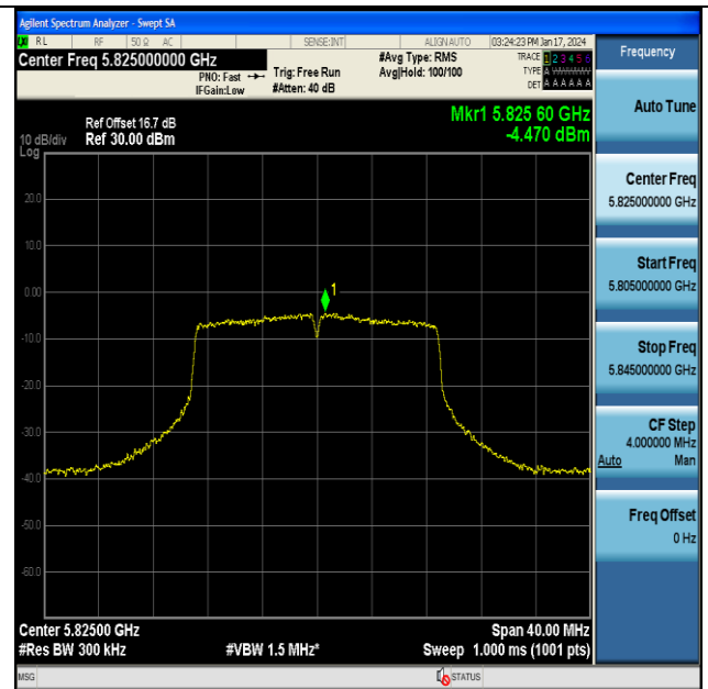
11AC20MIMO-Ant7-5825-PASS
