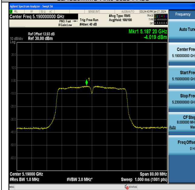
11AC40MIMO-Ant6-5190-PASS
