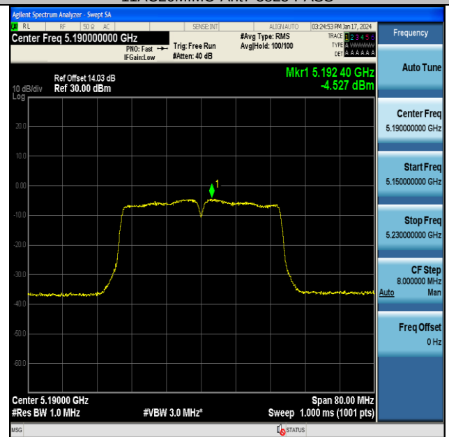
11AC40MIMO-Ant7-5190-PASS
