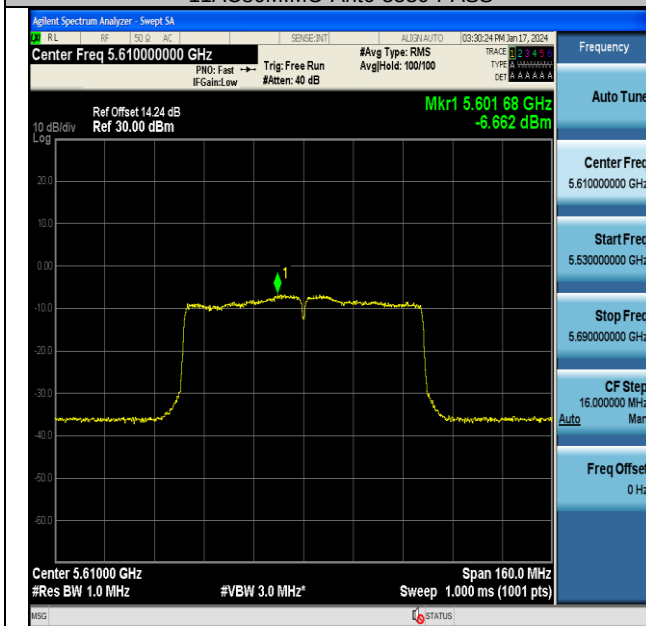
11AC80MIMO-Ant6-5610-PASS
