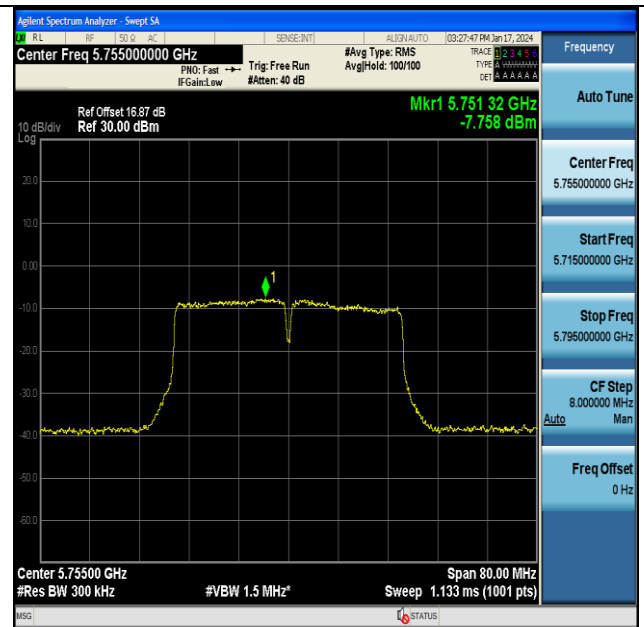
11AC40MIMO-Ant7-5755-PASS
