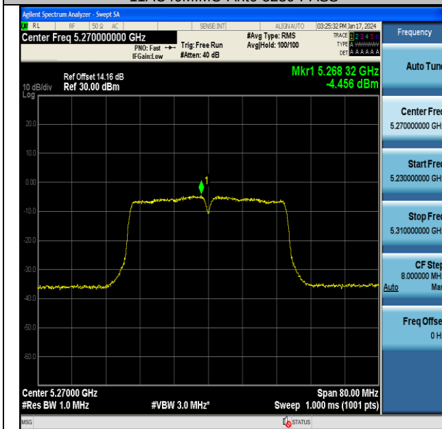
11AC40MIMO-Ant6-5270-PASS
