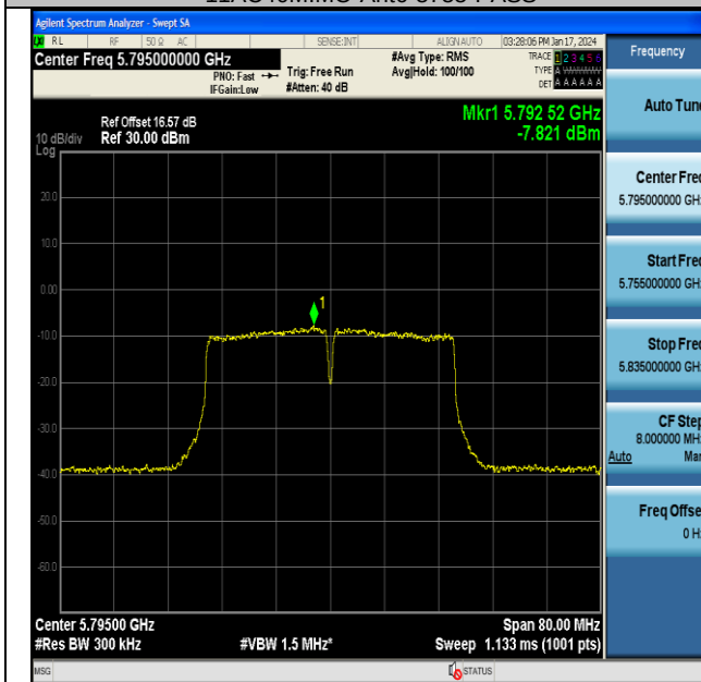
11AC40MIMO-Ant6-5795-PASS
