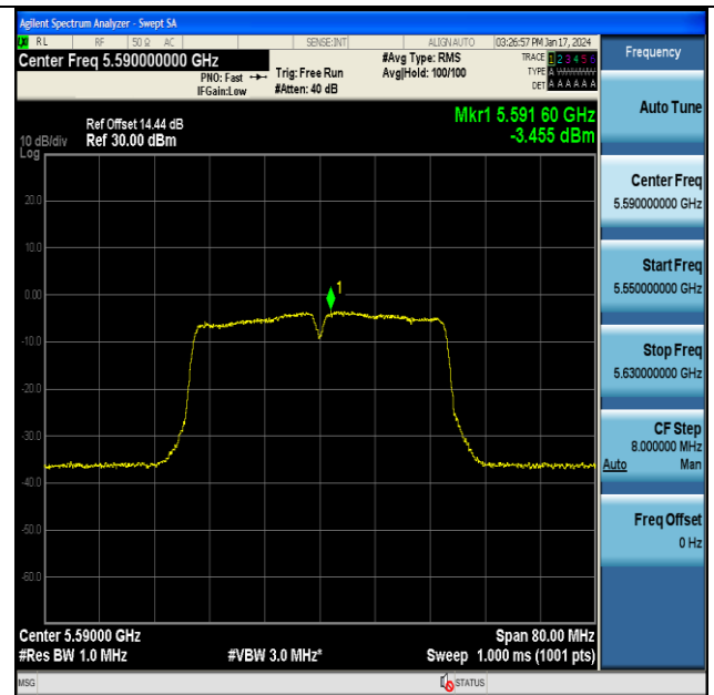
11AC40MIMO-Ant7-5590-PASS
