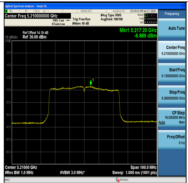
11AC80MIMO-Ant7-5210-PASS
