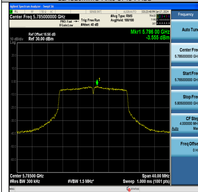
11AC20MIMO-Ant6-5785-PASS
