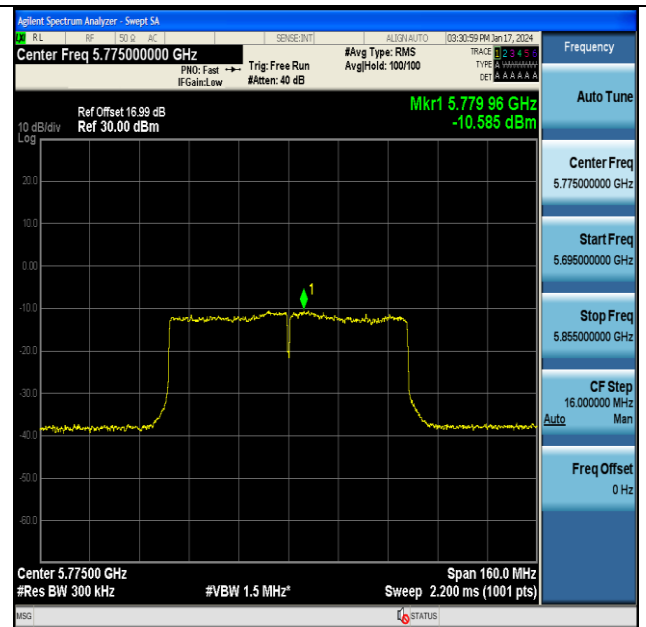
11AC80MIMO-Ant7-5775-PASS
