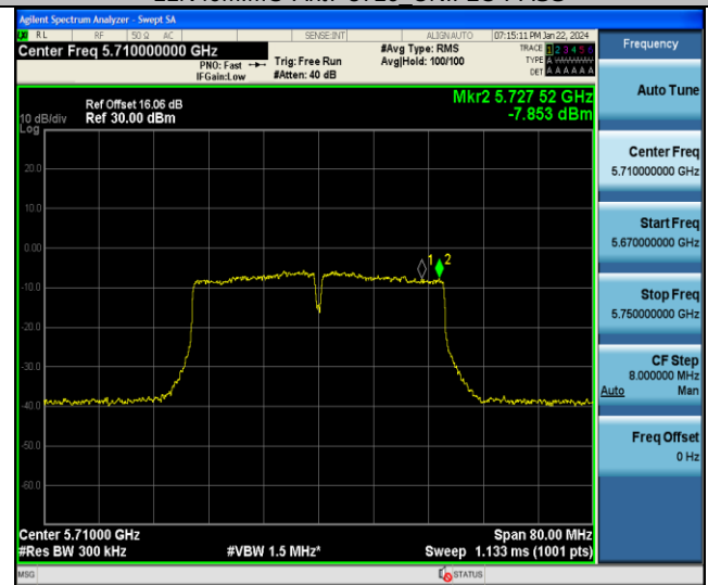
11N40MIMO-Ant7-5710 UNII-3-PASS
