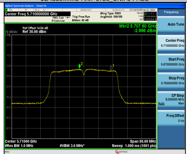
11AC40MIMO-Ant7-5710 UNII-2C-PASS
