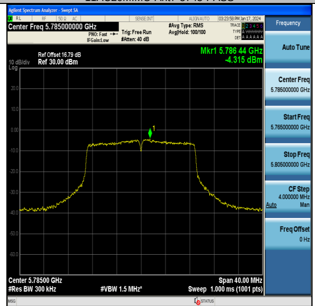
11AC20MIMO-Ant7-5785-PASS
