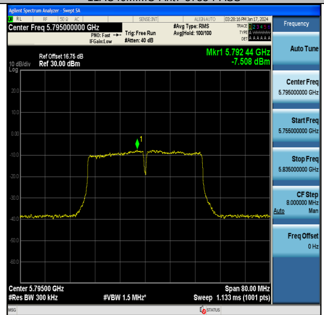
11AC40MIMO-Ant7-5795-PASS
