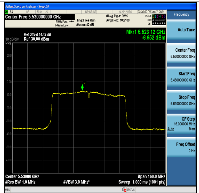
11AC80MIMO-Ant7-5530-PASS
