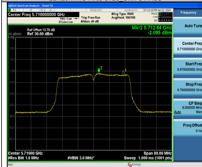
11N40MIMO-Ant6-5710 UNII-2C-PASS
