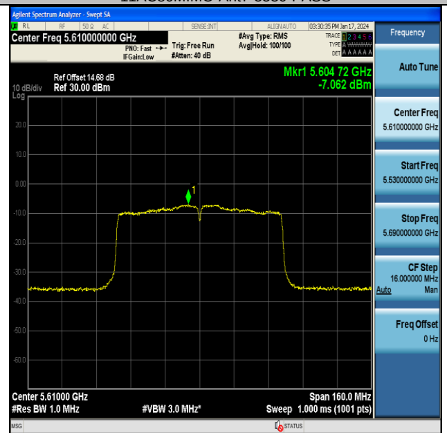
11AC80MIMO-Ant7-5610-PASS
