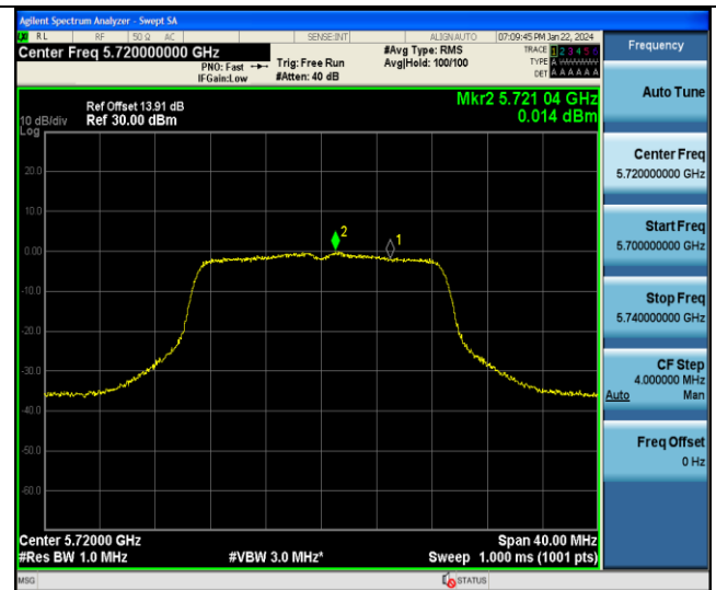
11AC20MIMO-Ant7-5720 UNII-2C-PASS
