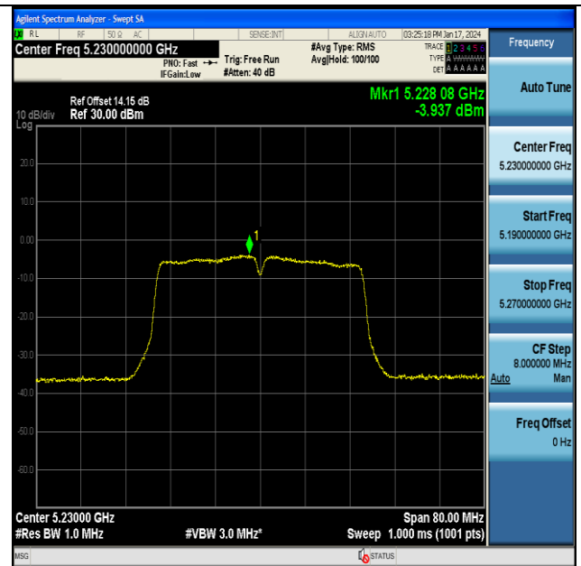
11AC40MIMO-Ant7-5230-PASS
