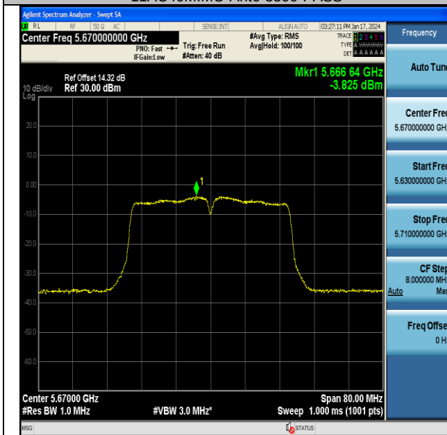
11AC40MIMO-Ant6-5670-PASS
