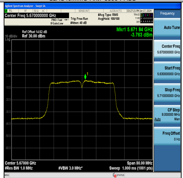
11AC40MIMO-Ant7-5670-PASS
