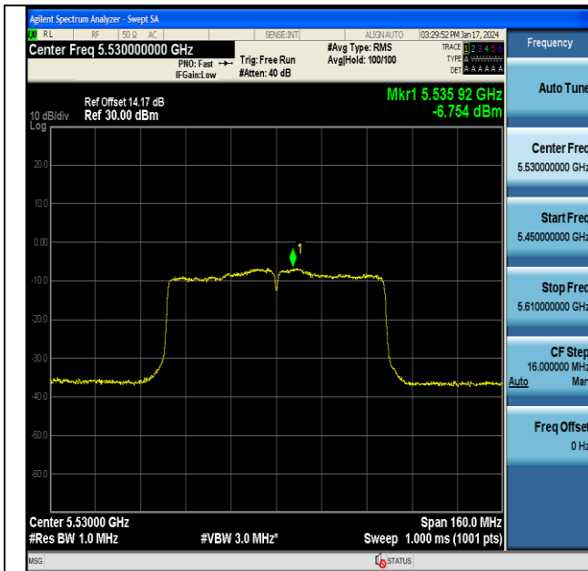
11AC80MIMO-Ant6-5530-PASS
