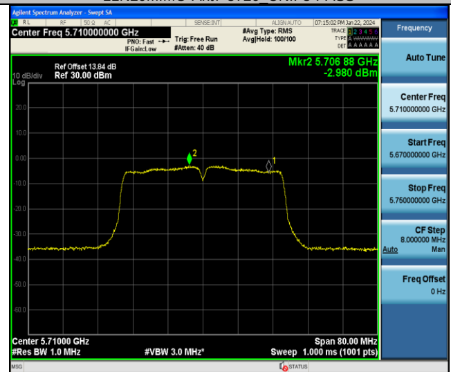
11N40MIMO-Ant7-5710 UNII-2C-PASS
