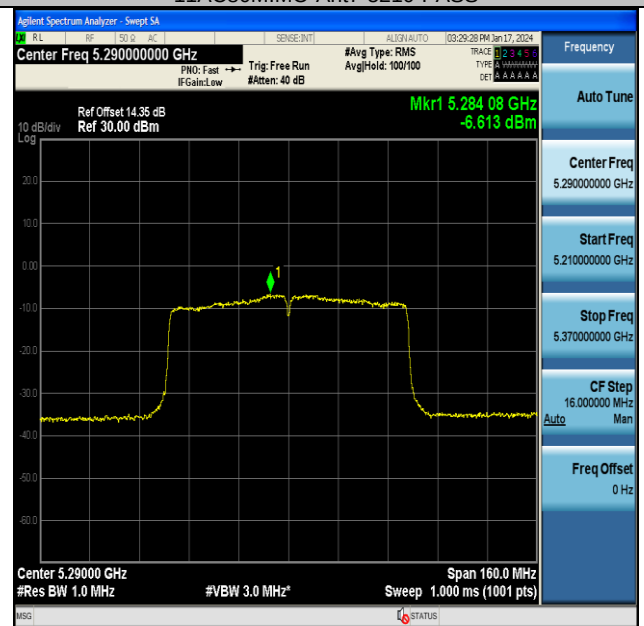
11AC80MIMO-Ant7-5290-PASS
