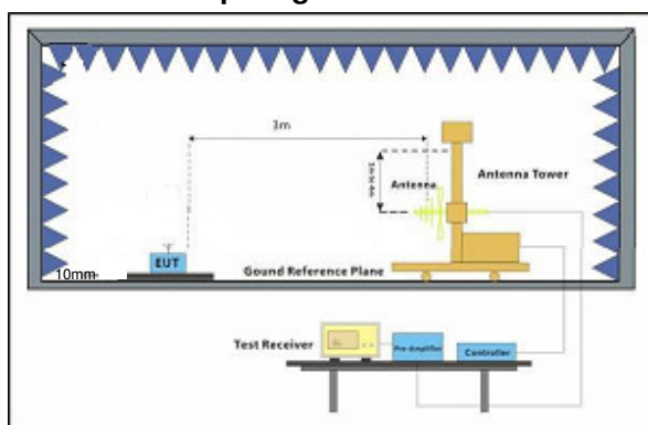
Below 1GHz
