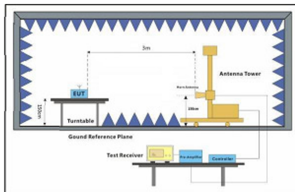
Above 1GHz
