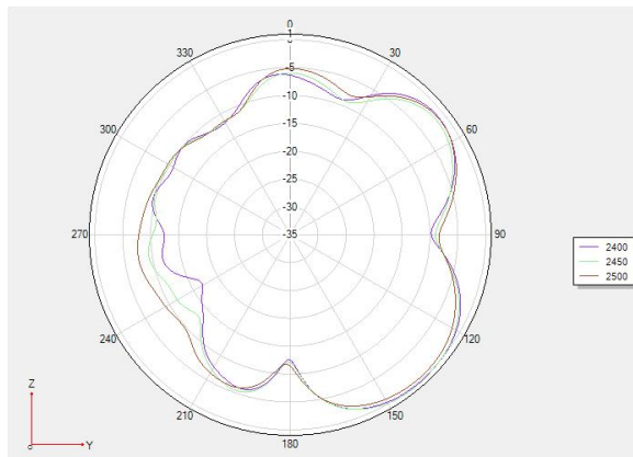
Phi 0 2Dfigure
