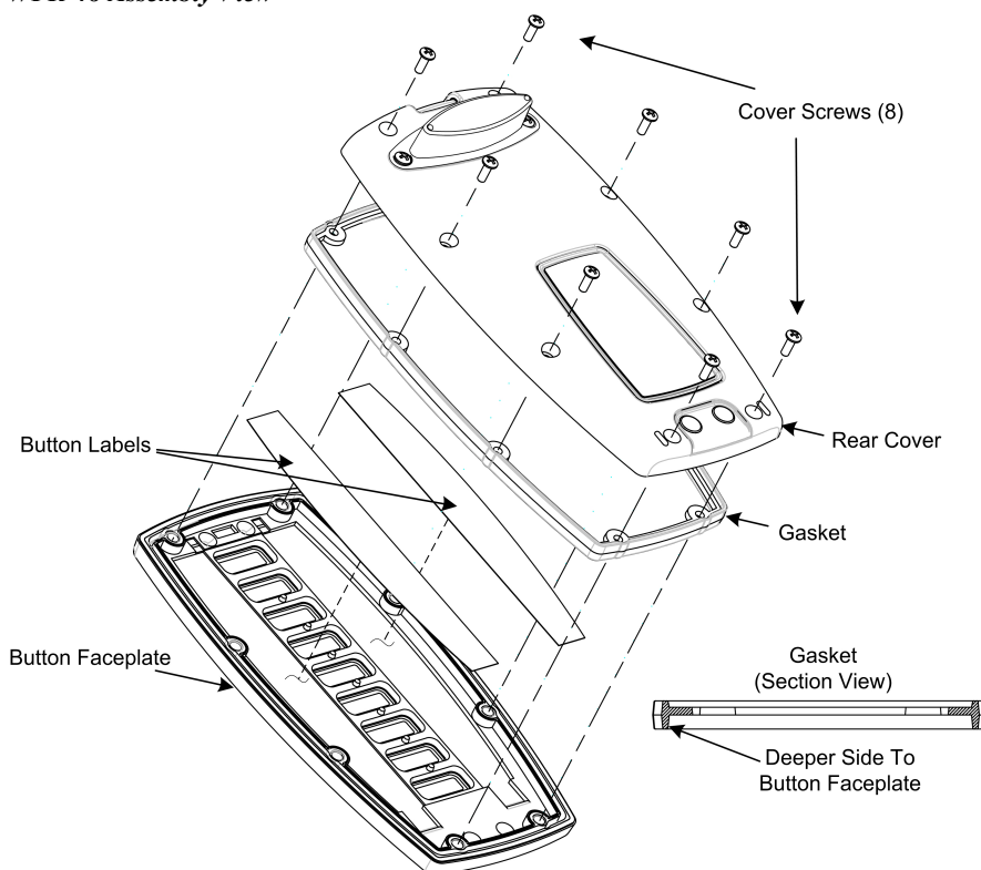
WPR-48 Assembly View
