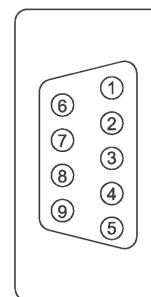
CONNECTOR, DB9, FEMALE (REAR VIEW)
