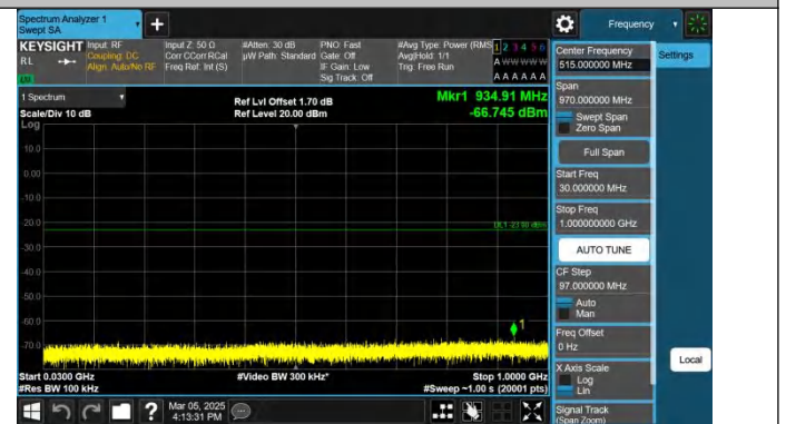
Band2-10MHz-QPSK-19150-1RB#49-30~1000-PASS
