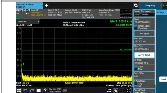
Band2-5MHz-QPSK-18625-1RB#24-0.15~30-PASS
