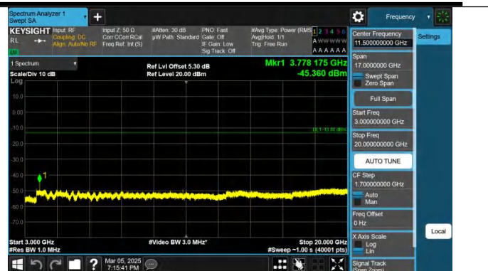
Band2-20MHz-QPSK-18900-1RB#99-3000~20000-PASS
