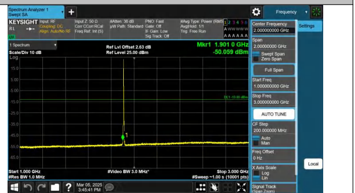
Band2-3MHz-QPSK-19185-1RB#0-1000~3000-PASS
