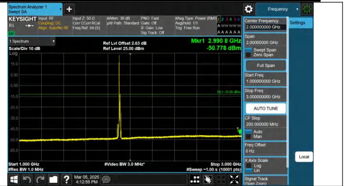
Band2-10MHz-QPSK-19150-1RB#0-1000~3000-PASS
