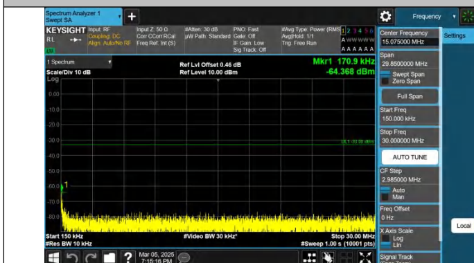
Band2-20MHz-QPSK-18900-1RB#99-0.15~30-PASS
