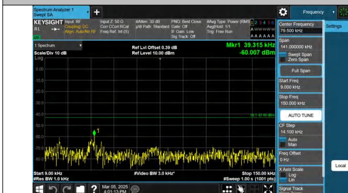
Band2-5MHz-QPSK-18900-1RB#0-0.009~0.15-PASS
