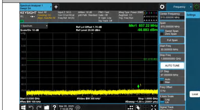
Band2-20MHz-QPSK-19100-1RB#0-30~1000-PASS
