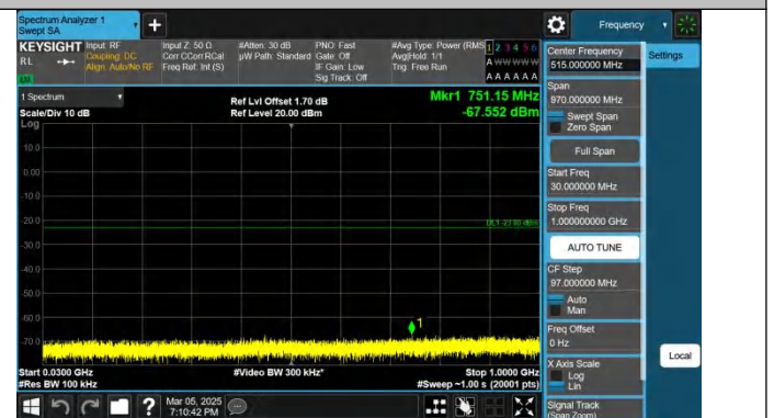
Band2-15MHz-QPSK-19125-1RB#74-30~1000-PASS
