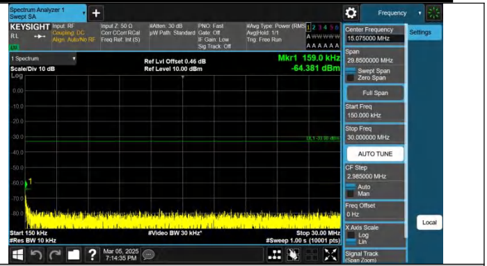
Band2-20MHz-QPSK-18900-1RB#0-0.15~30-PASS
