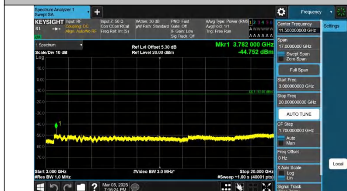
Band2-20MHz-QPSK-19100-1RB#0-3000~20000-PASS
