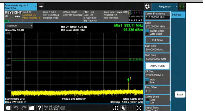
Band2-10MHz-QPSK-18900-1RB#49.30~1000-PASS
