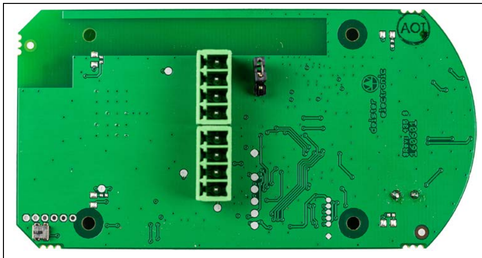
PCB Rear
