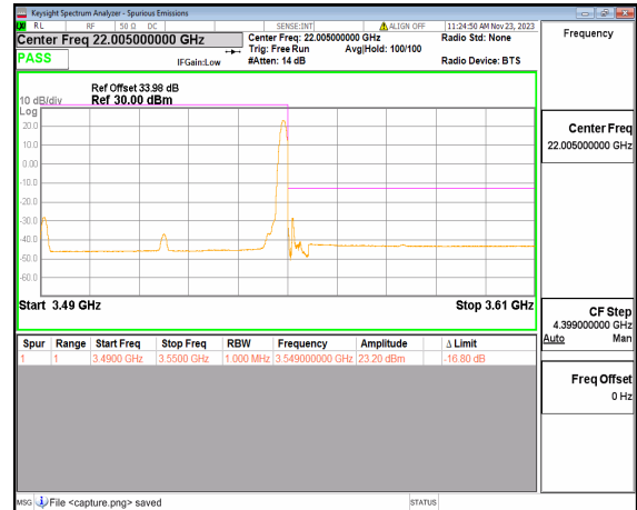
n77(3450-3550MHz) 60M DFT-s-OFDM QPSK Edge_1RB_Right High
