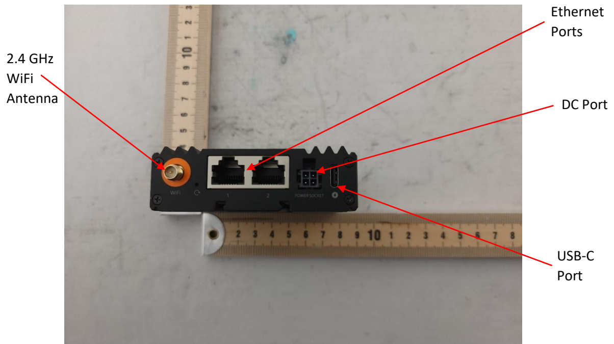
Photograph 7: Bottom View of DUT
