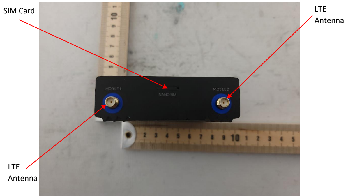
Photograph 5: Top View of DUT
