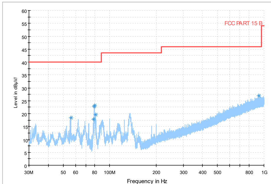
Fig.159 Radiated emission: 11b,Ch11, 30MHz-1GHz
