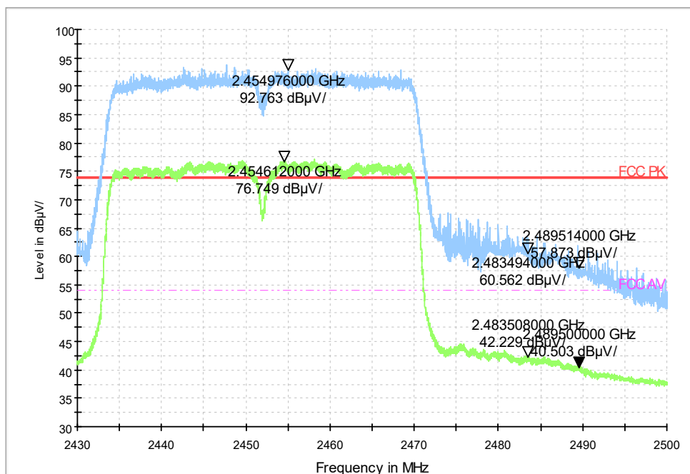
Fig.128 Frequency Band Edge: Ch9,11n(40M)
