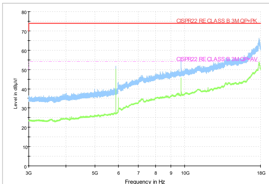
Fig.167 Radiated emission: 11g,Ch6, 3GHz-18GHz
