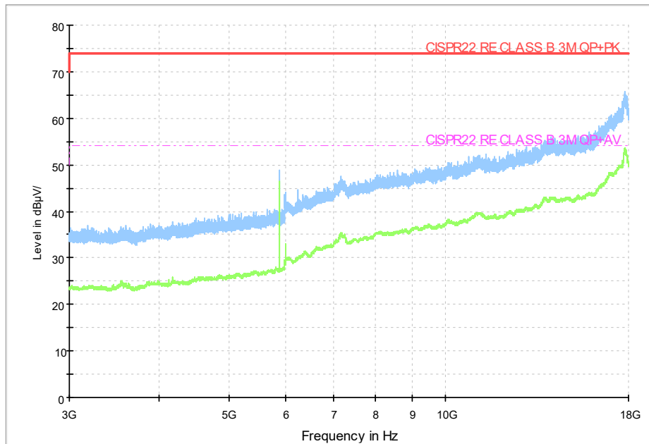
Fig.179 Radiated emission:11n,20M, Ch11, 3GHz-18GHz
