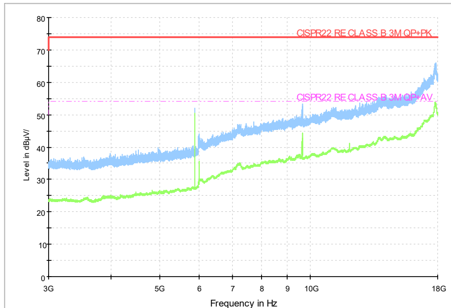
Fig.155 Radiated emission: 11b,Ch1, 3GHz-18GHz
