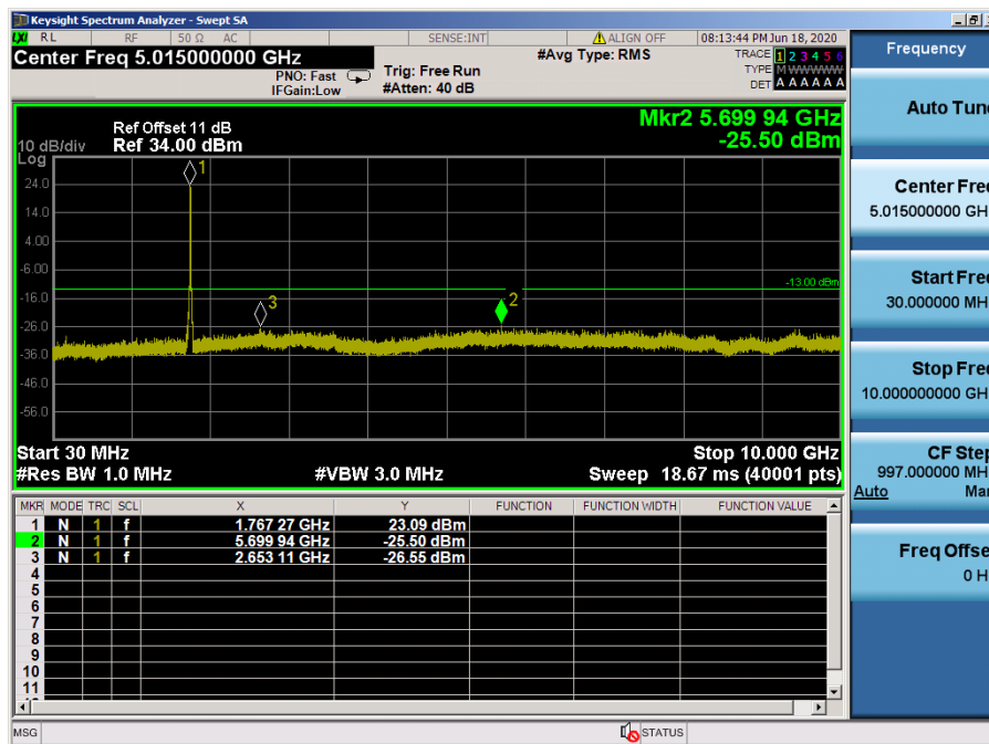
LTE Band 66, 4 / 20 MHz / QPSK - RB Size/Offset (100/0) – High Channel
