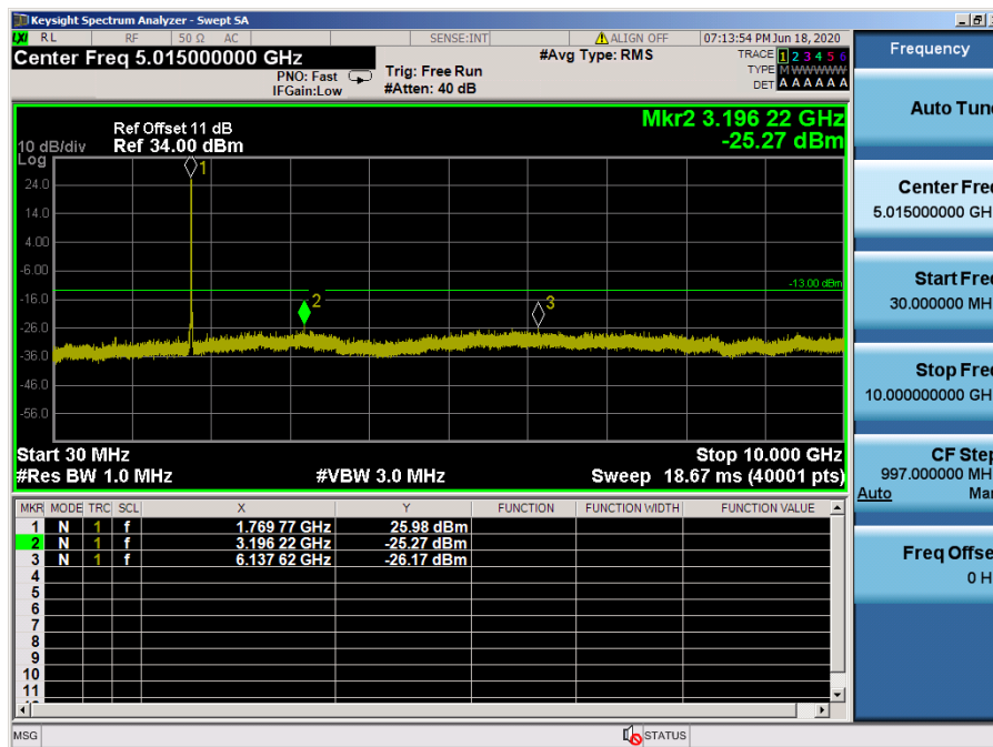
LTE Band 66, 4 / 15 MHz / QPSK - RB Size/Offset (36/18) – High Channel
