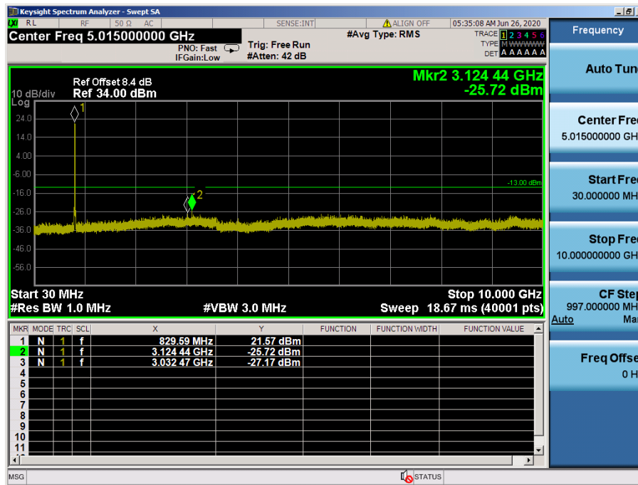
LTE Band 5 / 10 MHz / 64QAM - RB Size/Offset (50/0) – Low Channel
