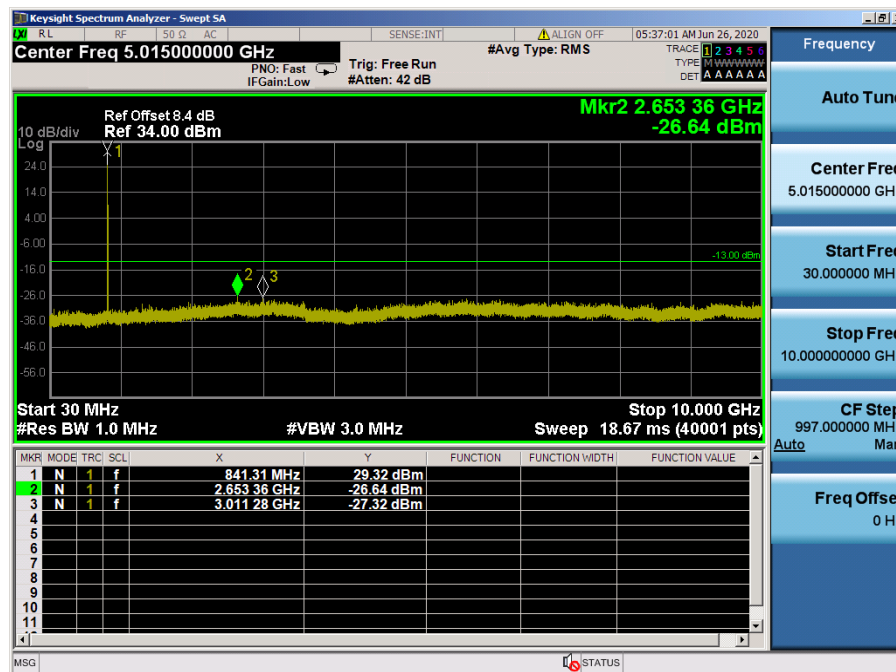
LTE Band 5 / 10 MHz / 64QAM - RB Size/Offset (1/49) – Mid Channel
