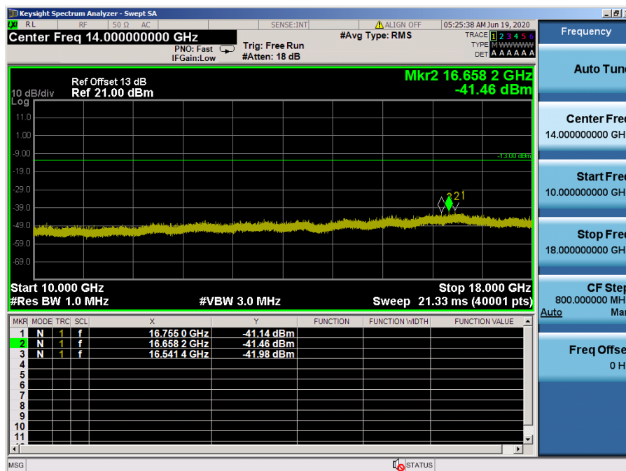
LTE Band 66, 4 / 15 MHz / 64QAM - RB Size/Offset (36/39) – Mid Channel
