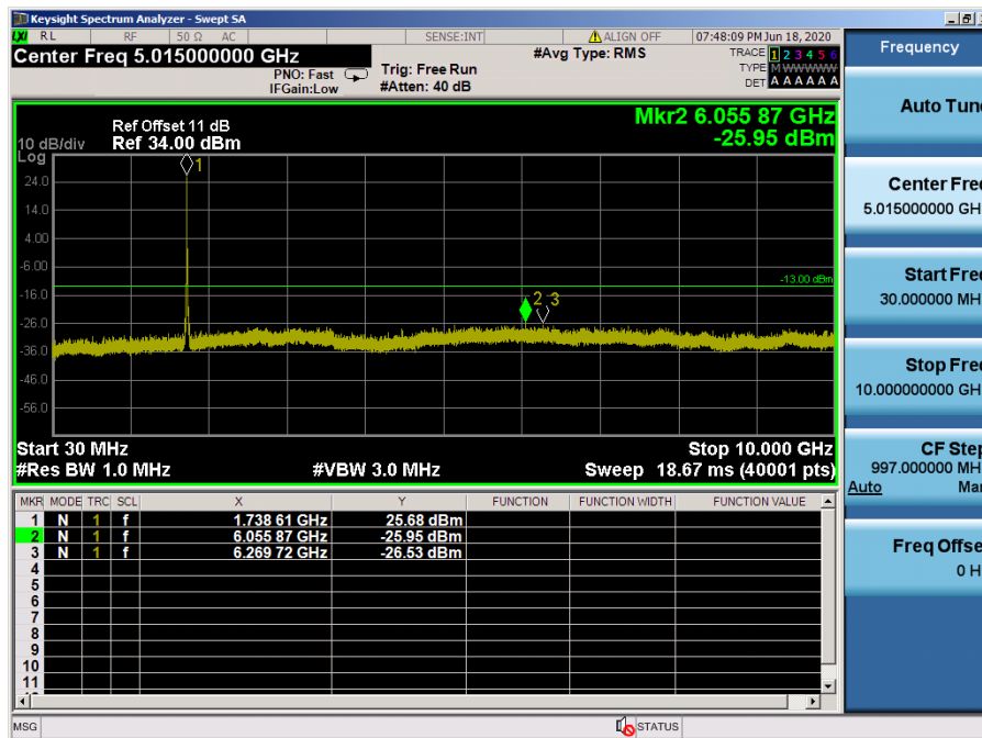
LTE Band 66, 4 / 20 MHz / QPSK - RB Size/Offset (50/0) – Mid Channel
