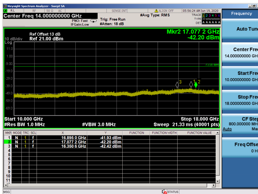
LTE Band 66, 4 / 20 MHz / 64QAM - RB Size/Offset (1/50) – Low Channel
