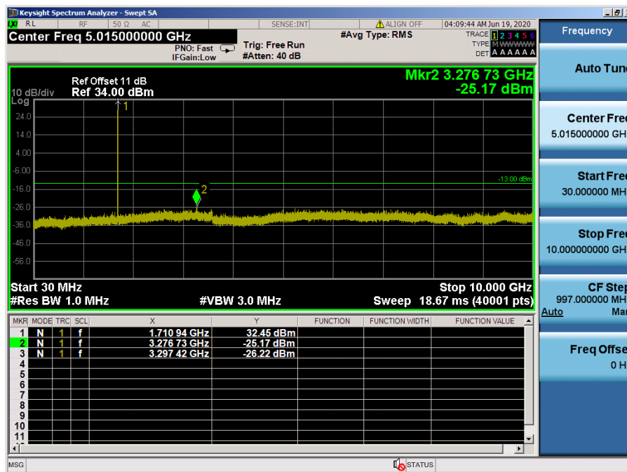
LTE Band 66, 4 / 10 MHz / 64QAM - RB Size/Offset (1/0) – Low Channel
