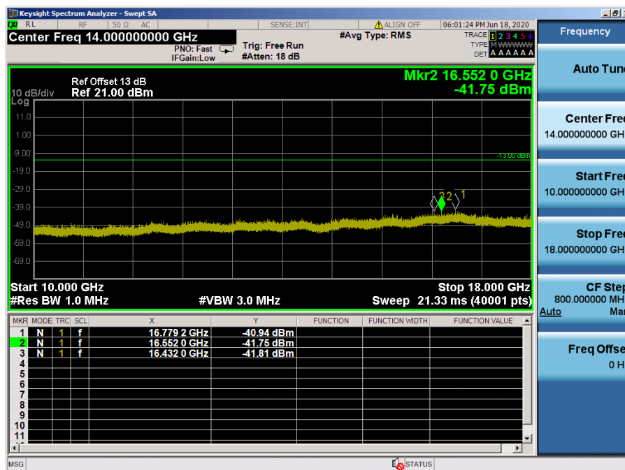
LTE Band 66, 4 / 10 MHz / QPSK - RB Size/Offset (25/25) – Mid Channel
