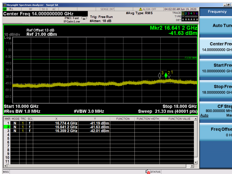
LTE Band 66, 4 / 5 MHz / 64QAM - RB Size/Offset (12/13) – High Channel
