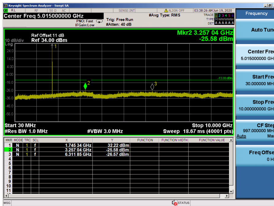
LTE Band 66, 4 / 5 MHz / 64QAM - RB Size/Offset (1/12) – Mid Channel
