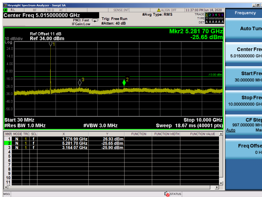
LTE Band 66, 4 / 10 MHz / 16QAM - RB Size/Offset (25/12) – High Channel
