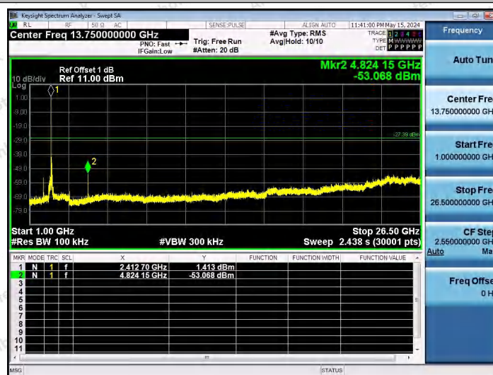
11B-Ant1-2412-1000~26500-PASS
