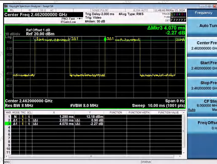
NTNV-11G-Ant1-2462
