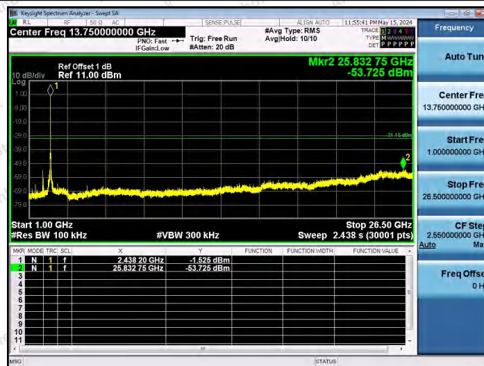
11N20SISO-Ant1-2437-1000~26500-PASS
