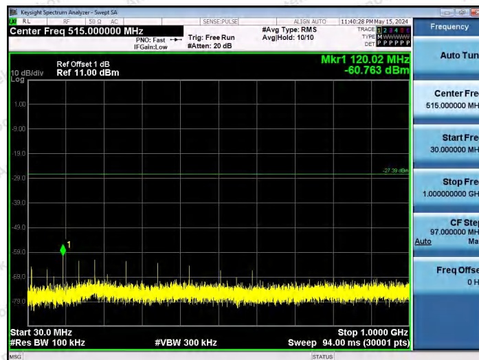
11B-Ant1-2412-30~1000-PASS
