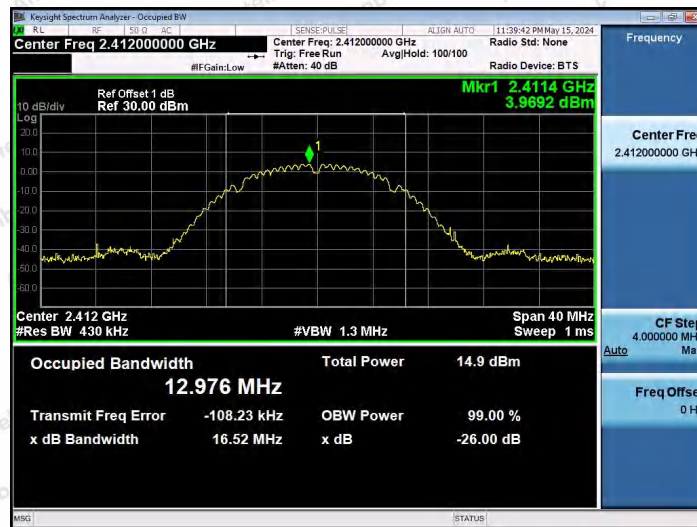
11B-Ant1-2412
