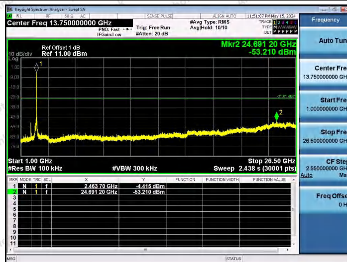
11G-Ant1-2462-1000~26500-PASS
