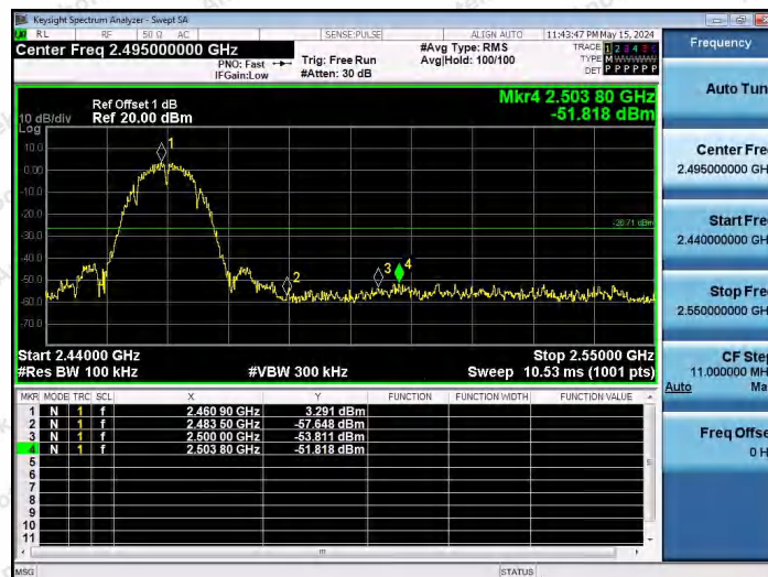
11B-Ant1-2462-PASS
