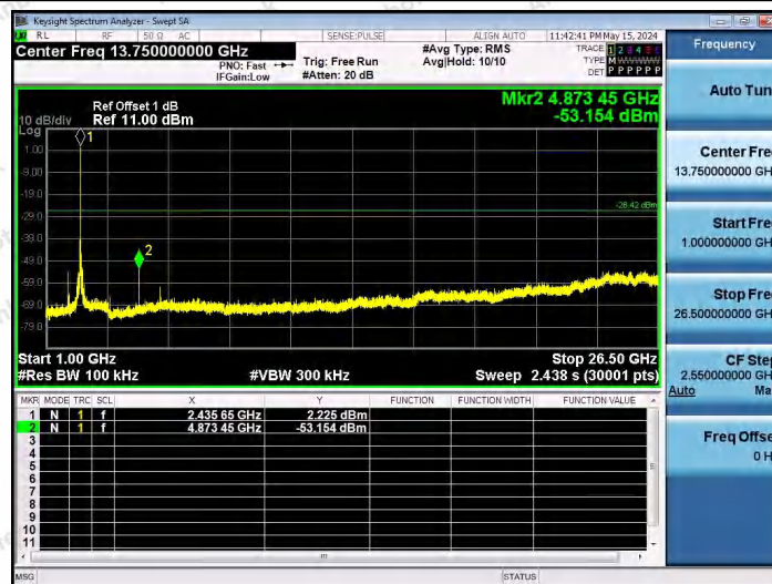
11B-Ant1-2437-1000~26500-PASS
