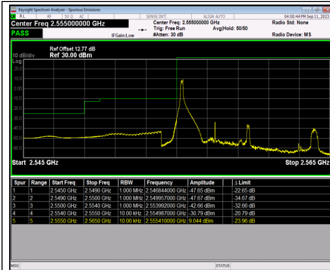
Band41-5MHz-64QAM-40265-25RB#0
