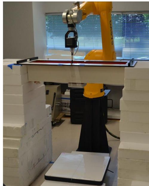
Figure 16 - SAR measurement test setup
