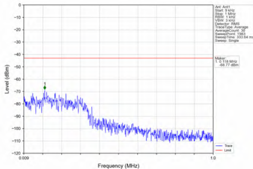
n41_30kHz_SISO_NTNV_30MHz_DFT-s-OFDM QPSK_2674.98MHz_Edge_1RB_Right
