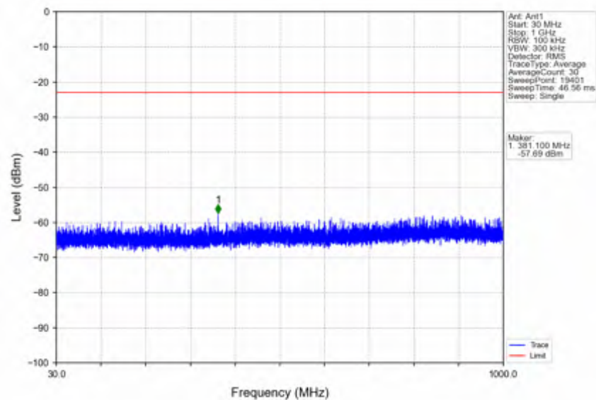
n41_30kHz_SISO_NTNV_40MHz_DFT-s-OFDM QPSK_2670MHz_Edge_1RB_Right
