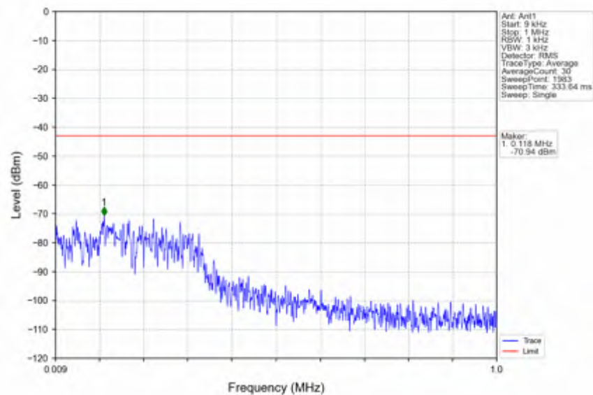
n41_30kHz_SISO_NTNV_40MHz_DFT-s-OFDM QPSK_2670MHz_Edge_1RB_Right
