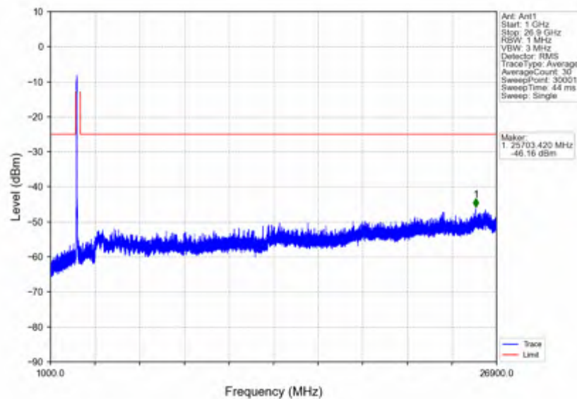
n41_30kHz_SISO_NTNV_40MHz_CP-OFDM QPSK_2516.01MHz_Outer_Full
