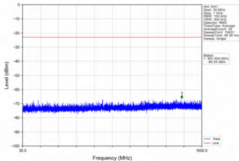
n41_30kHz_SISO_NTNV_20MHz_DFT-s-OFDM QPSK_2506.02MHz_Outer_Full
