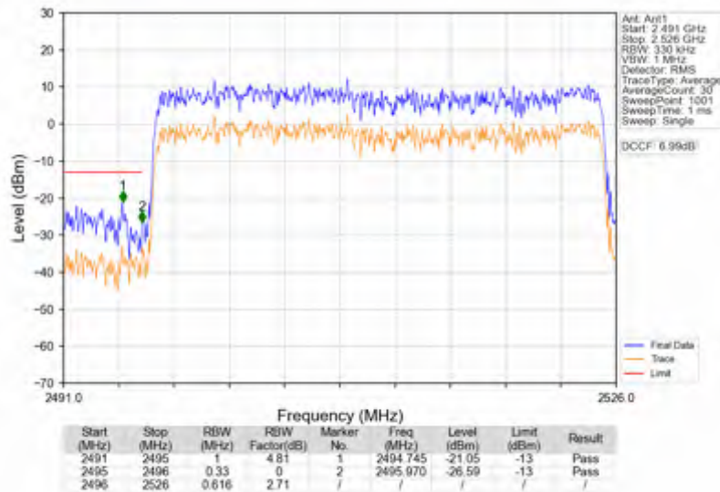
n41_30kHz_SISO_NTNV_30MHz_CP-OFDM QPSK_2511MHz_Outer_Full
