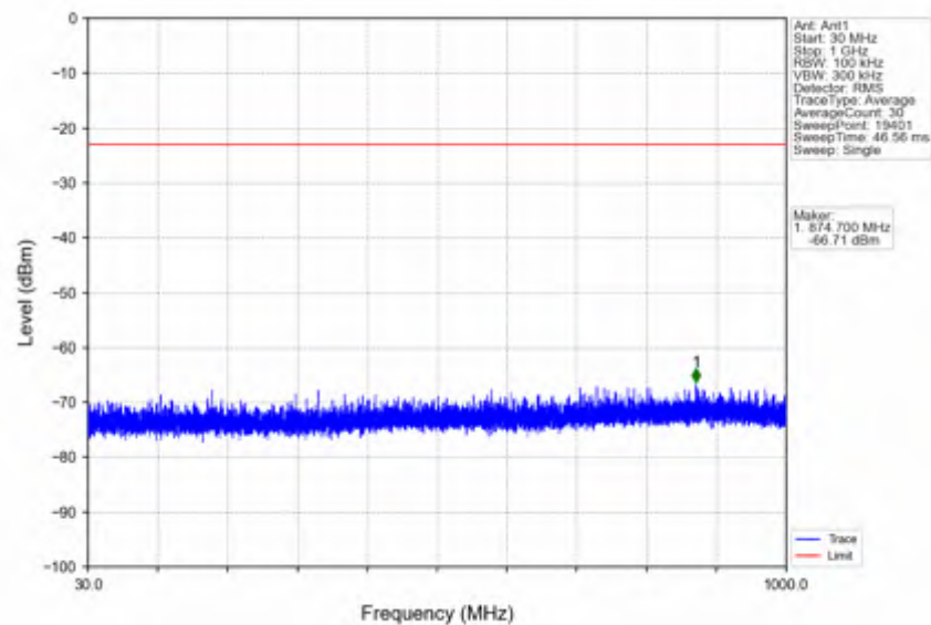
n41_30kHz_SISO_NTNV_20MHz_CP-OFDM QPSK_2679.99MHz_Outer_Full
