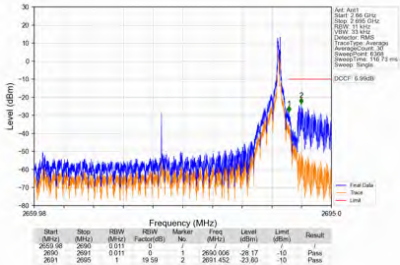
n41_30kHz_SISO_NTNV_30MHz_DFT-s-OFDM QPSK_2674.98MHz_Edge_1RB_Right
