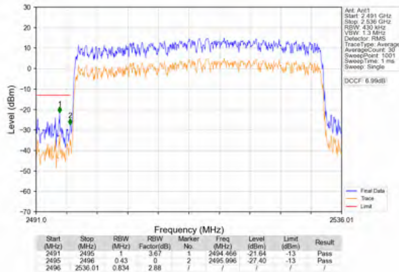
n41_30kHz_SISO_NTNV_40MHz_DFT-s-OFDM QPSK_2516.01MHz_Outer_Full
