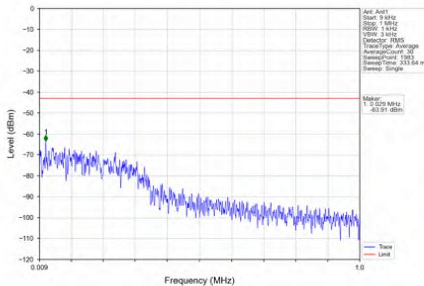
n41_30kHz_SISO_NTNV_30MHz_CP-OFDM_QPSK_2511MHz_Edge_1RB_Left
