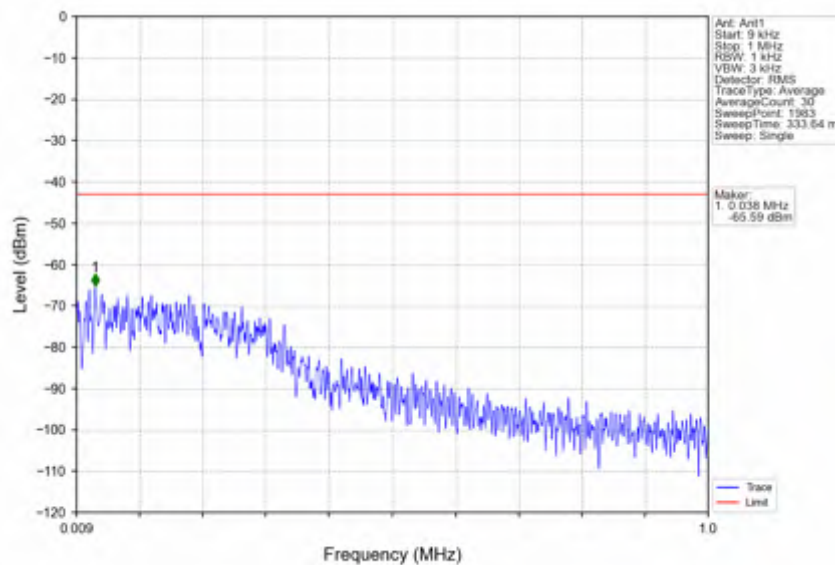
n41_30kHz_SISO_NTNV_40MHz_CP-OFDM QPSK_2670MHz_Edge_1RB_Right
