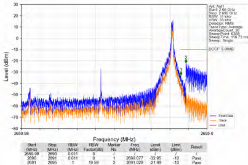
n41_30kHz_SISO_NTNV_30MHz_DFT-s-OFDM QPSK_2674.98MHz_Inner_1RB_Right
