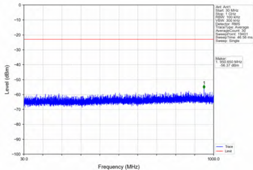
n41_30kHz_SISO_NTNV_40MHz_CP-OFDM QPSK_2670MHz_Edge_1RB_Right
