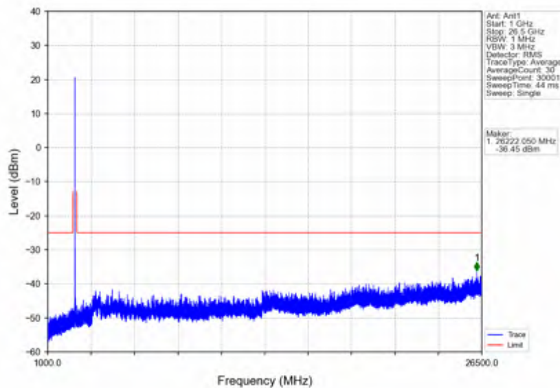
n41_30kHz_SISO_NTNV_20MHz_DFT-s-OFDM QPSK_2679.99MHz_Edge_1RB_Right
