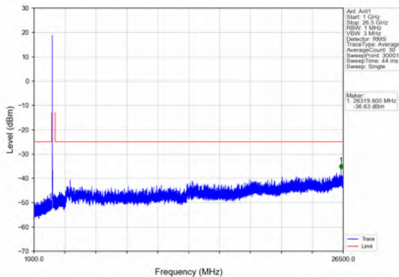
n41_30kHz_SISO_NTNV_40MHz_DFT-s-OFDM QPSK_2516.01MHz_Edge_1RB_Left
