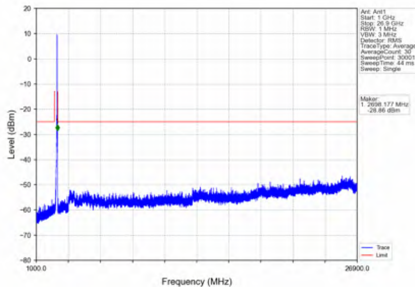
n41 30kHz SISO NTV 40MHz CP-OFDM QPSK 2670MHz Outer Full
