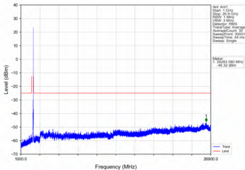
n41_30kHz_SISO_NTNV_30MHz_CP-OFDM QPSK_2674.98MHz_Outer_Full
