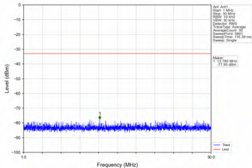
n41_30kHz_SISO_NTV_40MHz_CP-OFDM_QPSK_2670MHz_Outer_Full
