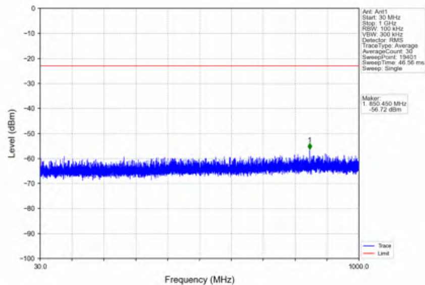
n41_30kHz_SISO_NTNV_30MHz_CP-OFDM QPSK_2592.99MHz_Edge_1RB_Left
