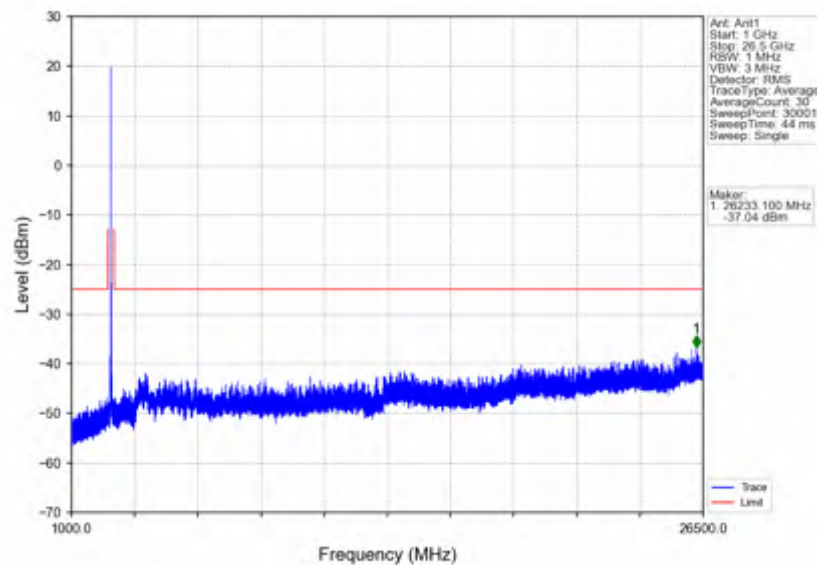
n41_30kHz_SISO_NTNV_30MHz_CP-OFDM QPSK_2592.99MHz_Edge_1RB_Left
