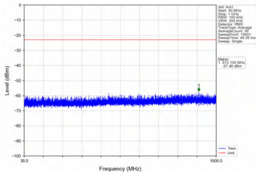
n41_30kHz_SISO_NTNV_30MHz_CP-OFDM_QPSK_2511MHz_Edge_1RB_Left
