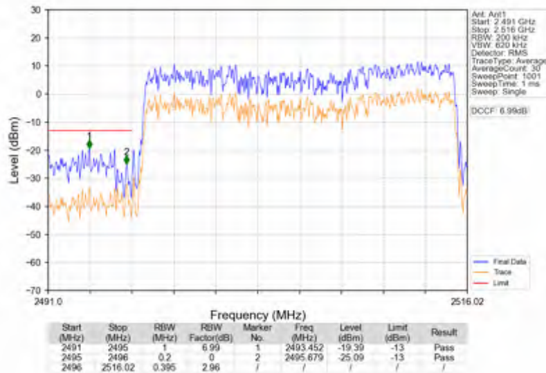
n41_30kHz_SISO_NTNV_20MHz_CP-OFDM QPSK_2506.02MHz_Outer_Full
