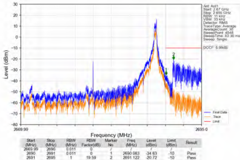
n41_30kHz_SISO_NTNV_20MHz_DFT-s-OFDM QPSK_2679.99MHz_Inner_1RB_Right
