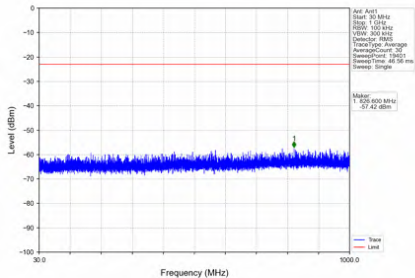
n41_30kHz_SISO_NTNV_30MHz_CP-OFDM QPSK_2674.98MHz_Edge_1RB_Right
