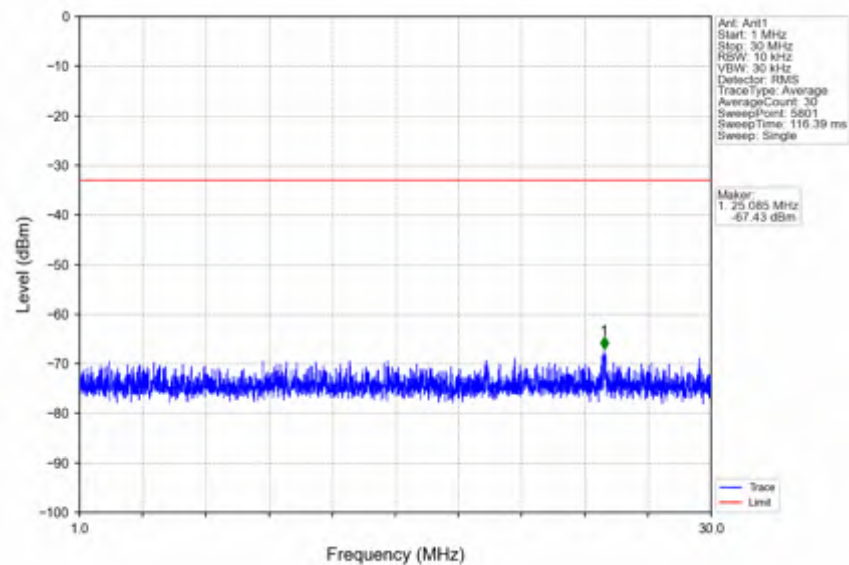
n41_30kHz_SISO_NTNV_15MHz_CP-OFDM QPSK_2592.99MHz_Edge_1RB_Left
