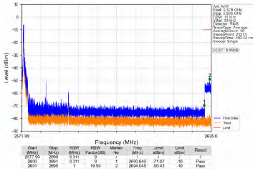
n41_30kHz_SISO_NTNV_30MHz_DFT-s-OFDM QPSK_2592.99MHz_Edge_1RB_Left
