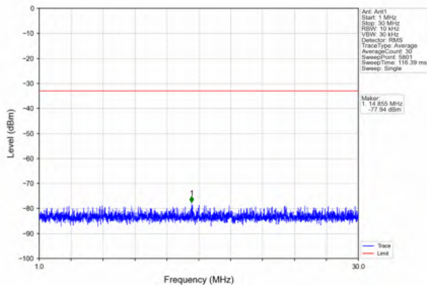
n41_30kHz_SISO_NTNV_15MHz_CP-OFDM QPSK_2682.48MHz_Inner_1RB_Right
