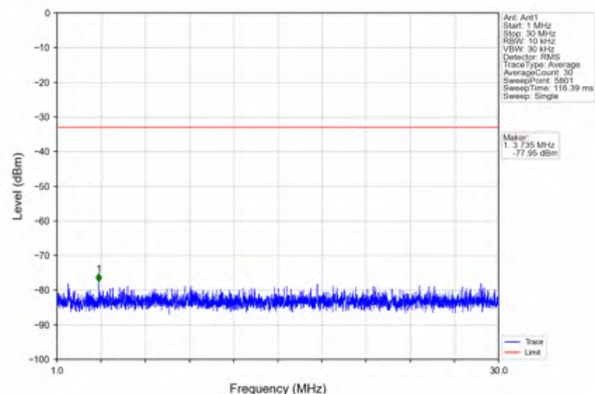
n41_30kHz_SISO_NTNV_15MHz_CP-OFDM QPSK_2682.48MHz_Outer_Full
