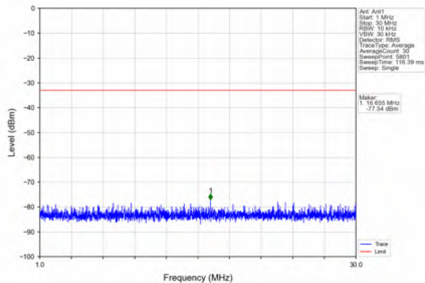
n41_30kHz_SISO_NTNV_30MHz_CP-OFDM QPSK_2674.98MHz_Outer_Full
