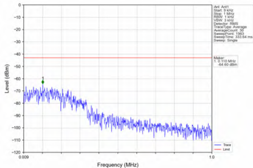
n41_30kHz_SISO_NTNV_40MHz_CP-OFDM QPSK_2592.99MHz_Edge_1RB_Left
