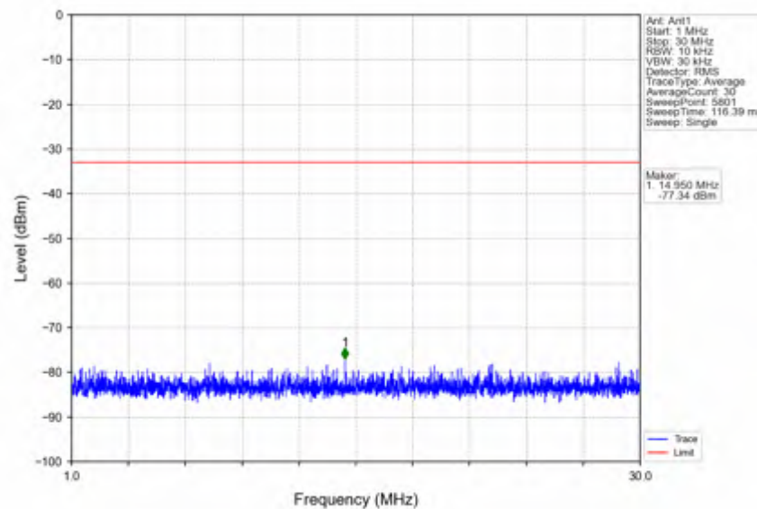
n41_30kHz_SISO_NTNV_40MHz_DFT-s-OFDM QPSK_2516.01MHz_Outer_Full
