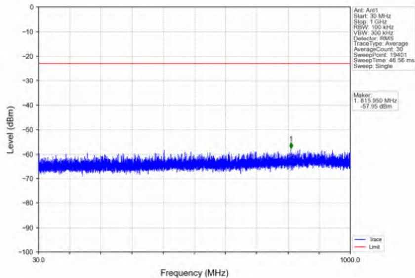
n41_30kHz_SISO_NTNV_30MHz_DFT-s-OFDM QPSK_2511MHz_Edge_1RB_Left
