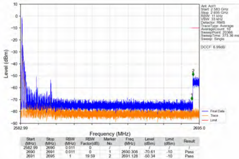
n41_30kHz_SISO_NTNV_20MHz_DFT-s-OFDM_QPSK_2592.99MHz_Edge_1RB_Left
