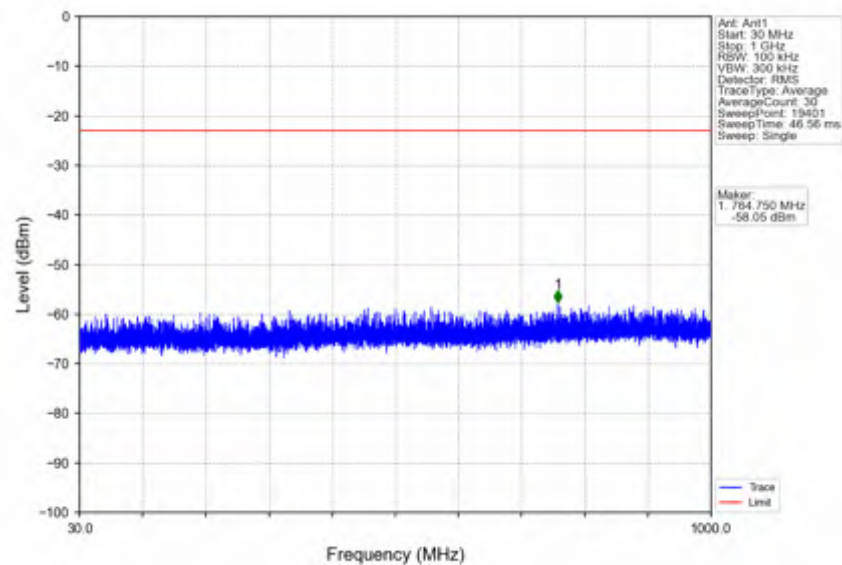
n41_30kHz_SISO_NTNV_40MHz_CP-OFDM QPSK_2516.01MHz_Edge_1RB_Left
