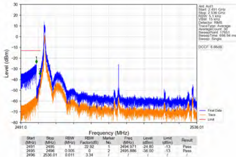
n41_30kHz_SISO_NTNV_40MHz_DFT-s-OFDM_PI/2_BPSK_2516.01MHz_Edge_1RB_Left
