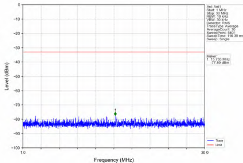
n41_30kHz_SISO_NTNV_30MHz_DFT-s-OFDM QPSK_2674.98MHz_Outer_Full
