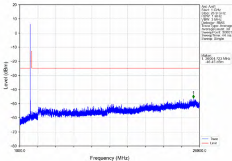
n41_30kHz_SISO_NTNV_30MHz_DFT-s-OFDM PI/2 BPSK_2592.99MHz_Edge_1RB_Left
