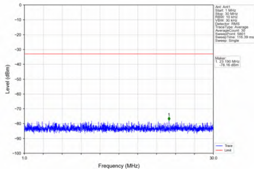
n41_30kHz_SISO_NTNV_20MHz_CP-OFDM QPSK_2506.02MHz_Outer_Full
