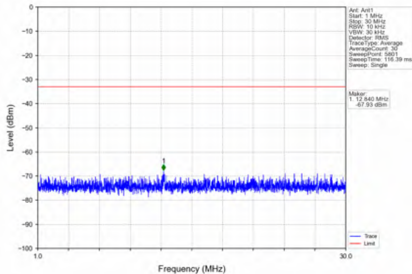
n41_30kHz_SISO_NTNV_40MHz_DFT-s-OFDM QPSK_2592.99MHz_Edge_1RB_Left
