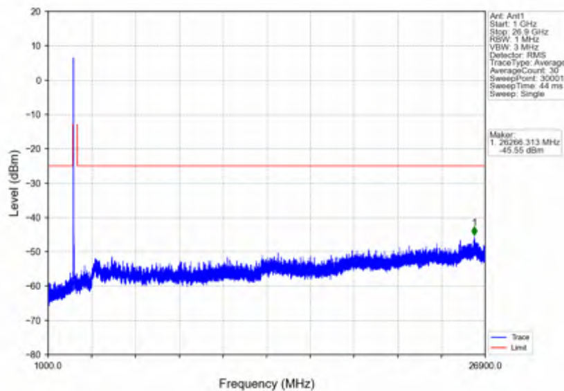
n41_30kHz_SISO_NTNV_40MHz_CP-OFDM QPSK_2592.99MHz_Edge_1RB_Left
