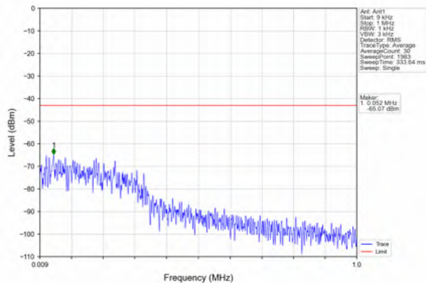
n41_30kHz_SISO_NTNV_30MHz_CP-OFDM QPSK_2592.99MHz_Edge_1RB_Left
