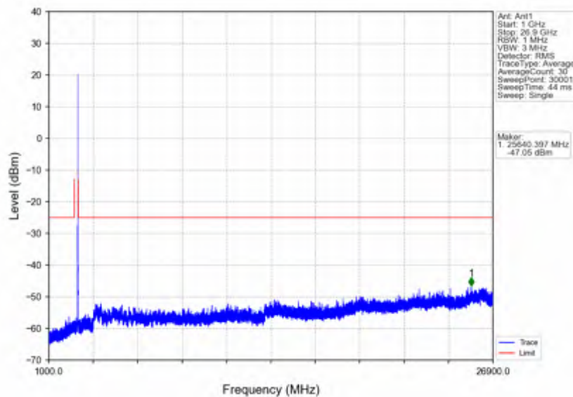
n41_30kHz_SISO_NTNV_15MHz_CP-OFDM_QPSK_2682.48MHz_Outer_Full
