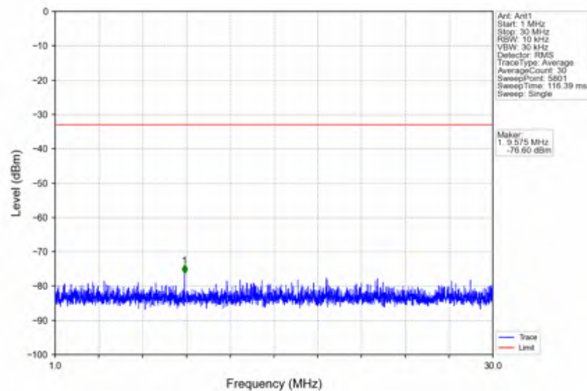
n41_30kHz_SISO_NTNV_20MHz_DFT-s-OFDM QPSK_2506.02MHz_Outer_Full
