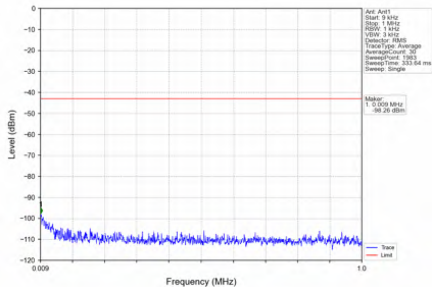
n41_30kHz_SISO_NTNV_40MHz_DFT-s-OFDM_PI/2_BPSK_2670MHz_Outer_Full
