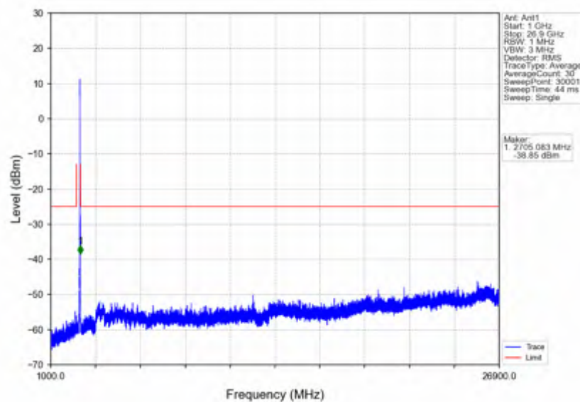
n41 30kHz SISO NTNV 15MHz CP-OFDM QPSK 2682.48MHz Outer Full
