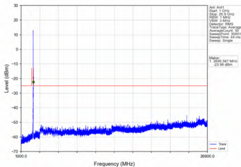
n41_30kHz_SISO_NTNV_20MHz_CP-OFDM QPSK_2679.99MHz_Outer_Full
