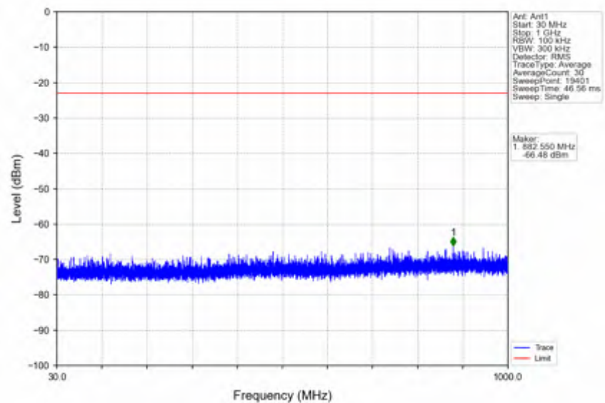
n41_30kHz_SISO_NTNV_30MHz_DFT-s-OFDM QPSK_2511MHz_Outer_Full
