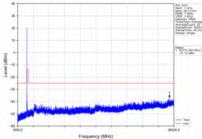
n41_30kHz_SISO_NTNV_30MHz_DFT-s-OFDM QPSK_2511MHz_Edge_1RB_Left
