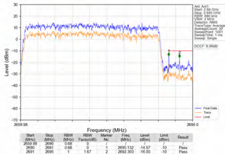
n41_30kHz_SISO_NTNV_30MHz_DFT-s-OFDM QPSK_2674.98MHz_Outer_Full
