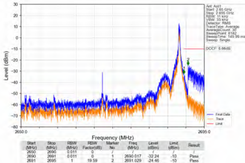
n41_30kHz_SISO_NTNV_40MHz_DFT-s-OFDM QPSK_2670MHz_Edge_1RB_Right
