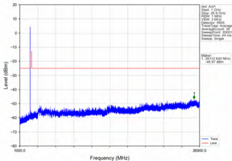
n41_30kHz_SISO_NTNV_15MHz_CP-OFDM_QPSK_2592.99MHz_Edge_1RB_Left
