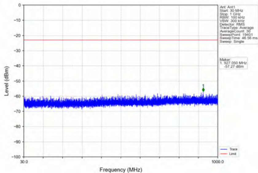
n41_30kHz_SISO_NTNV_40MHz_DFT-s-OFDM QPSK_2516.01MHz_Edge_1RB_Left
