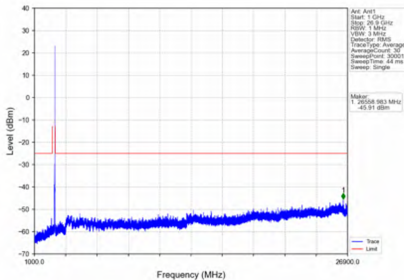
n41_30kHz_SISO_NTNV_20MHz_CP-OFDM QPSK_2679.99MHz_Outer_Full
