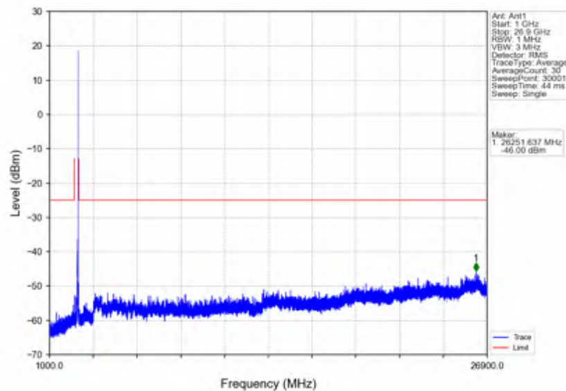
n41_30kHz_SISO_NTNV_40MHz_DFT-s-OFDM QPSK_2670MHz_Edge_1RB_Right
