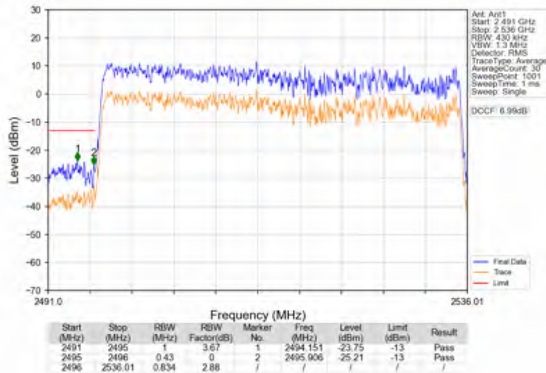
n41_30kHz_SISO_NTNV_40MHz_CP-OFDM QPSK_2516.01MHz_Outer_Full
