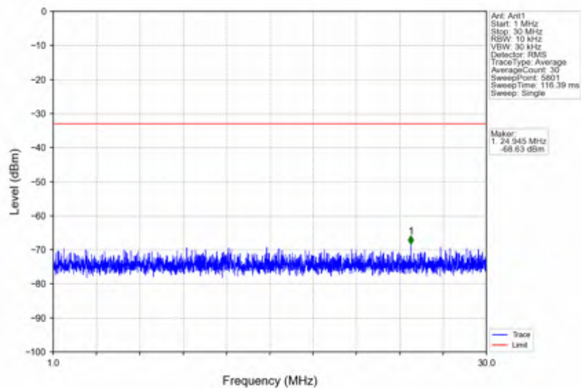
n41_30kHz_SISO_NTNV_40MHz_DFT-s-OFDM QPSK_2516.01MHz_Edge_1RB_Left
