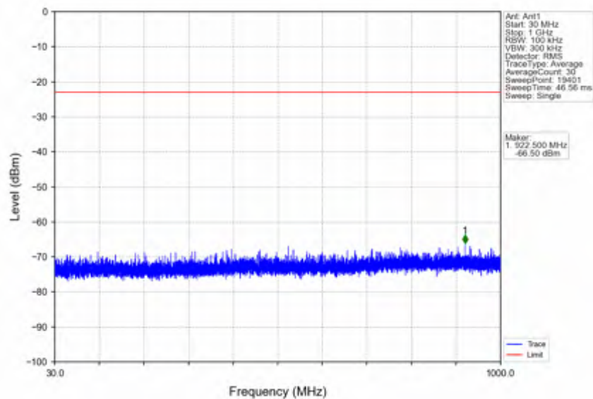
n41_30kHz_SISO_NTNV_15MHz_CP-OFDM QPSK_2682.48MHz_Inner_1RB_Right
