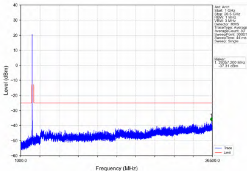
n41_30kHz_SISO_NTNV_30MHz_DFT-s-OFDM PI/2 BPSK_2511MHz_Outer_Full
