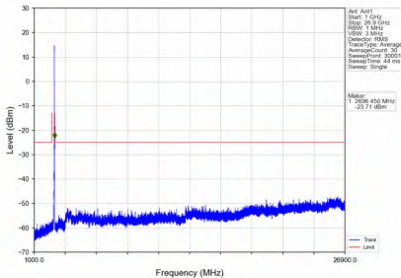
n41_30kHz_SISO_NTNV_20MHz_DFT-s-OFDM QPSK_2679.99MHz_Inner_1RB_Right
