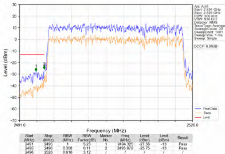
n41_30kHz_SISO_NTNV_30MHz_DFT-s-OFDM PI/2 BPSK_2511MHz_Outer_Full
