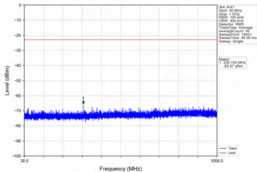
n41_30kHz_SISO_NTNV_30MHz_CP-OFDM QPSK_2511MHz_Outer_Full
