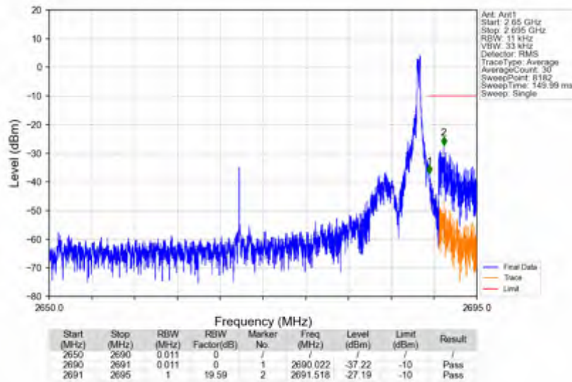
n41_30kHz_SISO_NTNV_40MHz_CP-OFDM QPSK_2670MHz_Edge_1RB_Right
