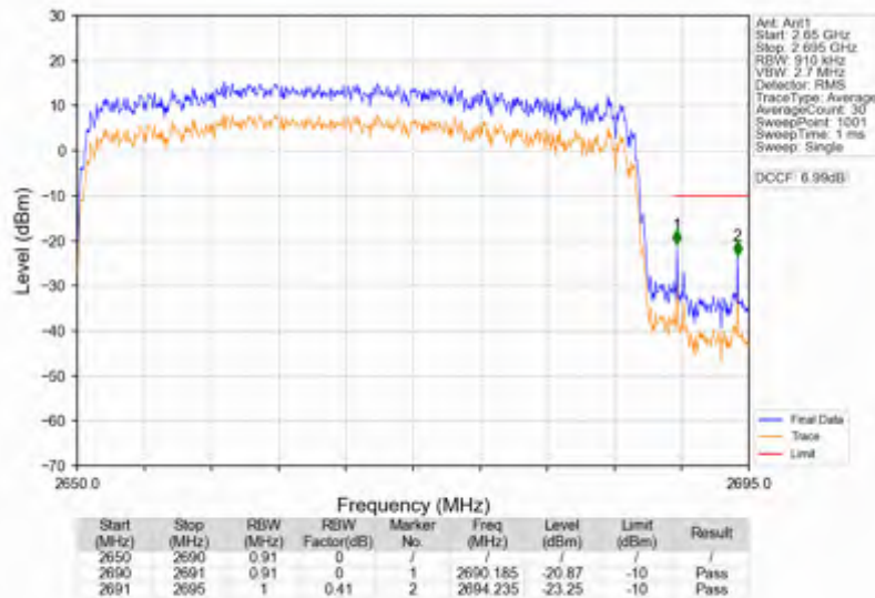
n41_30kHz_SISO_NTNV_40MHz_DFT-s-OFDM PI/2 BPSK_2670MHz_Outer_Full
