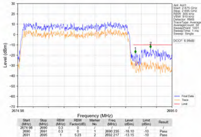
n41_30kHz_SISO_NTNV_15MHz_CP-OFDM_QPSK_2682.48MHz_Outer_Full
