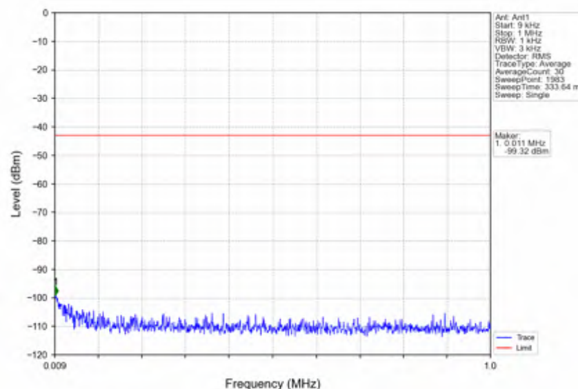
n41_30kHz_SISO_NTNV_30MHz_DFT-s-OFDM QPSK_2674.98MHz_Outer_Full
