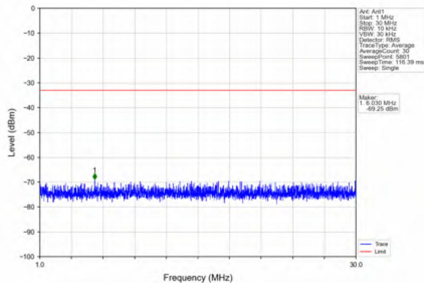
n41_30kHz_SISO_NTNV_40MHz_CP-OFDM QPSK_2516.01MHz_Edge_1RB_Left
