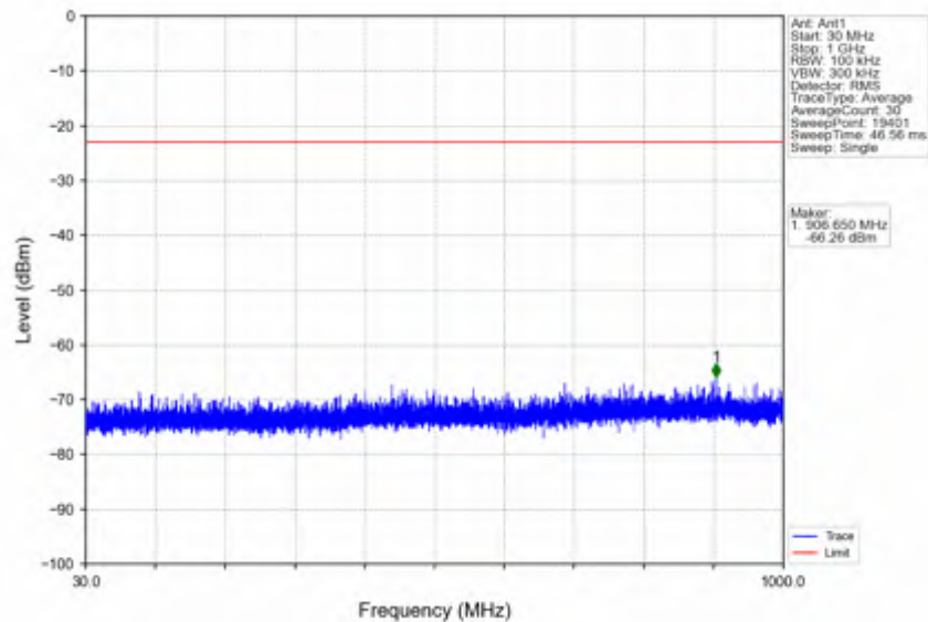
n41_30kHz_SISO_NTNV_40MHz_DFT-s-OFDM PI/2 BPSK_2670MHz_Outer_Full
