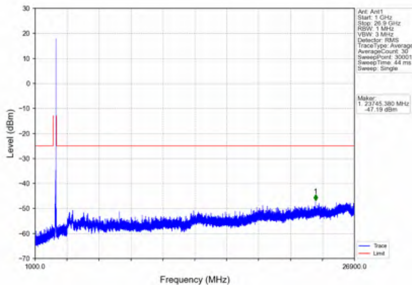
n41_30kHz_SISO_NTNV_40MHz_CP-OFDM QPSK_2670MHz_Outer_Full
