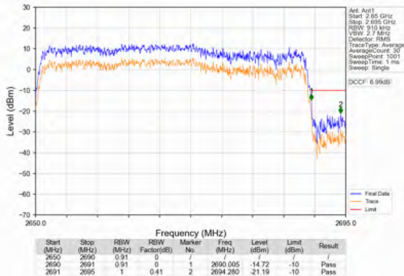
n41_30kHz_SISO_NTNV_40MHz_CP-OFDM QPSK_2670MHz_Outer_Full
