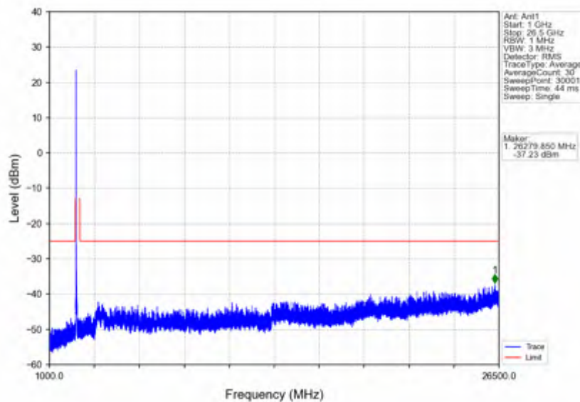
n41_30kHz_SISO_NTNV_30MHz_CP-OFDM QPSK_2511MHz_Outer_Full
