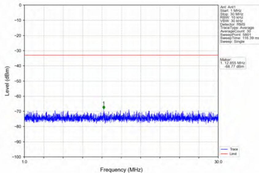
n41_30kHz_SISO_NTNV_20MHz_CP-OFDM QPSK_2679.99MHz_Edge_1RB_Right
