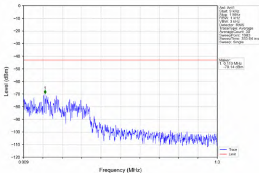
n41_30kHz_SISO_NTNV_40MHz_DFT-s-OFDM_PI/2_BPSK_2516.01MHz_Edge_1RB_Left
