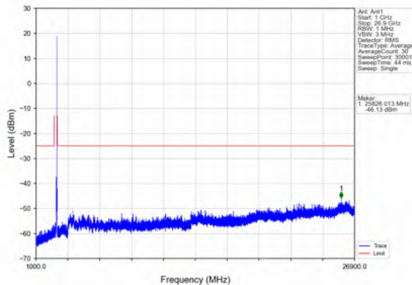
n41_30kHz_SISO_NTNV_30MHz_DFT-s-OFDM_QPSK_2674.98MHz_Edge_1RB_Right
