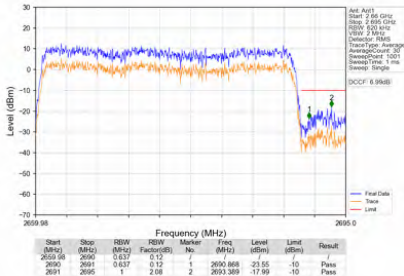
n41_30kHz_SISO_NTNV_30MHz_CP-OFDM QPSK_2674.98MHz_Outer_Full
