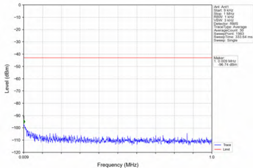
n41_30kHz_SISO_NTNV_30MHz_DFT-s-OFDM_PI/2_BPSK_2511MHz_Outer_Full
