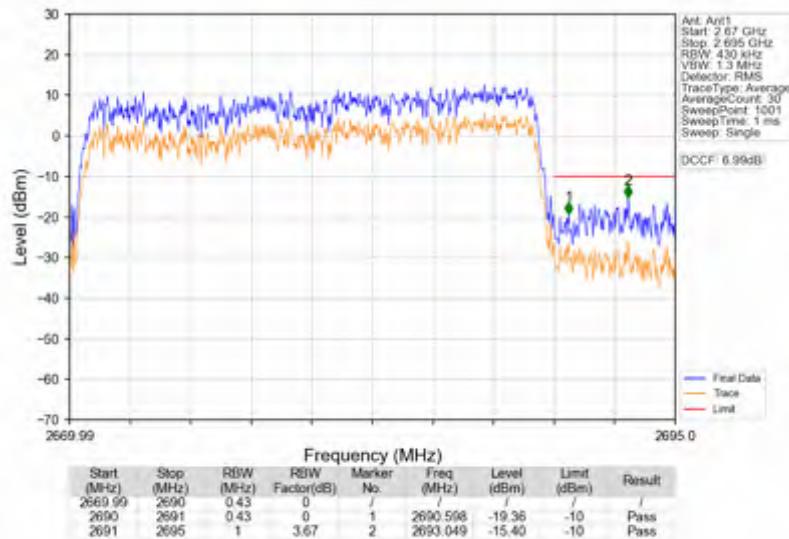
n41_30kHz_SISO_NTNV_20MHz_CP-OFDM QPSK_2679.99MHz_Outer_Full
