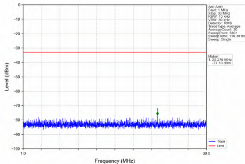
n41_30kHz_SISO_NTNV_20MHz_DFT-s-OFDM QPSK_2679.99MHz_Outer_Full
