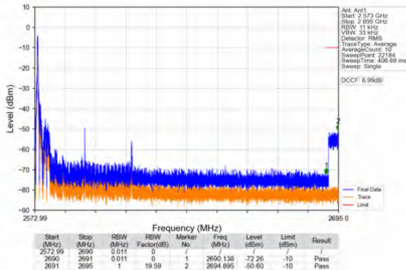
n41_30kHz_SISO_NTNV_40MHz_CP-OFDM QPSK_2592.99MHz_Edge_1RB_Left
