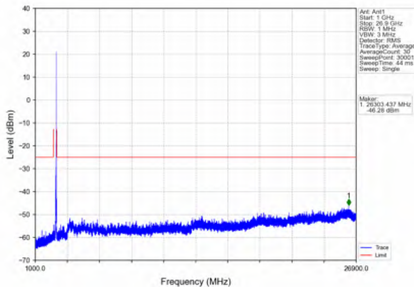
n41_30kHz_SISO_NTNV_40MHz_DFT-s-OFDM PI/2 BPSK_2670MHz_Outer_Full
