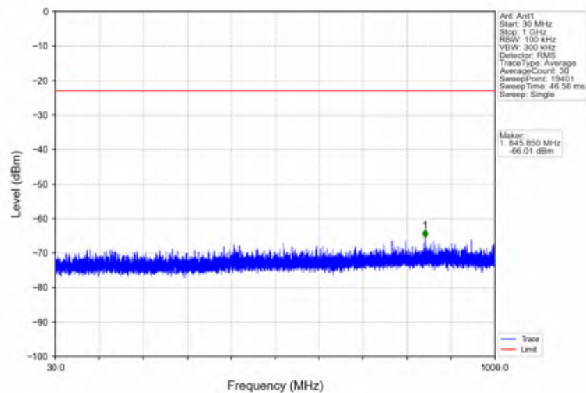
n41 30kHz SISO NTNV 15MHz CP-OFDM QPSK 2682.48MHz Outer Full
