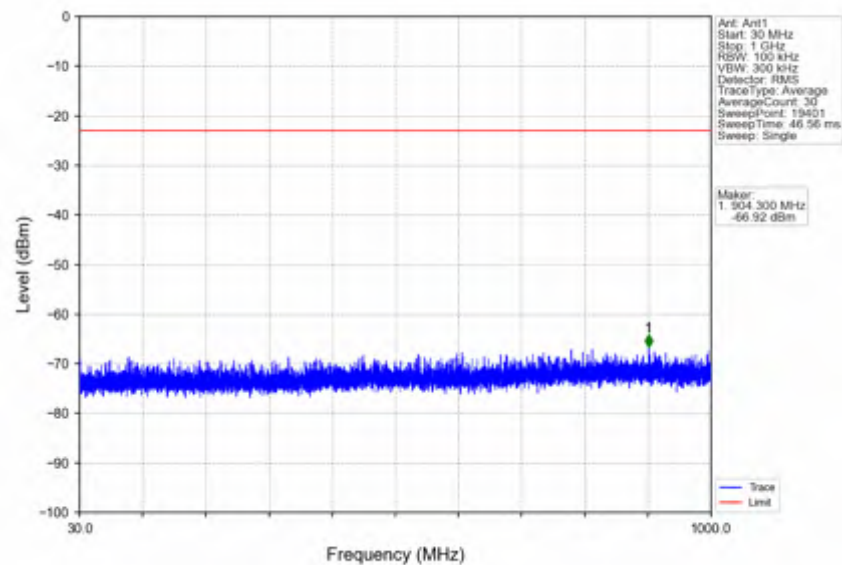
n41_30kHz_SISO_NTNV_40MHz_CP-OFDM QPSK_2516.01MHz_Outer_Full
