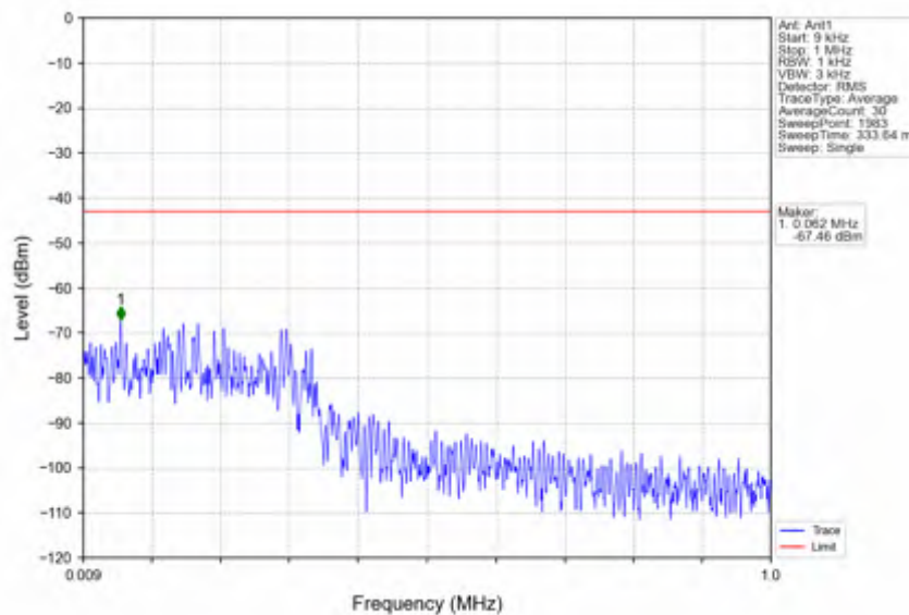
n41_30kHz_SISO_NTNV_20MHz_DFT-s-OFDM_QPSK_2592.99MHz_Edge_1RB_Left
