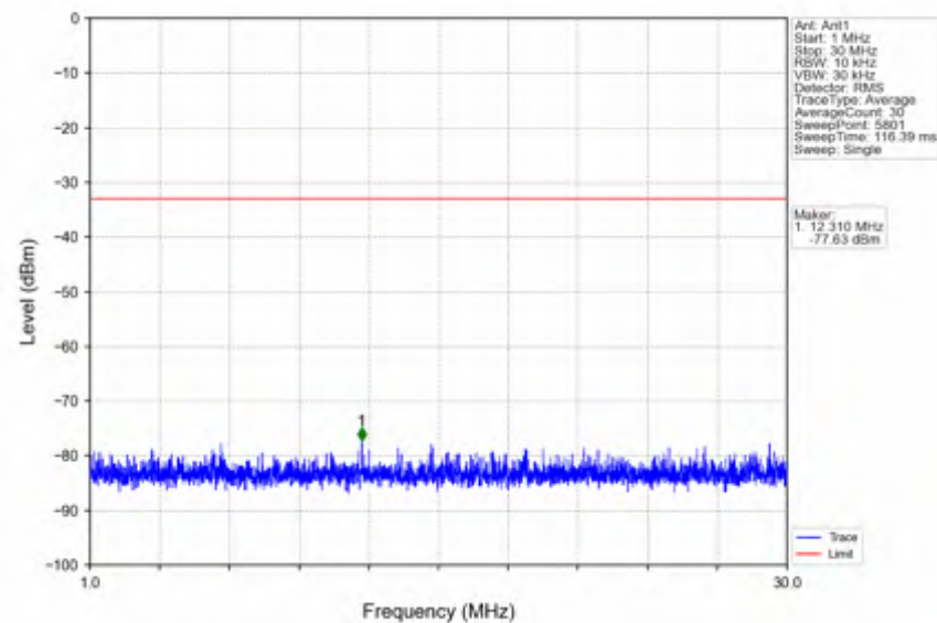
n41_30kHz_SISO_NTNV_40MHz_DFT-s-OFDM QPSK_2670MHz_Outer_Full
