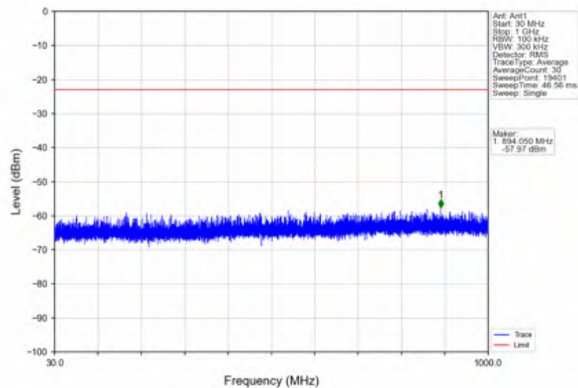
n41_30kHz_SISO_NTNV_15MHz_CP-OFDM QPSK_2682.48MHz_Edge_1RB_Right
