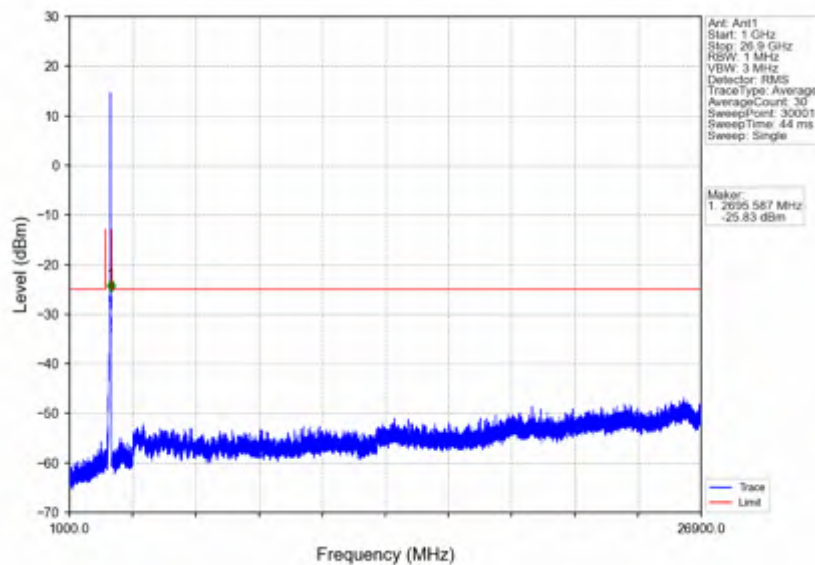
n41_30kHz_SISO_NTNV_30MHz_DFT-s-OFDM QPSK_2674.98MHz_Inner_1RB_Right
