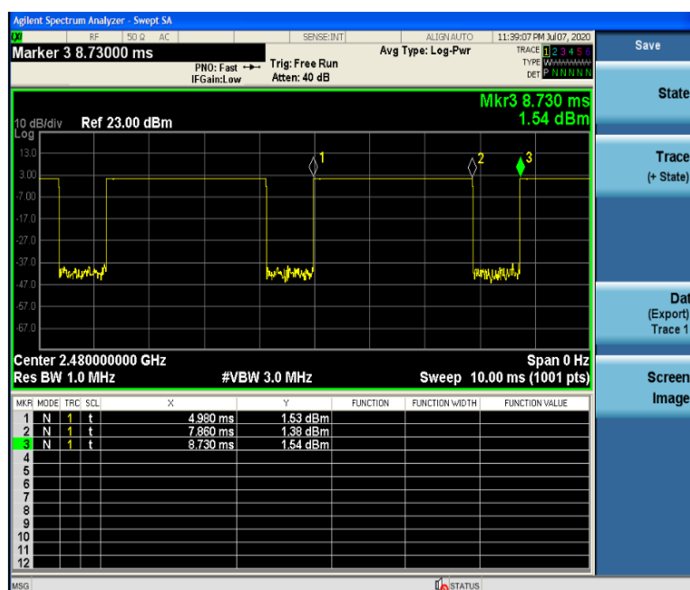
Time-domain plot for Bluetooth transmission signal
