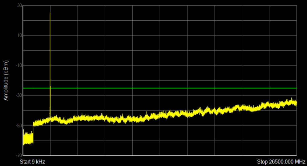
Band41 QAM16 BW=20MHz Channel=41090 RB Size=1 Position=#0
