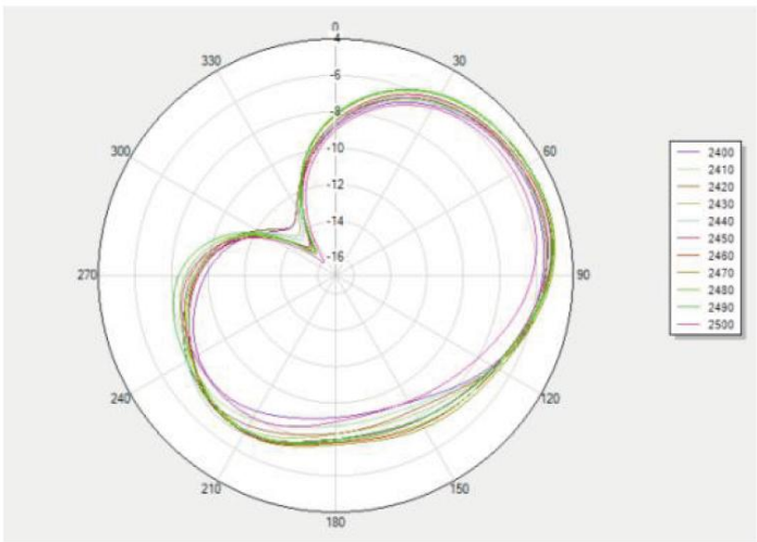
Theta 90 2D
