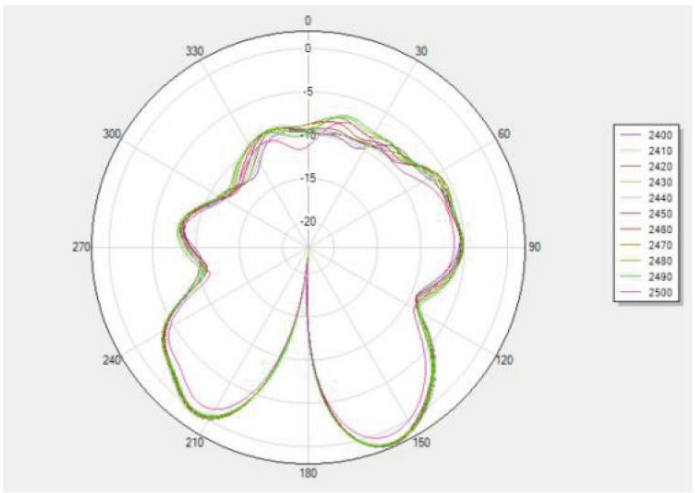
Theta 90 2D
