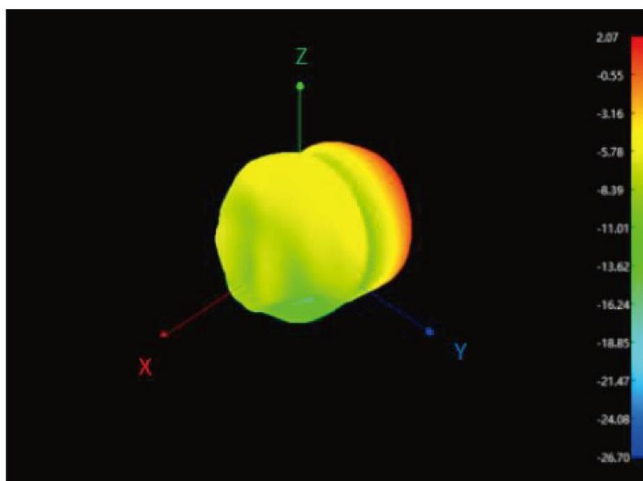
2440MHz 3D
