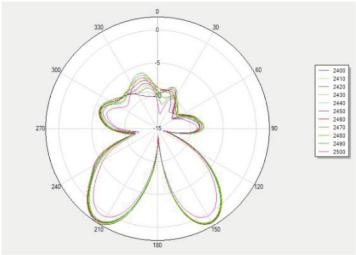
Phi 90 2D
