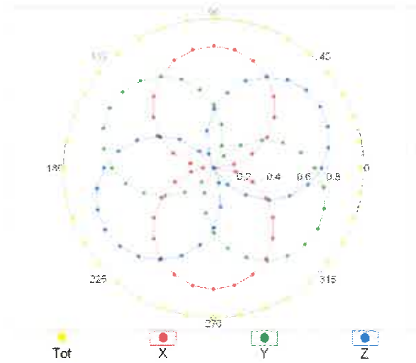
f=600 MHz,TEM
