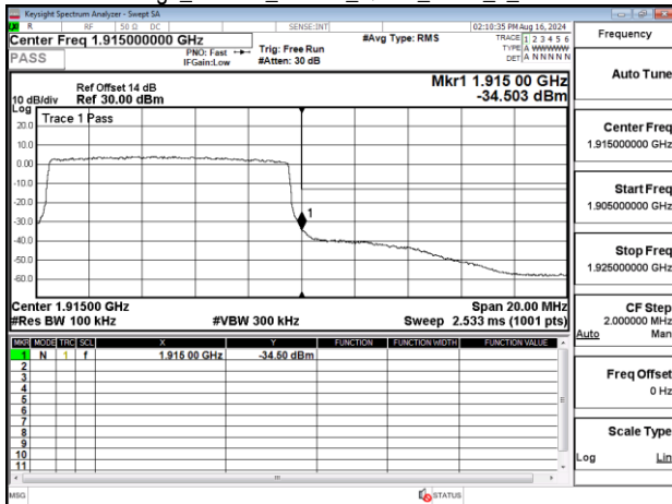
Band Edge_Band25_10MHz_QPSK_RB50_0_CH26640
