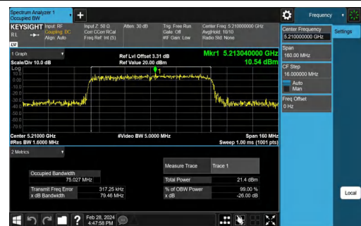
11AC80MIMO-Ant2-5210
