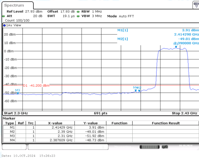
11AX20MIMO-Ant1-2412-PASS
