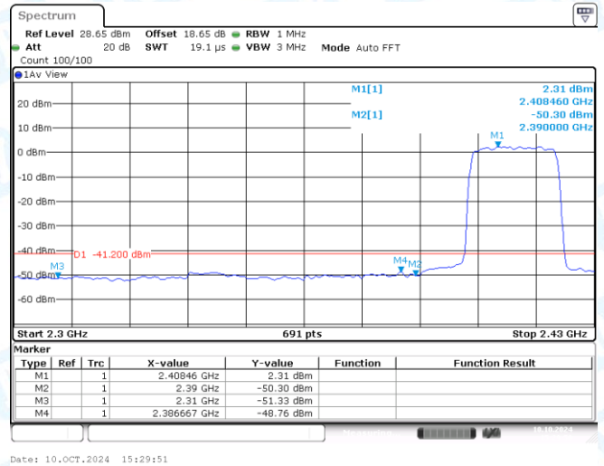
11AX20MIMO-Ant2-2412-PASS
