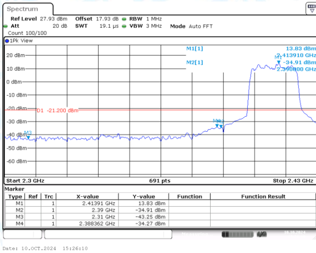
11AX20MIMO-Ant1-2412-PASS
