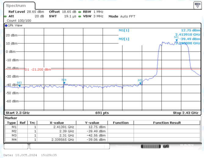
11AX20MIMO-Ant2-2412-PASS
