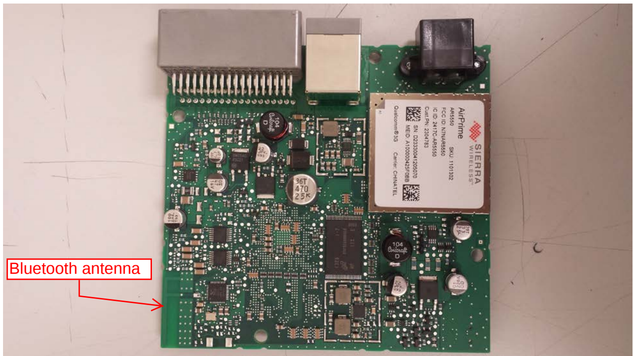
PCBA Top View
