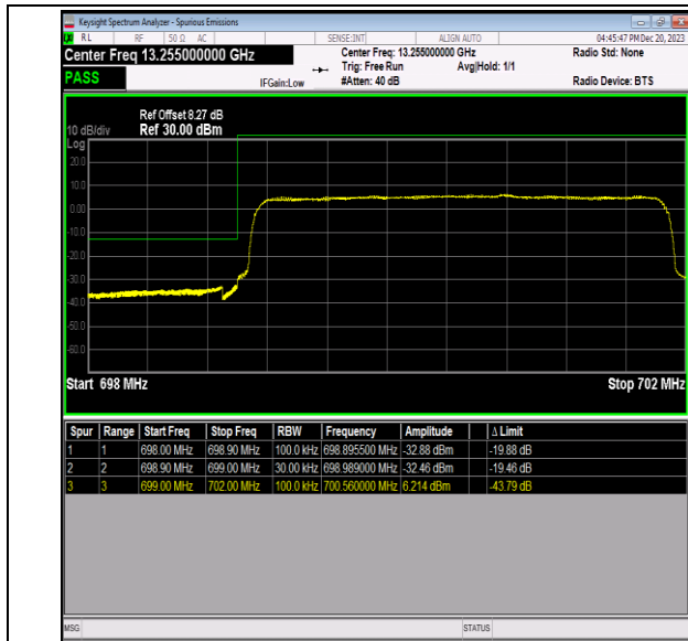
Band12_3MHz_QPSK_23025_15RB#0
