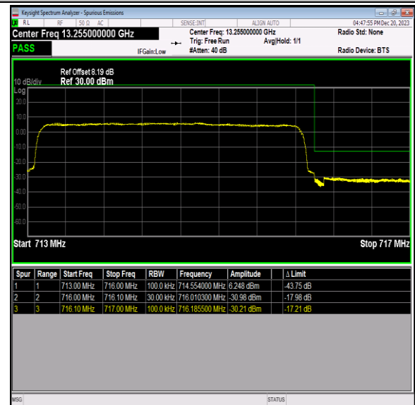
Band12_3MHz_QPSK_23165_15RB#0
