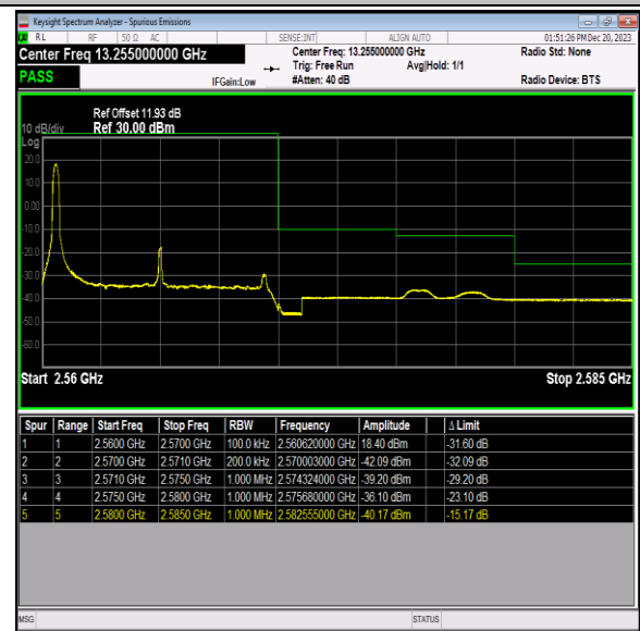
Band7_10MHz_16QAM_21400_1RB#0
