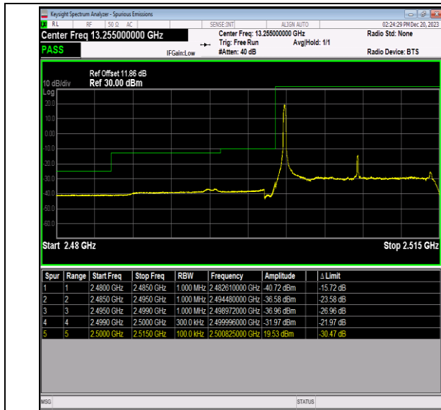
Band7_15MHz_QPSK_20825_1RB#0
