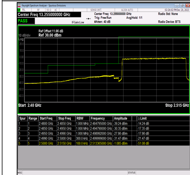
Band7_15MHz_QPSK_20825_75RB#0
