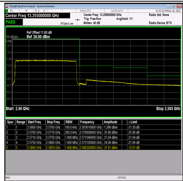
Band7_10MHz_64QAM_21400_50RB#0
