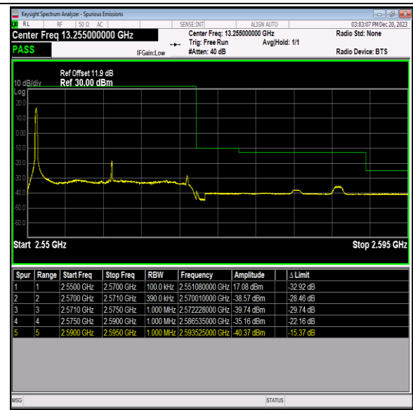
Band7_20MHz_64QAM_21350_1RB#0
