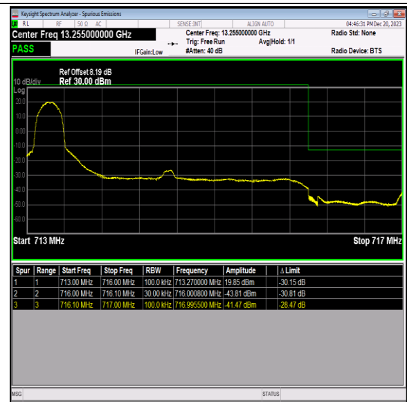
Band12_3MHz_QPSK_23165_1RB#0
