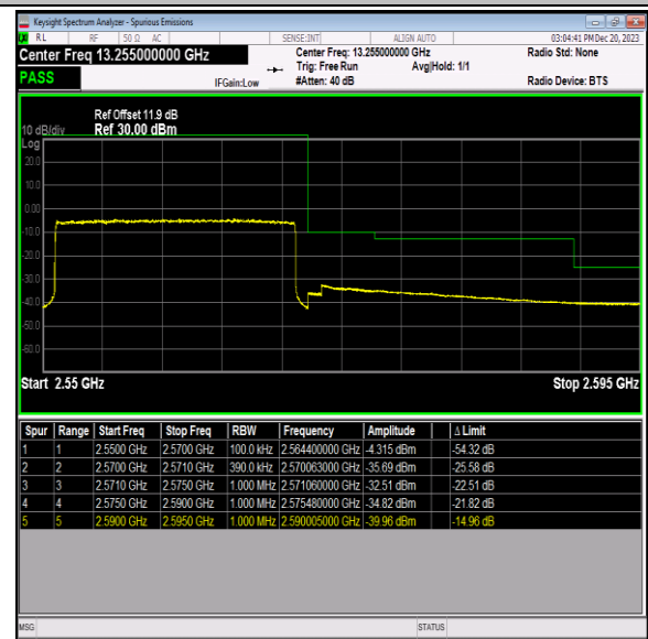
Band7_20MHz_64QAM_21350_100RB#0
