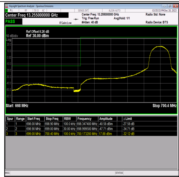
Band12_1.4MHz_64QAM_23017_1RB#5
