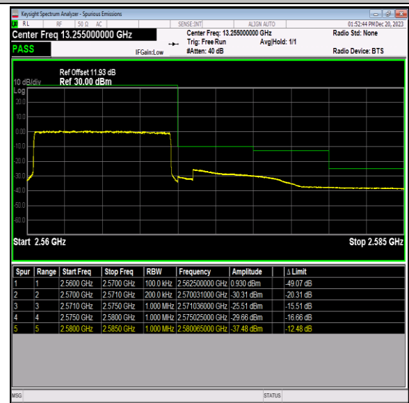
Band7_10MHz_QPSK_21400_50RB#0
