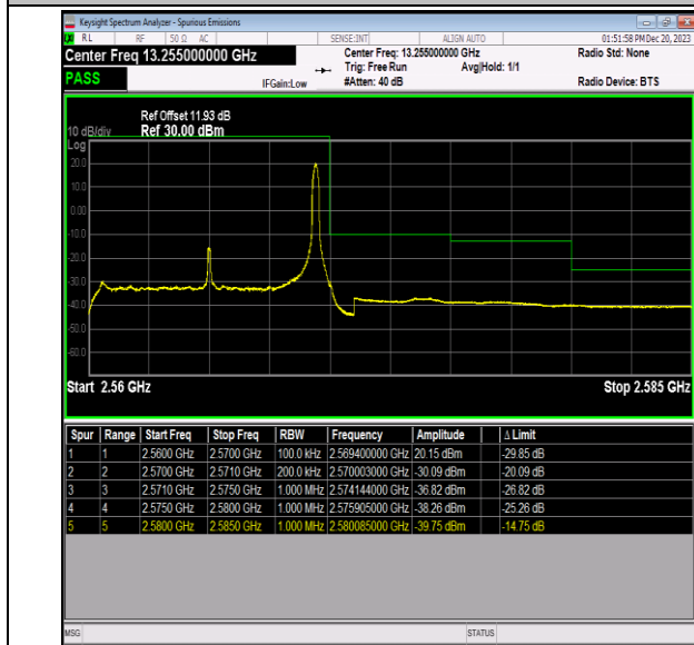
Band7_10MHz_QPSK_21400_1RB#49
