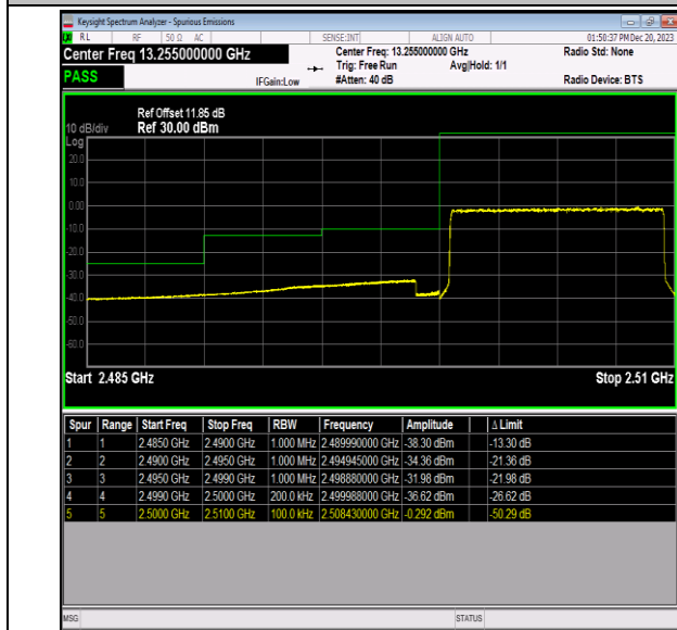
Band7_10MHz_16QAM_20800_50RB#0
