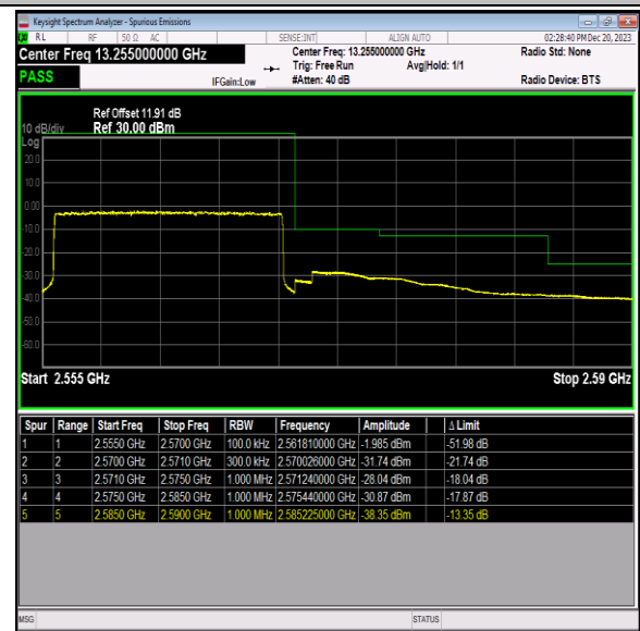
Band7_15MHz_16QAM_21375_75RB#0
