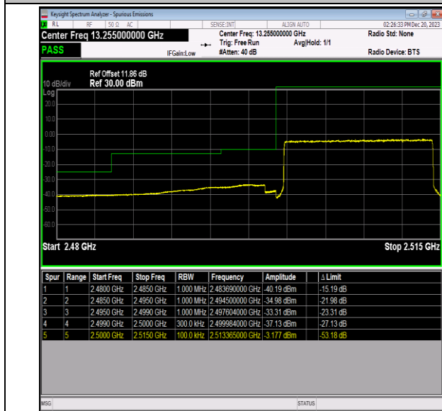
Band7_15MHz_64QAM_20825_75RB#0
