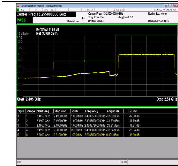
Band7_10MHz_QPSK_20800_50RB#0
