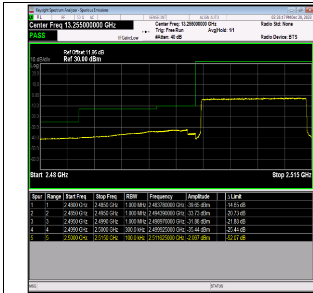
Band7_15MHz_16QAM_20825_75RB#0
