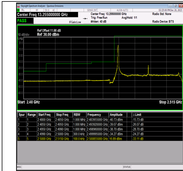
Band7_15MHz_64QAM_20825_1RB#0
