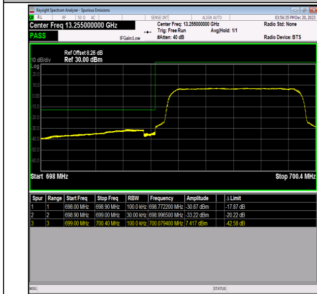
Band12_1.4MHz_64QAM_23017_6RB#0
