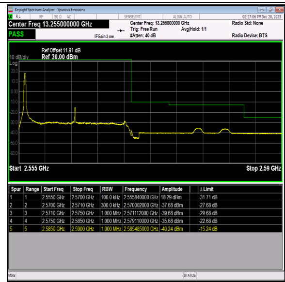
Band7_15MHz_16QAM_21375_1RB#0
