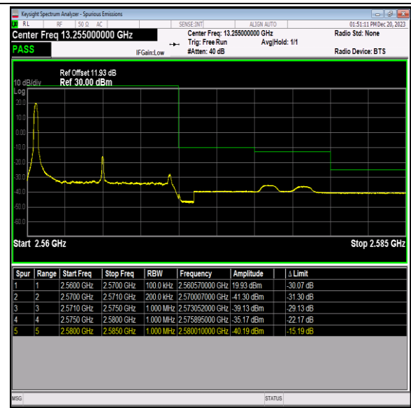
Band7_10MHz_QPSK_21400_1RB#0
