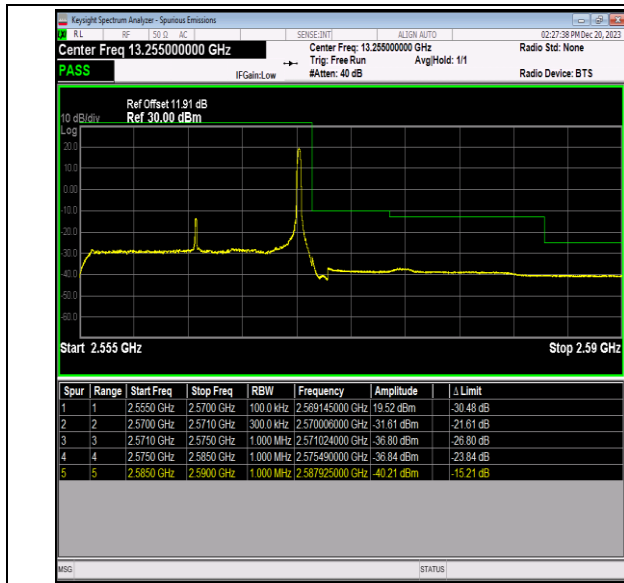
Band7_15MHz_QPSK_21375_1RB#74
