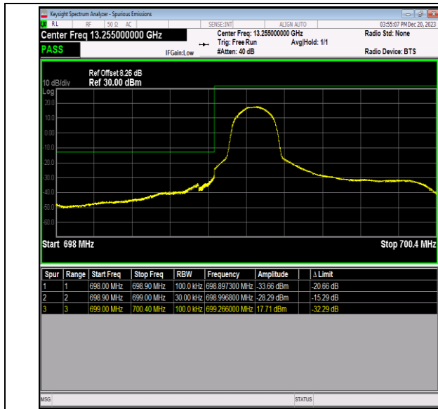
Band12_1.4MHz_64QAM_23017_1RB#0
