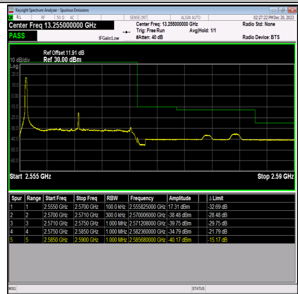
Band7_15MHz_64QAM_21375_1RB#0
