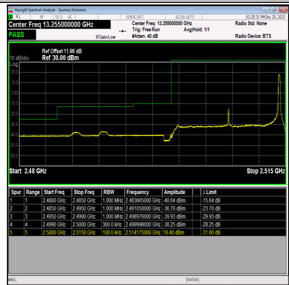
Band7_15MHz_16QAM_20825_1RB#74
