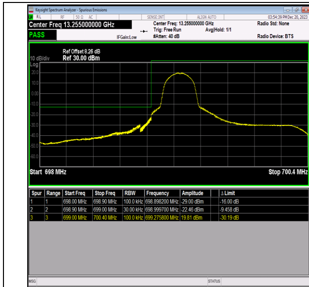
Band12_1.4MHz_QPSK_23017_1RB#0
