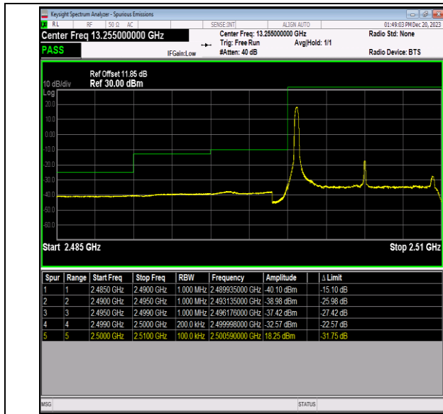
Band7_10MHz_16QAM_20800_1RB#0
