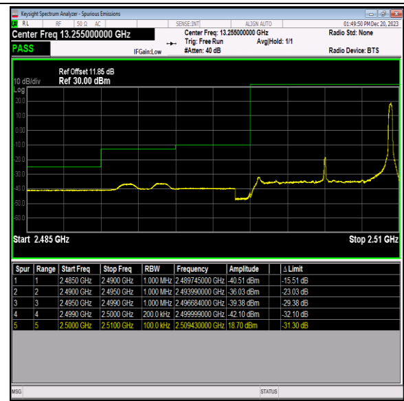
Band7_10MHz_16QAM_20800_1RB#49
