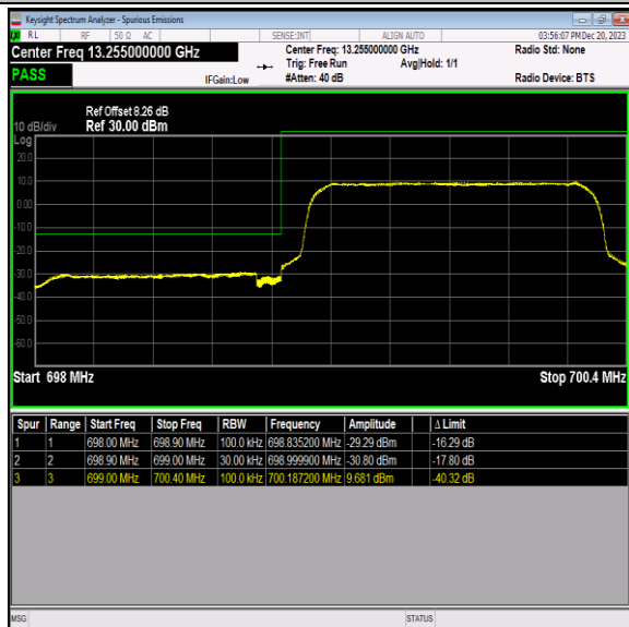
Band12_1.4MHz_QPSK_23017_6RB#0
