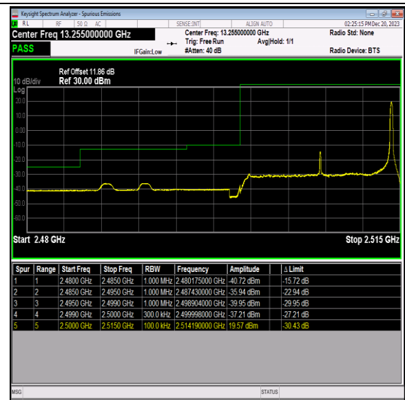
Band7_15MHz_QPSK_20825_1RB#74
