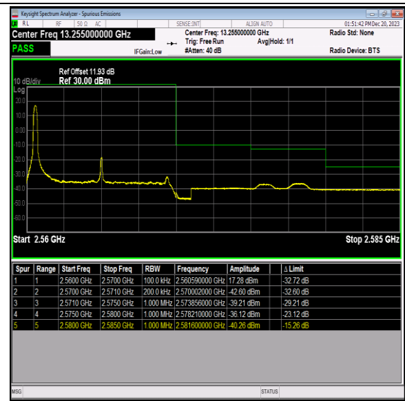
Band7_10MHz_64QAM_21400_1RB#0
