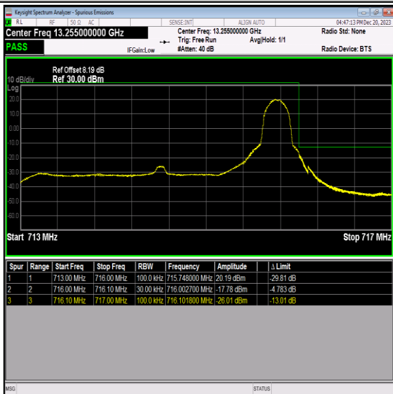
Band12_3MHz_QPSK_23165_1RB#14
