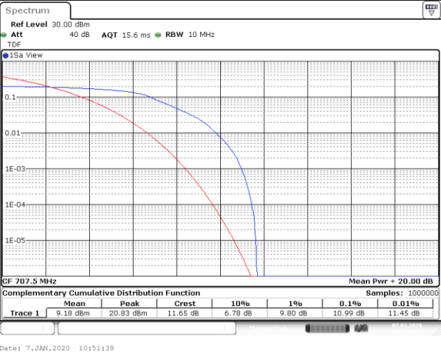
Band12_5MHz_QPSK_23095_6_0_Low_8.29_<=13_PASS_
