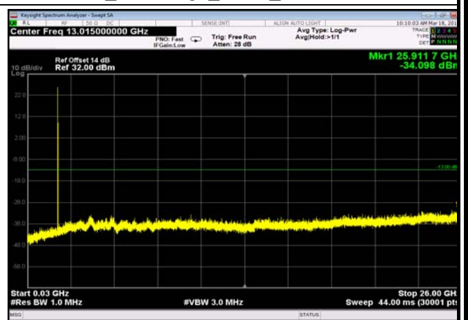
FDD02_MidRange_10MHz_30MHz~26GHz
