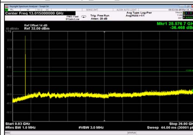
FDD02_MidRange_1.4MHz_30MHz~26GHz
