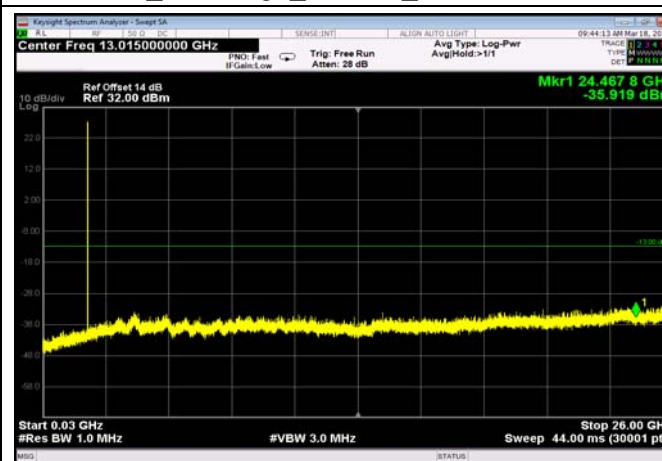
FDD02_MidRange_1.4MHz_30MHz~26GHz
