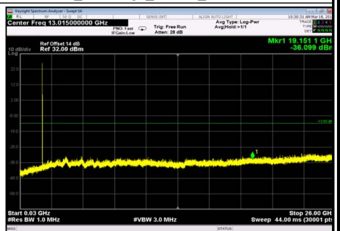
FDD02_MidRange_10MHz_30MHz~26GHz
