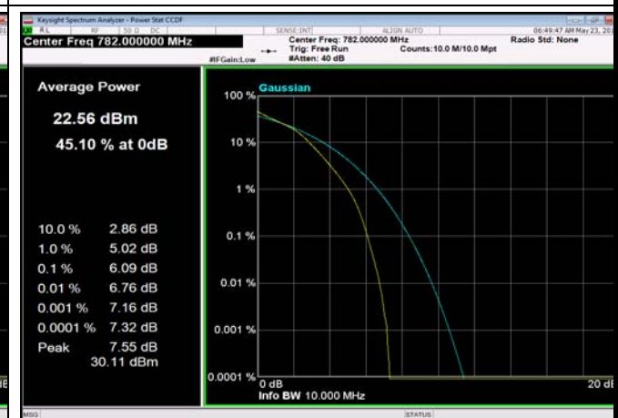
FDD13_10MHz_782MHz_fullRB_Q16
