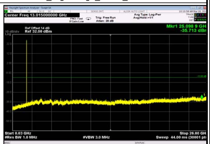
FDD02_HighRange_5MHz_30MHz~26GHz
