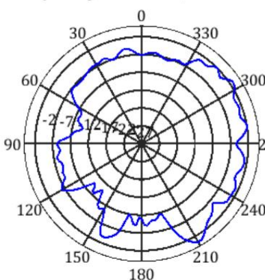
2400MHz_3D
