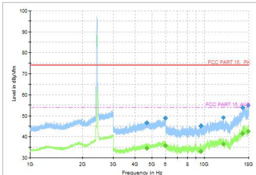
Fig.42 Radiated Spurious Emission (802.11n-HT40, CH3, 1GHz-18GHz)
