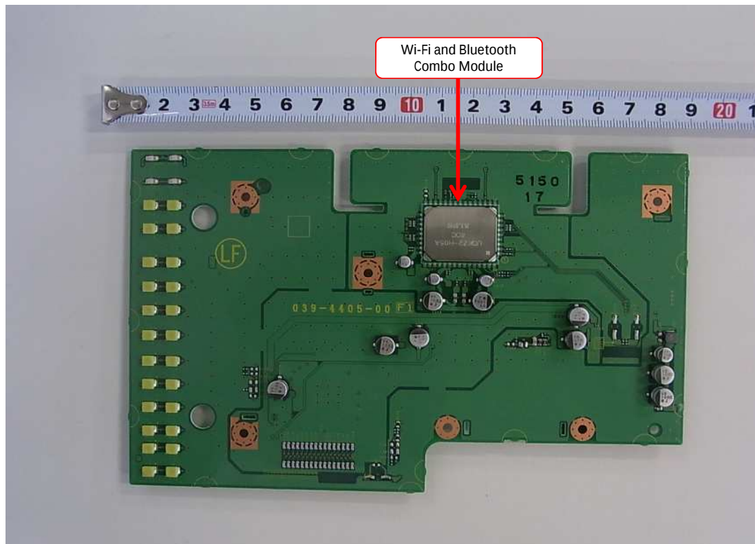
LCD PCB ASSY Component - F2 View
