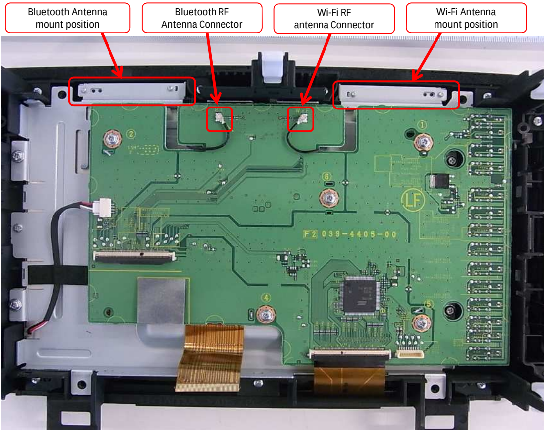
LCD PCB ASSY Component - F2 View
