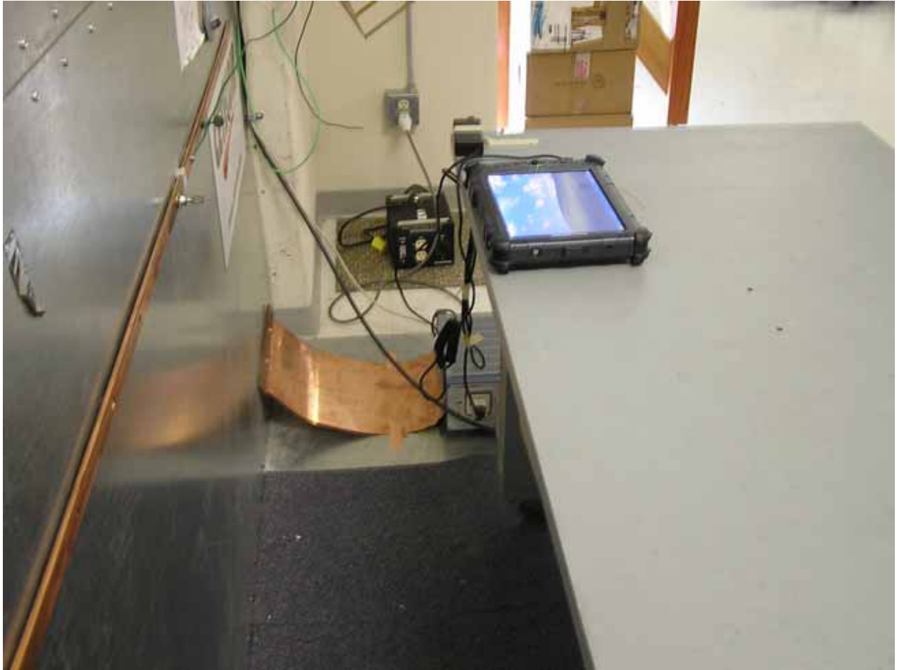
Conducted emissions
