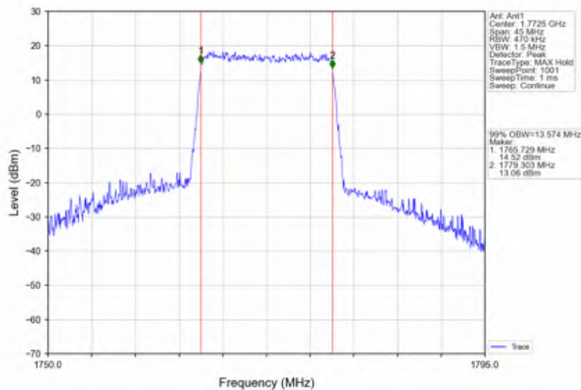
Band66_15MHz_16QAM_HCH_1772.5MHz_RB_75_0_NTNV
