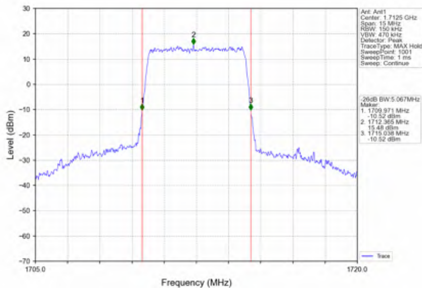
Band66_5MHz_256QAM_LCH_1712.5MHz_RB_25_0_NTNV
