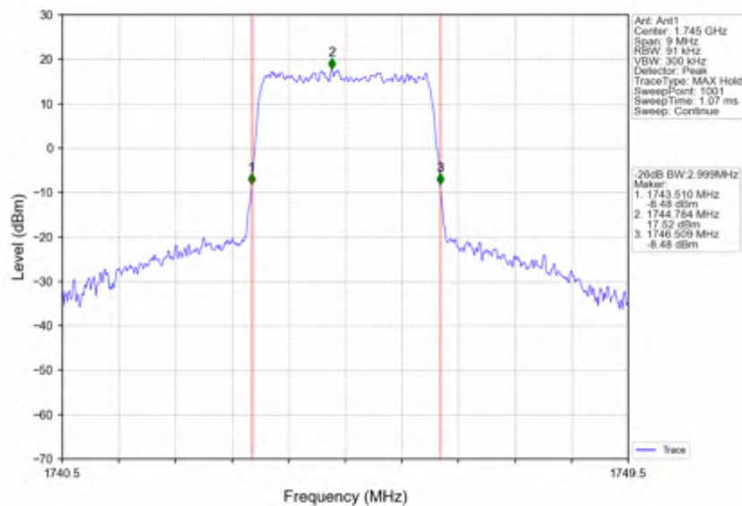
Band66_3MHz_64QAM_MCH_1745MHz_RB_15_0_NTNV
