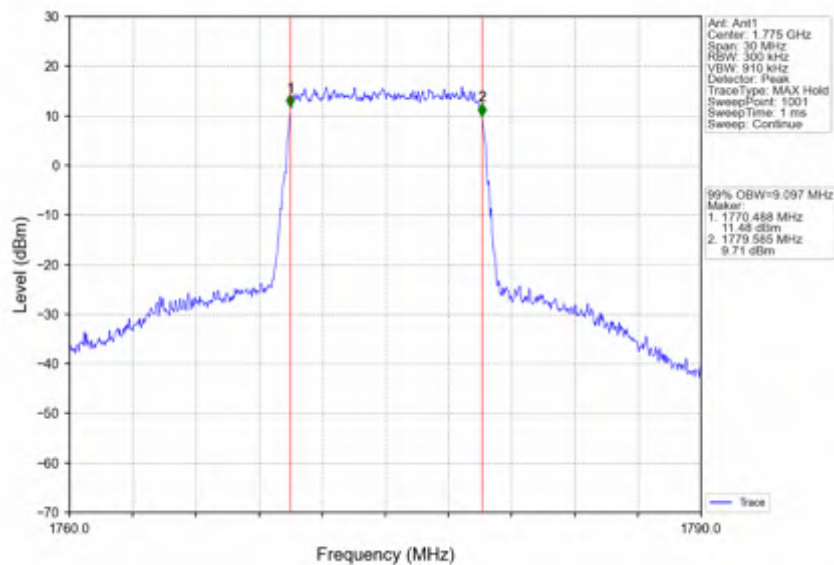
Band66 10MHz 256QAM HCH 1775MHz RB 50 0 NTNV
