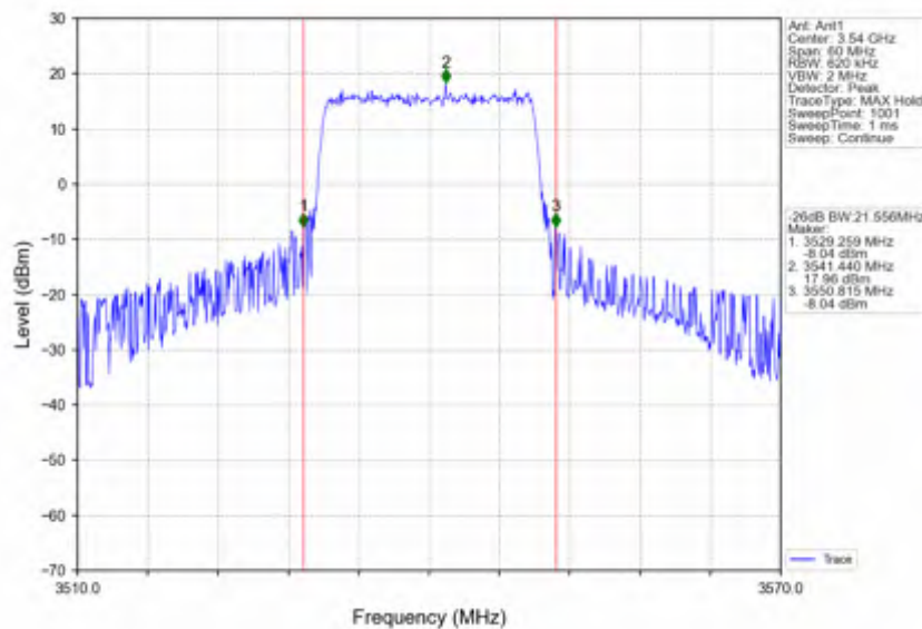
Band42a_20MHz_256QAM_HCH_3540MHz_RB_100_0_NTNV
