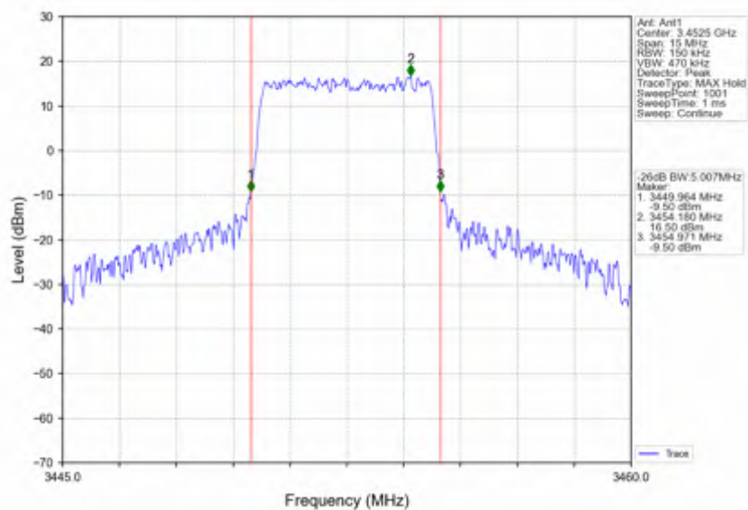
Band42a 5MHz 256QAM LCH 3452.5MHz RB 25 0 NTNV
