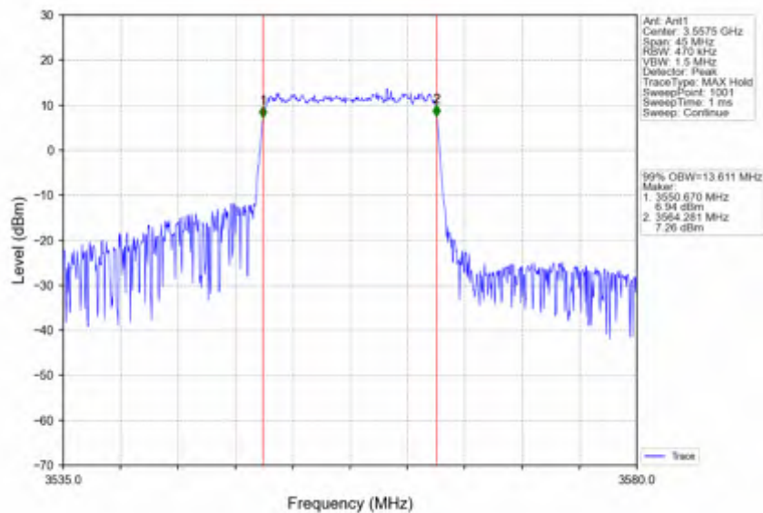
Band42c_15MHz_16QAM_LCH_3557.5MHz_RB_75_0_NTNV
