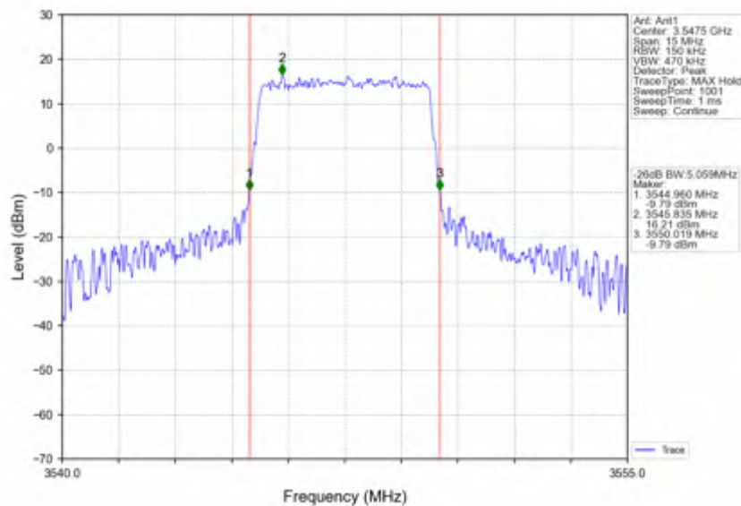
Band42a_5MHz_256QAM_HCH_3547.5MHz_RB_25_0_NTNV
