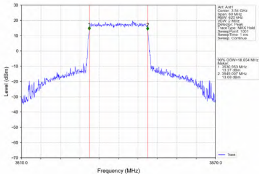
Band42a_20MHz_16QAM_HCH_3540MHz_RB_100_0_NTNV
