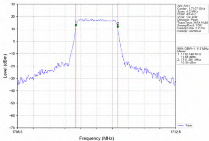
Band66_1.4MHz_16QAM_LCH_1710.7MHz_RB_6_0_NTNV
