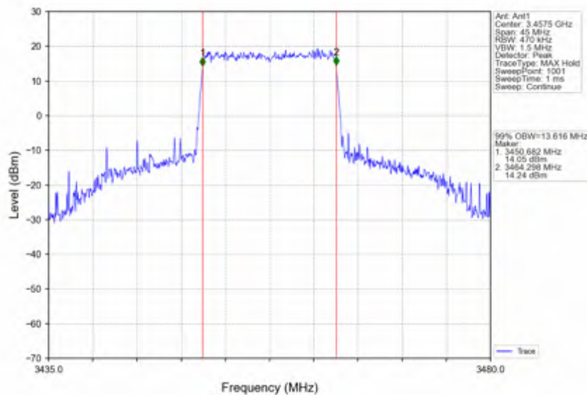
Band42a_15MHz_16QAM_LCH_3457.5MHz_RB_75_0_NTNV
