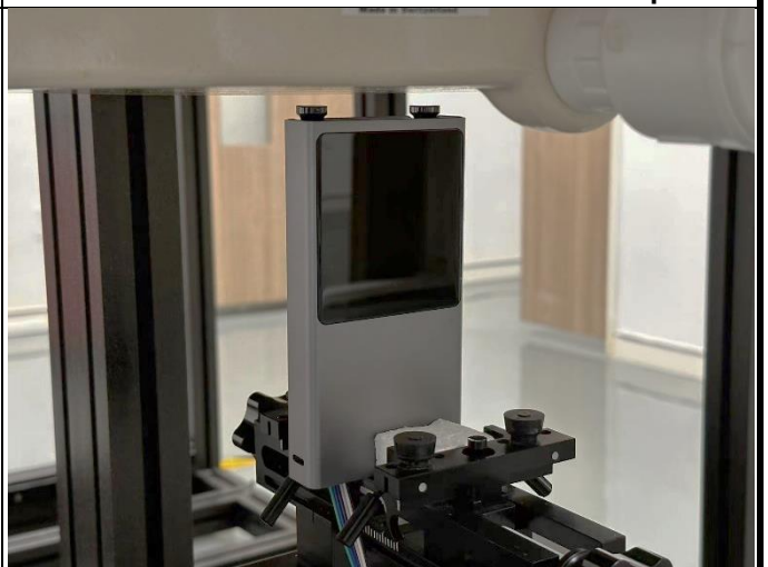
Top Side of EUT + Probe with 10mm Gap
