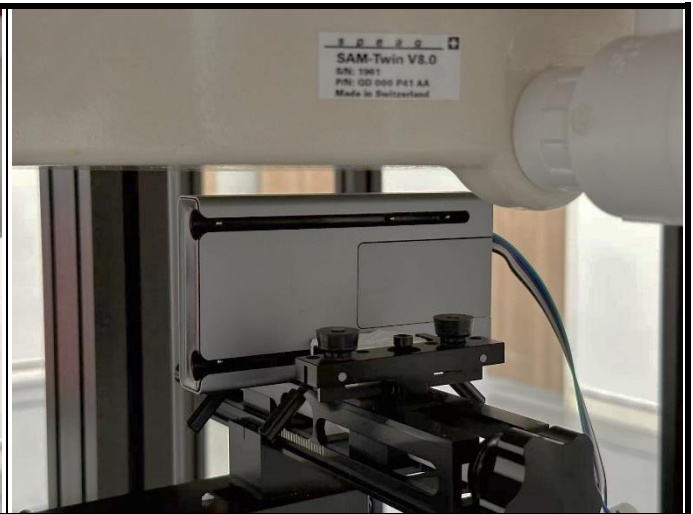
Left Side of EUT with 10mm Gap
