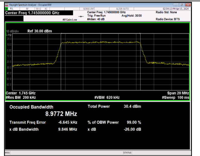
Band66-10MHz-16QAM-132322-50RB#0-PASS
