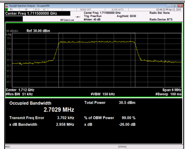
Band66-3MHz-QPSK-131987-15RB#0-PASS
