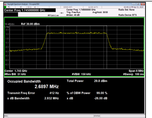
Band66-3MHz-16QAM-132322-15RB#0-PASS
