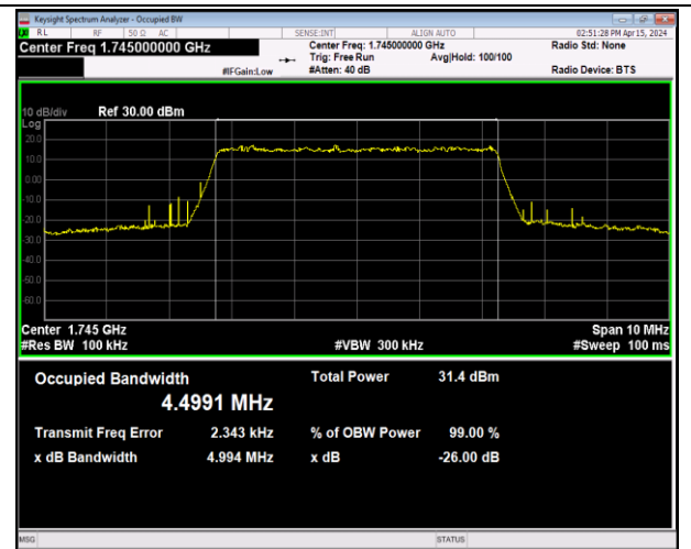
Band66-5MHz-QPSK-132322-25RB#0-PASS
