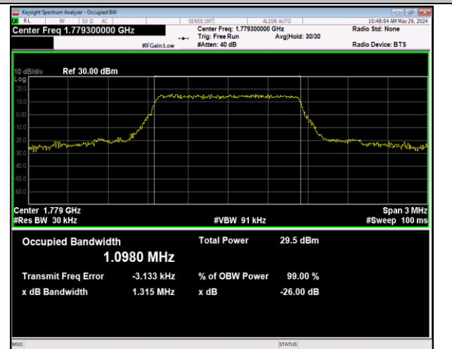
Band66-1.4MHz-16QAM-132665-6RB#0-PASS
