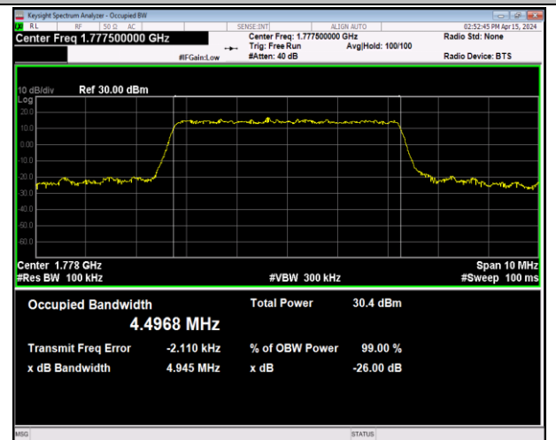
Band66-5MHz-16QAM-132647-25RB#0-PASS
