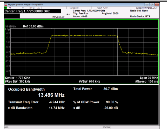
Band66-15MHz-16QAM-132597-75RB#0-PASS
