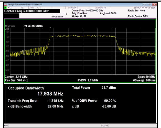
42(3450-3550)-20MHz-64QAM-42190-100RB#0-PASS
