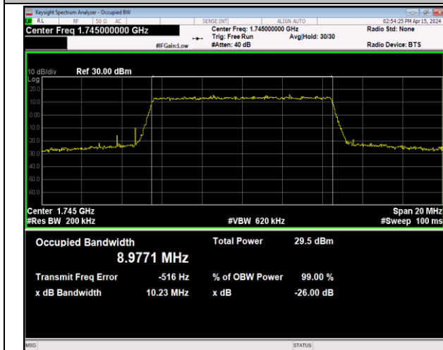
Band66-10MHz-64QAM-132322-50RB#0-PASS
