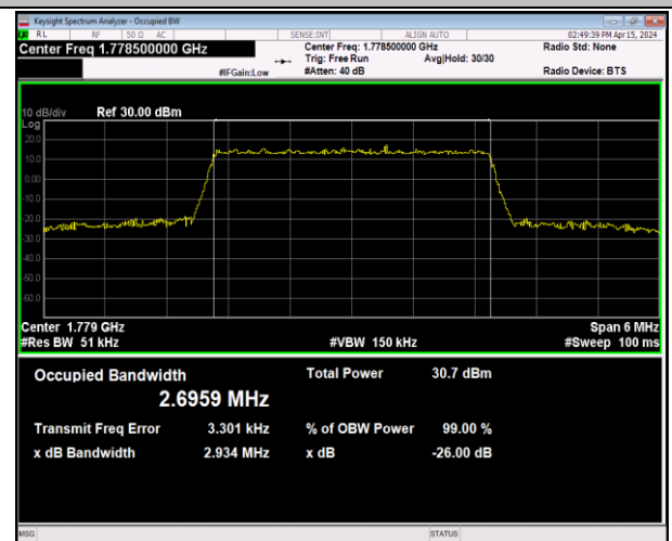
Band66-3MHz-QPSK-132657-15RB#0-PASS
