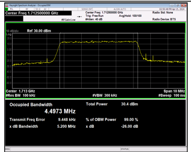
Band66-5MHz-16QAM-131997-25RB#0-PASS
