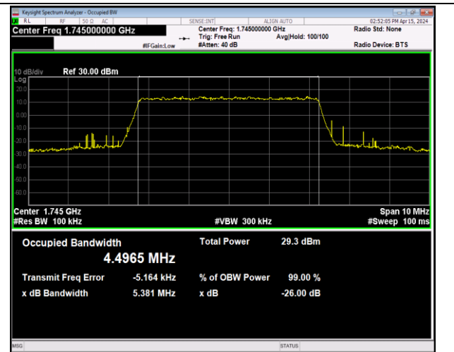
Band66-5MHz-64QAM-132322-25RB#0-PASS
