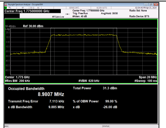
Band66-10MHz-QPSK-132622-50RB#0-PASS
