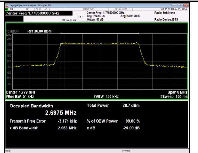
Band66-3MHz-64QAM-132657-15RB#0-PASS
