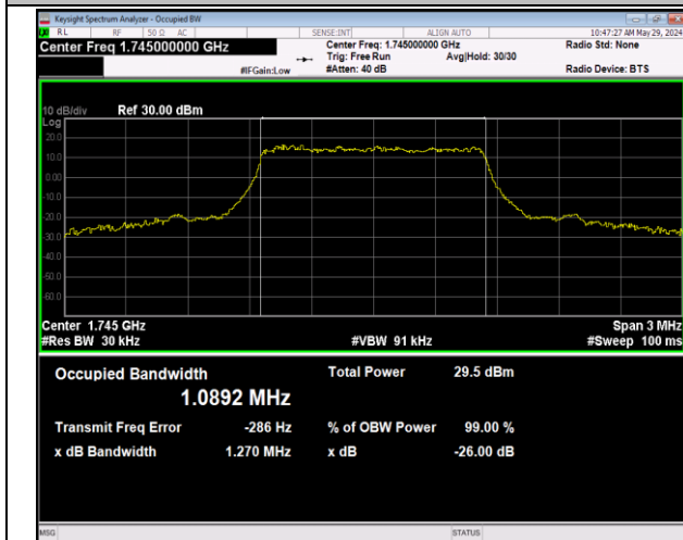
Band66-1.4MHz-16QAM-132322-6RB#0-PASS
