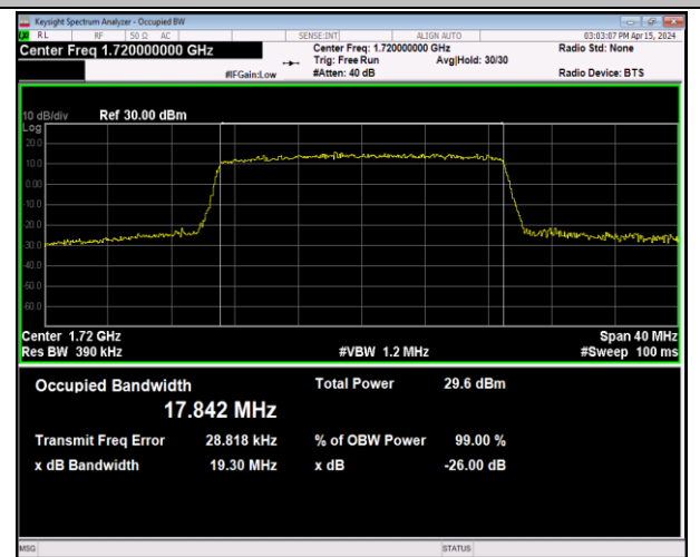
Band66-20MHz-64QAM-132072-100RB#0-PASS
