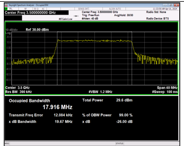
42(3450-3550)-20MHz-16QAM-42590-100RB#0-PASS
