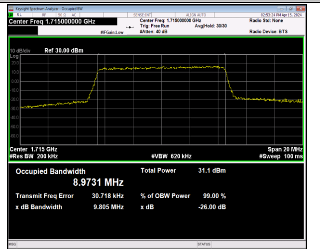
Band66-10MHz-QPSK-132022-50RB#0-PASS
