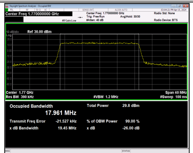
Band66-20MHz-64QAM-132572-100RB#0-PASS
