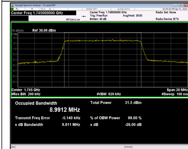
Band66-10MHz-QPSK-132322-50RB#0-PASS
