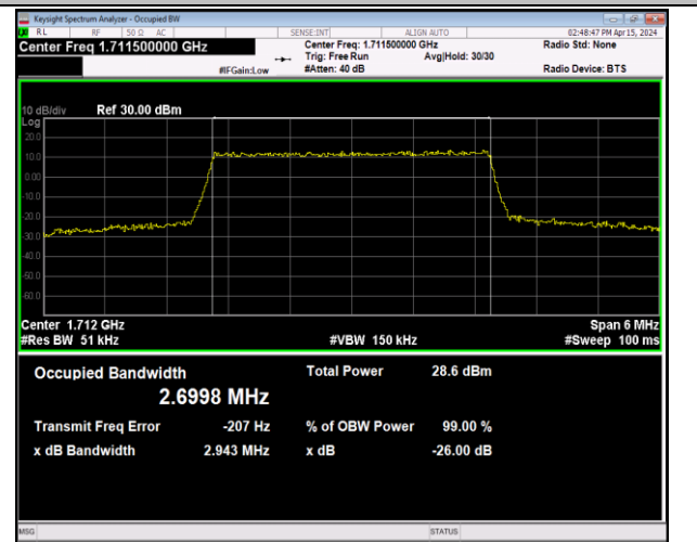
Band66-3MHz-64QAM-131987-15RB#0-PASS
