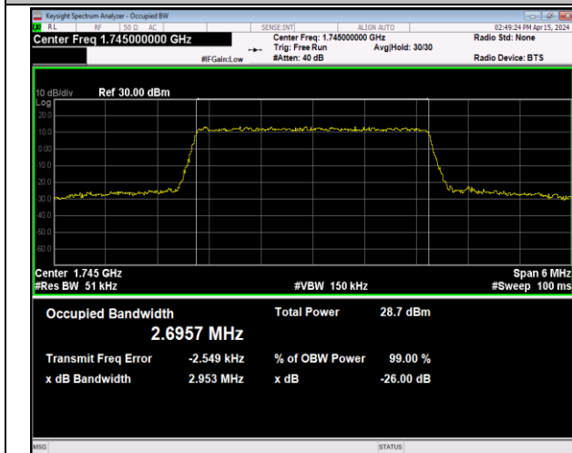
Band66-3MHz-64QAM-132322-15RB#0-PASS
