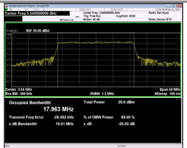
42(3450-3550)-20MHz-64QAM-42990-100RB#0-PASS
