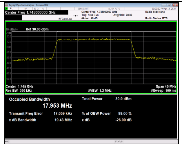
Band66-20MHz-16QAM-132322-100RB#0-PASS
