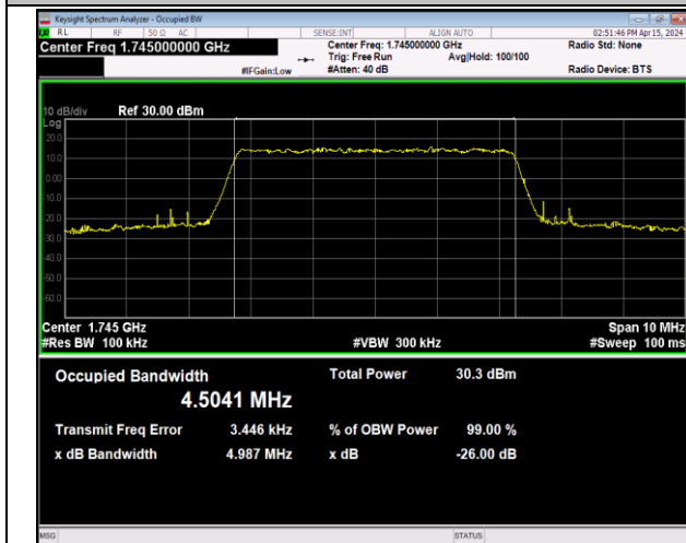
Band66-5MHz-16QAM-132322-25RB#0-PASS
