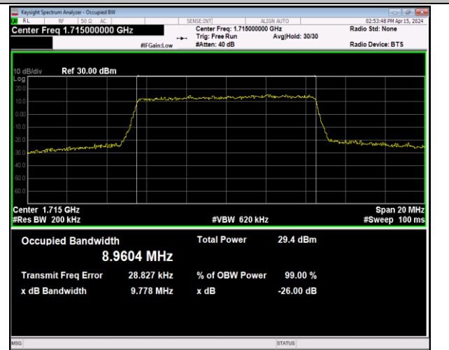
Band66-10MHz-64QAM-132022-50RB#0-PASS
