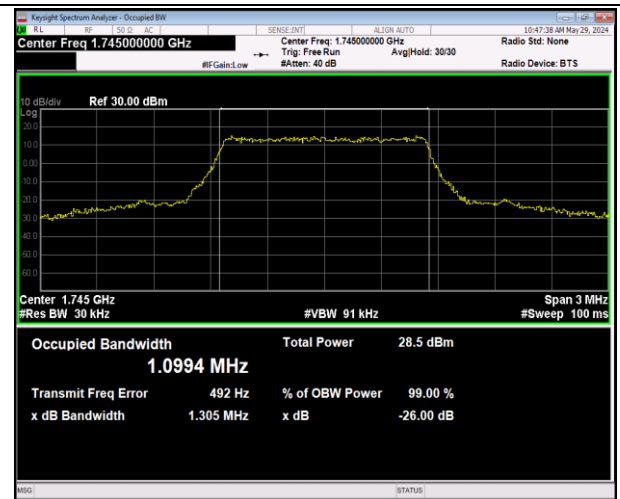
Band66-1.4MHz-64QAM-132322-6RB#0-PASS
