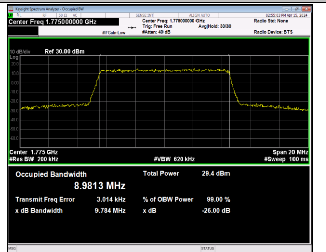
Band66-10MHz-64QAM-132622-50RB#0-PASS
