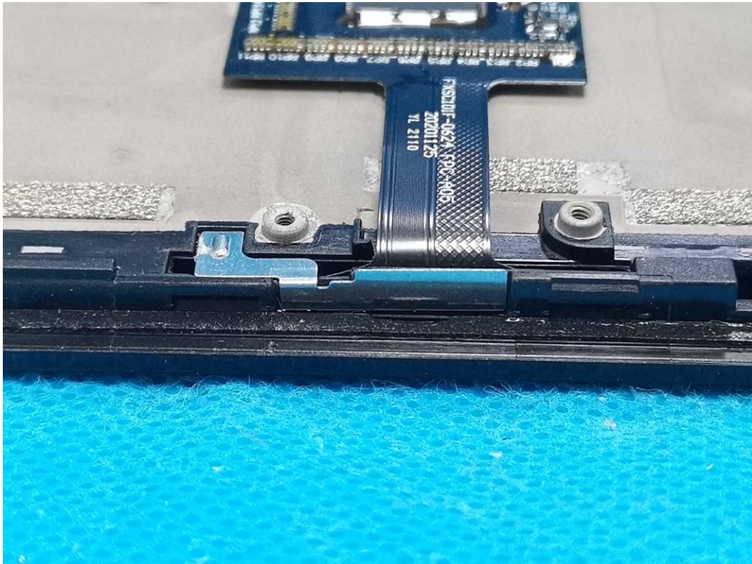
2.4G&5G Wi-Fi Antenna Chain1
