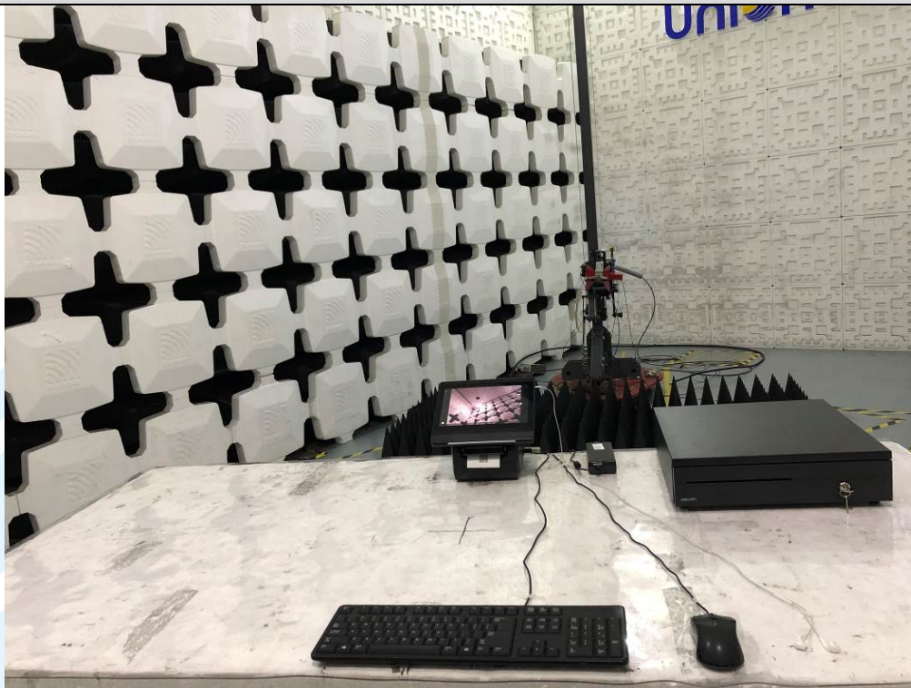
Radiated emission Test Setup-2 (Above 1 GHz) – Test Mode 1
